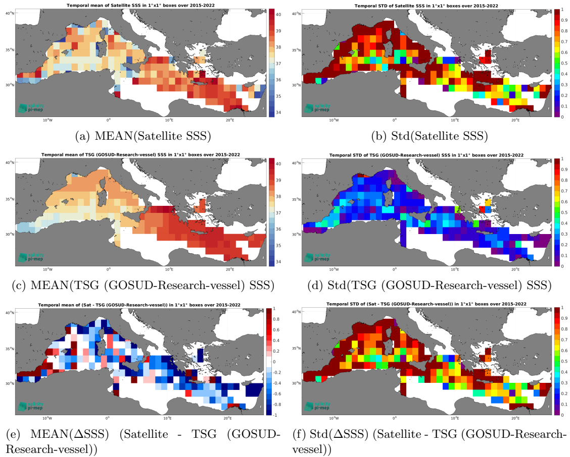
Figure 7: Temporal mean (left) and Std (right) of SSS from SMAP SSS L2 v5.0 (JPL) (top), TSG (GOSUD-Research-vessel) (middle), and of \Delta SSS (Satellite - TSG (GOSUD-Research-vessel)). Only match-up pairs are used to generate these maps.
