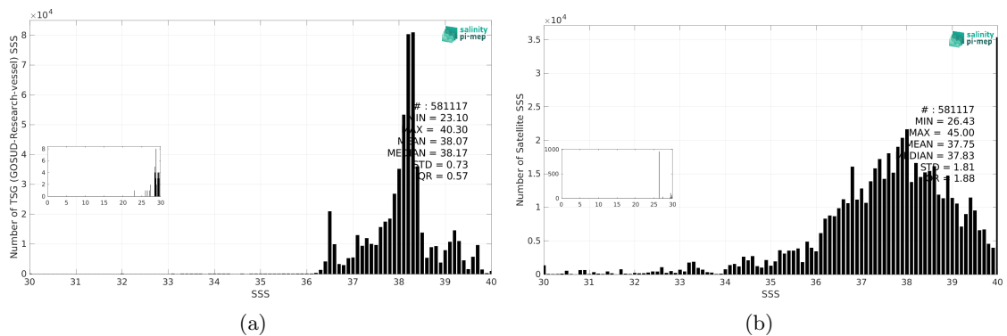
Figure 3: Histograms of SSS from TSG (GOSUD-Research-vessel) (a) and SMAP SSS L2 v5.0 (JPL) (b) considering all match-up pairs per bins of 0.1 over the Mediterranean Sea Pi-MEP region and for the full satellite product period.
