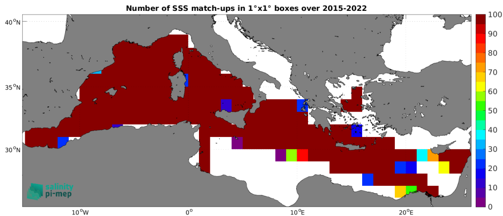
Figure 5: Number of SSS match-ups between TSG (GOSUD-Research-vessel) SSS and the SMAP SSS L2 v5.0 (JPL) SSS product for the Mediterranean Sea Pi-MEP region over 1^\circ \times 1^\circ boxes and for the full satellite product period.
