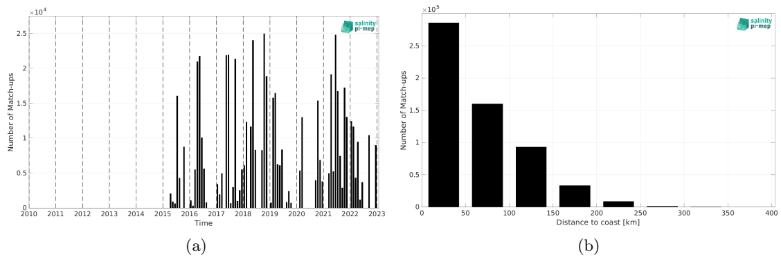
Figure 2: Number of match-ups between TSG (GOSUD-Research-vessel) and SMAP SSS L2 v5.0 (JPL) SSS as a function of time (a) and as function of the distance to coast (b) over the Mediterranean Sea Pi-MEP region and for the full satellite product period.
