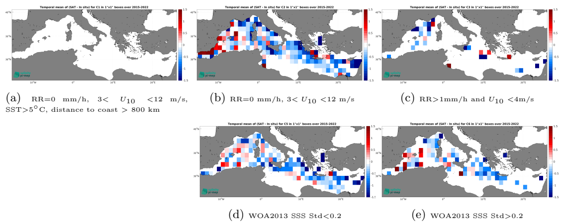
Figure 14: Temporal mean gridded over spatial boxes of size 1^\circ \times 1^\circ of \Delta\text{SSS} (SMAP SSS L2 v5.0 (JPL) - TSG (GOSUD-Research-vessel)) for 5 different subdatasets corresponding to:RR=0 mm/h, 3 < U_{10} < 12 m/s, SST >5^\circ\text{C} , distance to coast > 800 km (a), RR=0 mm/h, 3 < U_{10} < 12 m/s (b), RR >1 mm/h and U_{10} < 4 m/s (c), WOA2013 SSS Std <0.2 (d), WOA2013 SSS Std >0.2 (e).
