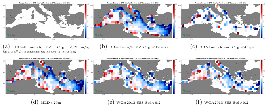
Figure 12: Temporal mean gridded over spatial boxes of size 1^\circ \times 1^\circ of \Delta SSS (SMAP SSS L2 v5.0 (JPL) - Argo) for 6 different subdatasets corresponding to:RR=0 mm/h, 3 < U_{10} < 12 m/s, SST >5^\circ C, distance to coast > 800 km (a), RR=0 mm/h, 3 < U_{10} < 12 m/s (b), RR >1 mm/h and U_{10} < 4 m/s (c),MLD <20 m (d),WOA2013 SSS Std <0.2 (e),WOA2013 SSS Std >0.2 (f).
