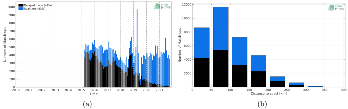
Figure 1: Number of match-ups between Argo and SMAP SSS L2 v5.0 (JPL) SSS as a function of time (a) and as function of the distance to coast (b) over the Mediterranean Sea Pi-MEP region and for the full satellite product period.
