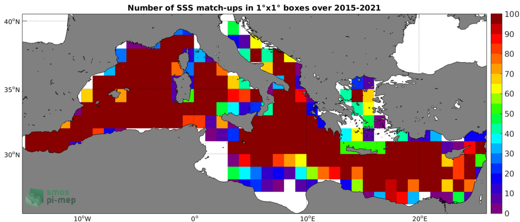
Figure 4: Number of SSS match-ups between Argo SSS and the SMAP SSS L2 v5.0 (JPL) SSS product for the Mediterranean Sea Pi-MEP region over 1^\circ \times 1^\circ boxes and for the full satellite product period.
