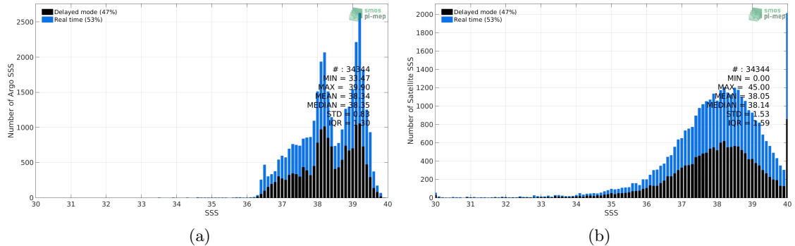
Figure 2: Histograms of SSS from Argo (a) and SMAP SSS L2 v5.0 (JPL) (b) considering all match-up pairs per bins of 0.1 over the Mediterranean Sea Pi-MEP region and for the full satellite product period.
