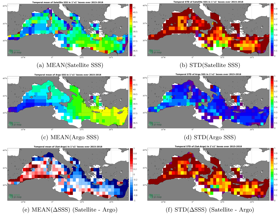
Figure 6: Temporal mean (left) and STD (right) of SSS from SMAP-L2-JPL-V4 (top), Argo (middle), and of \Delta SSS (Satellite - Argo). Only match-up pairs are used to generate these maps.
