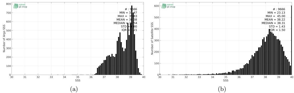
Figure 2: Histograms of SSS from Argo (a) and SMAP-L2-JPL-V4 (b) considering all match-up pairs per bins of 0.1 over the Mediterranean Sea Pi-MEP region and for the full satellite product period.
