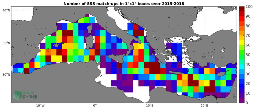
Figure 4: Number of SSS match-ups between Argo SSS and the SMAP-L2-JPL-V4 SSS product for the Mediterranean Sea Pi-MEP region over 1^\circ \times 1^\circ boxes and for the full satellite product period.
