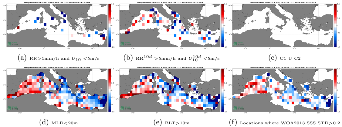
Figure 12: Temporal mean gridded over spatial boxes of size 1°x1° of \Delta SSS (SMAP-L2-JPL-V4 - Argo) for 6 different subdatasets corresponding to: RR>1mm/h and U_{10} < 5m/s (a), RR^{10d} > 5mm/h and U_{10}^{10d} < 5m/s (b), C1 U C2 (c), MLD<20m (d), BLT>10m (e), Locations where WOA2013 SSS STD>0.2 (f).
