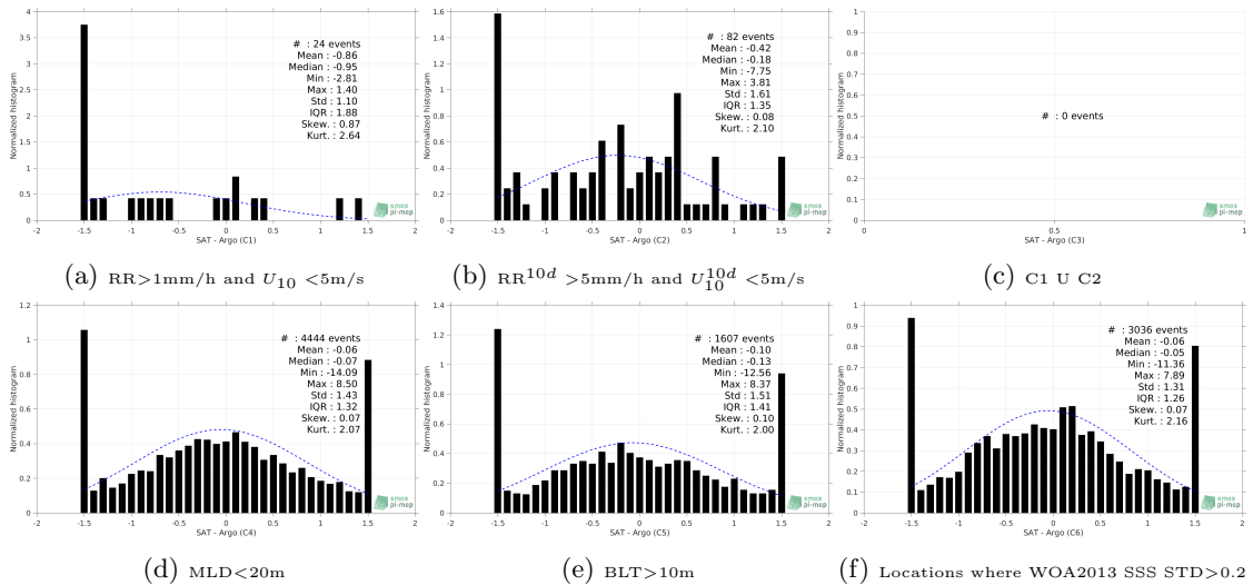
Figure 13: Normalized histogram of \Delta SSS (SMAP-L2-JPL-V4 - Argo) for 6 different subdatasets corresponding to: RR>1mm/h and U_{10} < 5m/s (a), RR^{10d} > 5mm/h and U_{10}^{10d} < 5m/s (b), C1 U C2 (c), MLD<20m (d), BLT>10m (e), Locations where WOA2013 SSS STD>0.2 (f).
