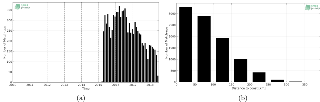
Figure 1: Number of match-ups between Argo and SMAP-L2-JPL-V4 SSS as a function of time (a) and as function of the distance to coast (b) over the Mediterranean Sea Pi-MEP region and for the full satellite product period.
