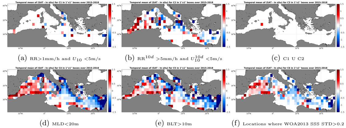
Figure 12: Temporal mean gridded over spatial boxes of size 1°x1° of \Delta SSS (SMAP-L2-JPL-V4 - Argo) for 6 different subdatasets corresponding to:RR>1mm/h and U_{10} < 5m/s (a), RR^{10d} > 5mm/h and U_{10}^{10d} < 5m/s (b), C1 U C2 (c),MLD<20m (d),BLT>10m (e),Locations where WOA2013 SSS STD>0.2 (f).
