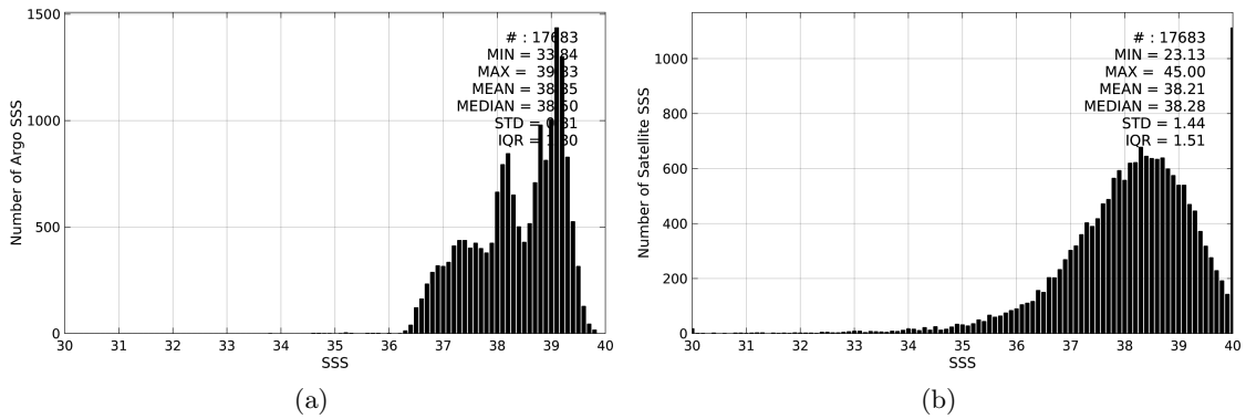
Figure 2: Histograms of SSS from Argo (a) and SMAP-L2-JPL-V4 (b) considering all match-up pairs per bins of 0.1 over the Mediterranean Sea Pi-MEP region and for the full satellite product period.
