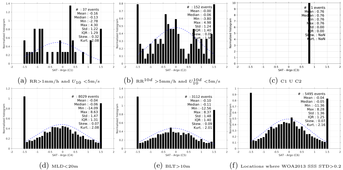
Figure 13: Normalized histogram of \Delta SSS (SMAP-L2-JPL-V4 - Argo) for 6 different subdatasets corresponding to: RR>1mm/h and U_{10} < 5m/s (a), RR^{10d} > 5mm/h and U_{10}^{10d} < 5m/s (b), C1 U C2 (c),MLD<20m (d),BLT>10m (e),Locations where WOA2013 SSS STD>0.2 (f).
