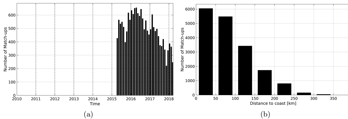
Figure 1: Number of match-ups between Argo and SMAP-L2-JPL-V4 SSS as a function of time (a) and as function of the distance to coast (b) over the Mediterranean Sea Pi-MEP region and for the full satellite product period.
