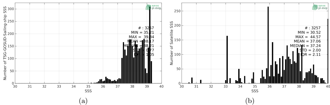
Figure 2: Histograms of SSS from TSG-GOSUD-Sailing-ship (a) and SMAP-L2-JPL-V4.2 (b) considering all match-up pairs per bins of 0.1 over the Mediterranean Sea Pi-MEP region and for the full satellite product period.
