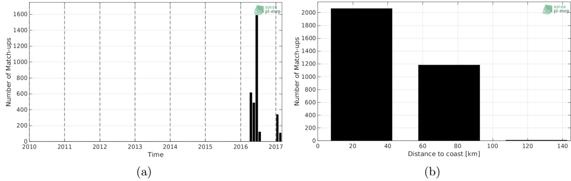
Figure 1: Number of match-ups between TSG-GOSUD-Sailing-ship and SMAP-L2-JPL-V4.2 SSS as a function of time (a) and as function of the distance to coast (b) over the Mediterranean Sea Pi-MEP region and for the full satellite product period.
