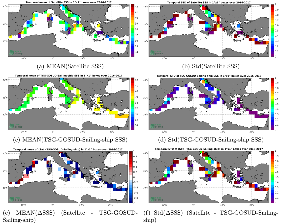
Figure 6: Temporal mean (left) and Std (right) of SSS from SMAP-L2-JPL-V4.2 (top), TSG-GOSUD-Sailing-ship (middle), and of \Delta SSS (Satellite - TSG-GOSUD-Sailing-ship). Only match-up pairs are used to generate these maps.
