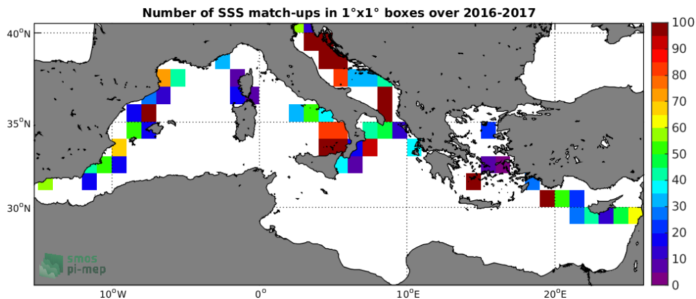
Figure 4: Number of SSS match-ups between TSG-GOSUD-Sailing-ship SSS and the SMAP-L2-JPL-V4.2 SSS product for the Mediterranean Sea Pi-MEP region over 1^\circ \times 1^\circ boxes and for the full satellite product period.
