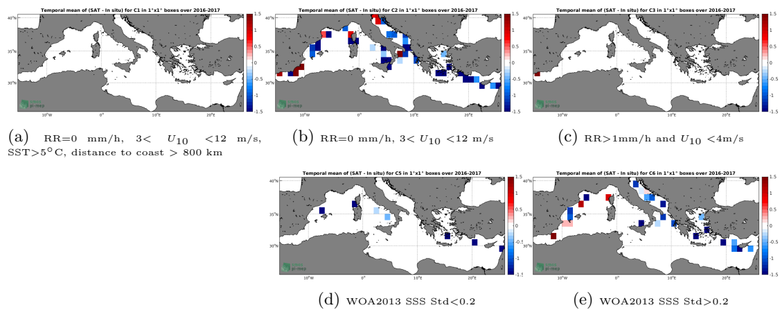
Figure 12: Temporal mean gridded over spatial boxes of size 1^\circ \times 1^\circ of \Delta SSS (SMAP-L2-JPL-V4.2 - TSG-GOSUD-Sailing-ship) for 5 different subdatasets corresponding to:RR=0 mm/h, 3 < U_{10} < 12 m/s, SST >5^\circ\text{C} , distance to coast > 800 km (a), RR=0 mm/h, 3 < U_{10} < 12 m/s (b), RR >1 mm/h and U_{10} < 4 m/s (c), WOA2013 SSS Std <0.2 (d), WOA2013 SSS Std >0.2 (e).
