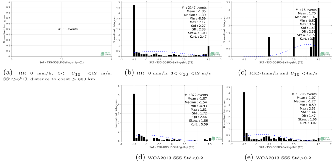
Figure 13: Normalized histogram of \Delta\text{SSS} (SMAP-L2-JPL-V4.2 - TSG-GOSUD-Sailing-ship) for 5 different subdatasets corresponding to: RR=0 mm/h, 3 < U_{10} < 12 m/s, SST > 5^\circ\text{C} , distance to coast > 800 km (a), RR=0 mm/h, 3 < U_{10} < 12 m/s (b), RR > 1\text{mm/h} and U_{10} < 4\text{m/s} (c), WOA2013 SSS Std < 0.2 (d), WOA2013 SSS Std > 0.2 (e).
