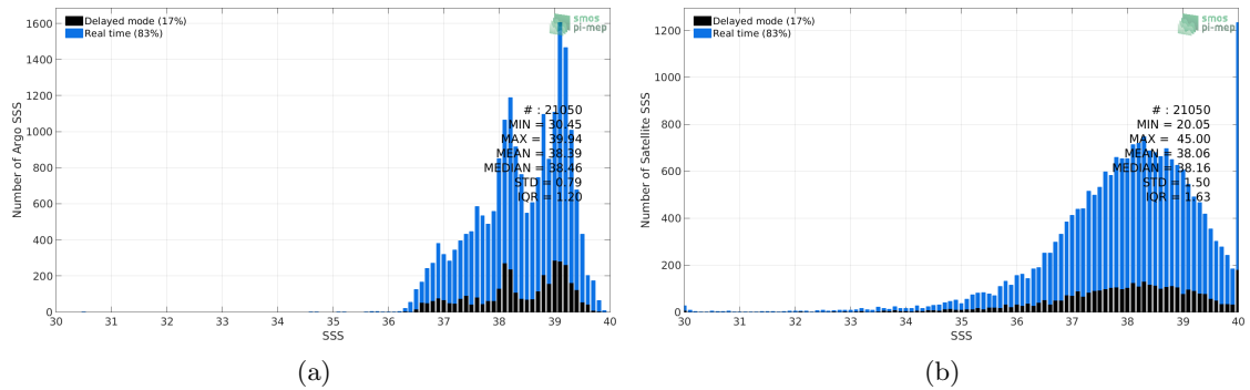
Figure 2: Histograms of SSS from Argo (a) and SMAP-L2-JPL-V4.2 (b) considering all match-up pairs per bins of 0.1 over the Mediterranean Sea Pi-MEP region and for the full satellite product period.
