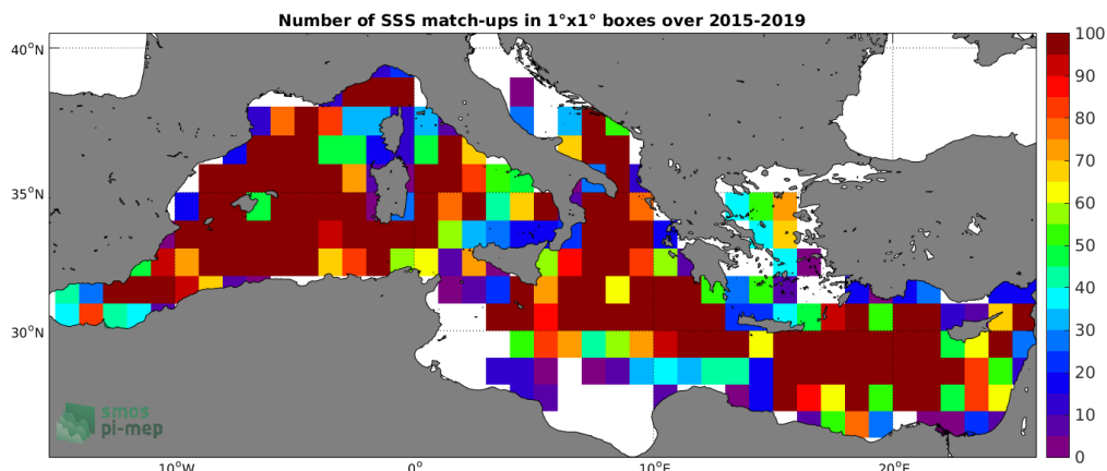
Figure 4: Number of SSS match-ups between Argo SSS and the SMAP-L2-JPL-V4.2 SSS product for the Mediterranean Sea Pi-MEP region over 1^\circ \times 1^\circ boxes and for the full satellite product period.
