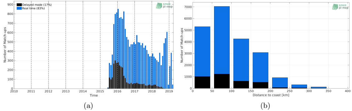
Figure 1: Number of match-ups between Argo and SMAP-L2-JPL-V4.2 SSS as a function of time (a) and as function of the distance to coast (b) over the Mediterranean Sea Pi-MEP region and for the full satellite product period.
