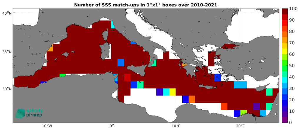
Figure 5: Number of SSS match-ups between TSG (GOSUD-Research-vessel) SSS and the ISAS SSS product for the Mediterranean Sea Pi-MEP region over 1^\circ \times 1^\circ boxes and for the full satellite product period.
