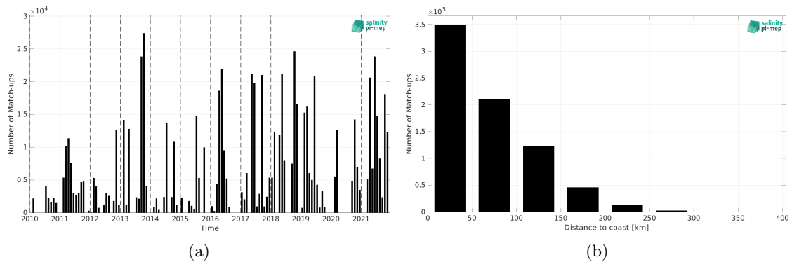
Figure 2: Number of match-ups between TSG (GOSUD-Research-vessel) and ISAS SSS as a function of time (a) and as function of the distance to coast (b) over the Mediterranean Sea Pi-MEP region and for the full satellite product period.
