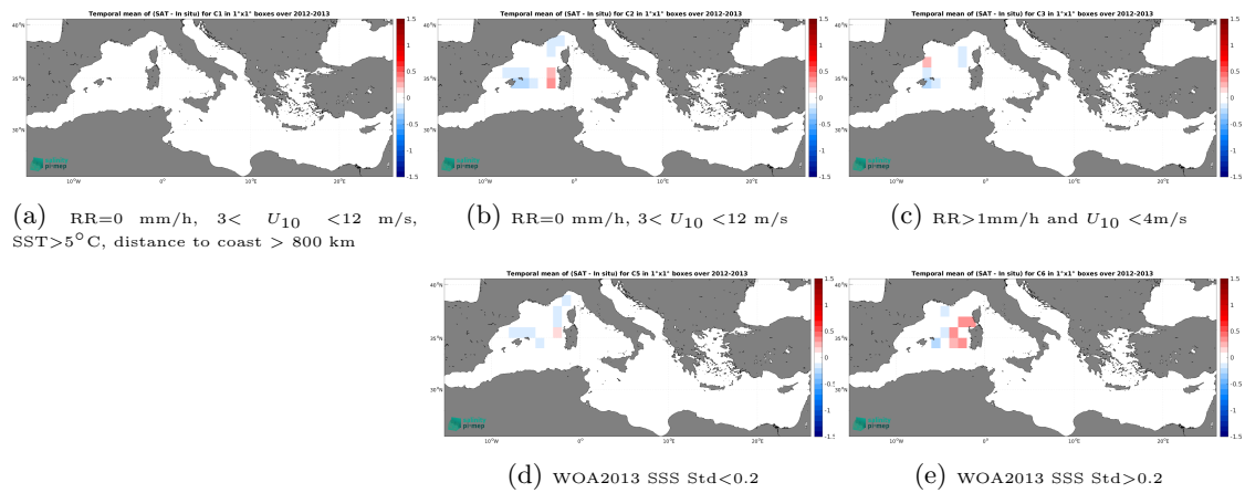
Figure 13: Temporal mean gridded over spatial boxes of size 1^\circ \times 1^\circ of \Delta SSS (ISAS - Surface drifters) for 5 different subdatasets corresponding to:RR=0 mm/h, 3 < U_{10} < 12 m/s, SST >5^\circ C, distance to coast > 800 km (a), RR=0 mm/h, 3 < U_{10} < 12 m/s (b), RR >1 mm/h and U_{10} < 4 m/s (c), WOA2013 SSS Std <0.2 (d), WOA2013 SSS Std >0.2 (e).
