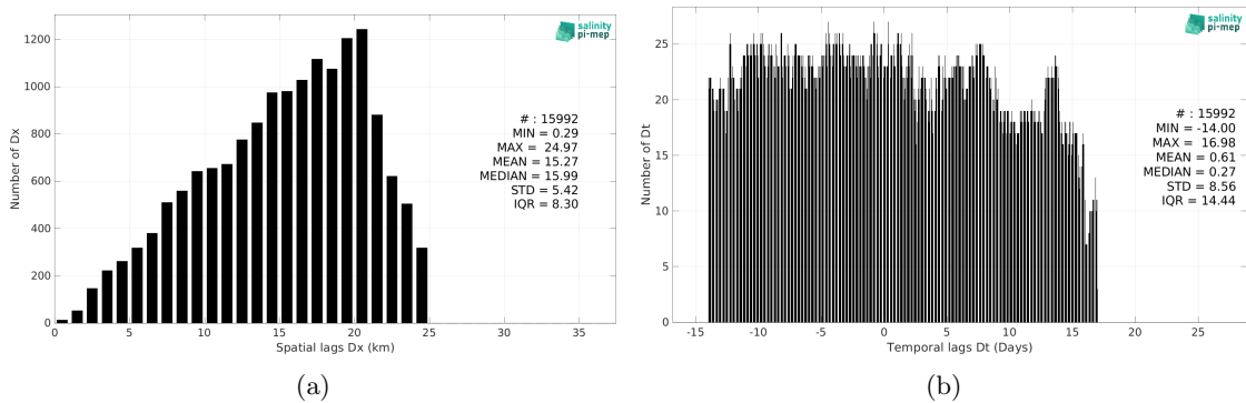
Figure 5: Histograms of the spatial (a) and temporal (b) lags between the location/time of the Surface drifters measurement and the date of the corresponding ISAS SSS pixel.
