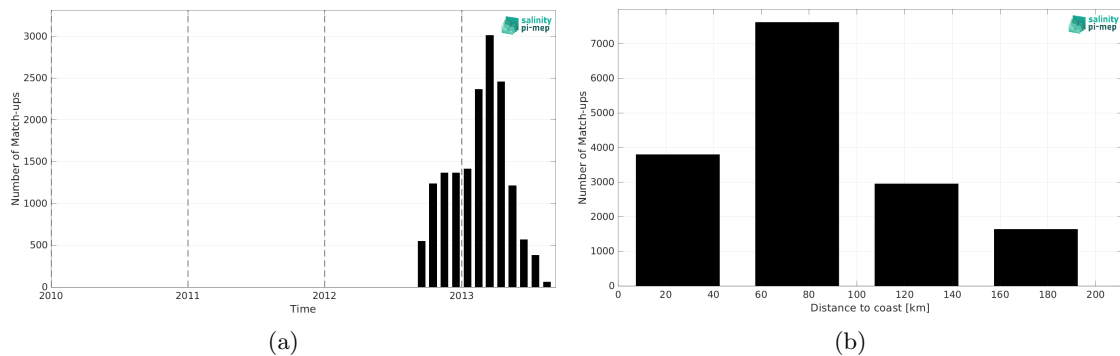
Figure 2: Number of match-ups between Surface drifters and ISAS SSS as a function of time (a) and as function of the distance to coast (b) over the Mediterranean Sea Pi-MEP region and for the full satellite product period.
