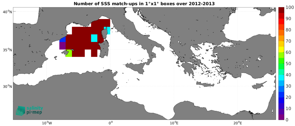
Figure 4: Number of SSS match-ups between Surface drifters SSS and the ISAS SSS product for the Mediterranean Sea Pi-MEP region over 1^\circ \times 1^\circ boxes and for the full satellite product period.
