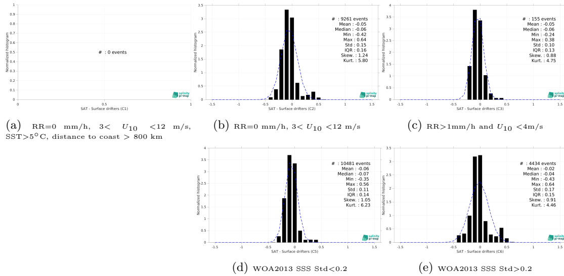
Figure 14: Normalized histogram of \Delta SSS (ISAS - Surface drifters) for 5 different subdatasets corresponding to: RR=0 mm/h, 3 < U_{10} < 12 m/s, SST > 5°C, distance to coast > 800 km (a), RR=0 mm/h, 3 < U_{10} < 12 m/s (b), RR > 1mm/h and U_{10} < 4 m/s (c), WOA2013 SSS Std < 0.2 (d), WOA2013 SSS Std > 0.2 (e).
