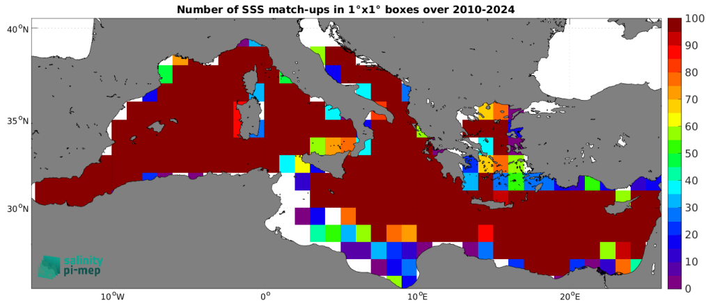
Figure 5: Number of SSS match-ups between Argo SSS and the ISAS v7 - Monthly (Ifremer-LOPS-CMEMS) SSS product for the Mediterranean Sea Pi-MEP region over 1^\circ \times 1^\circ boxes and for the full satellite product period.
