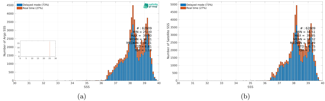
Figure 3: Histograms of SSS from Argo (a) and ISAS v7 - Monthly (Ifremer-LOPS-CMEMS) (b) considering all match-up pairs per bins of 0.1 over the Mediterranean Sea Pi-MEP region and for the full satellite product period.
