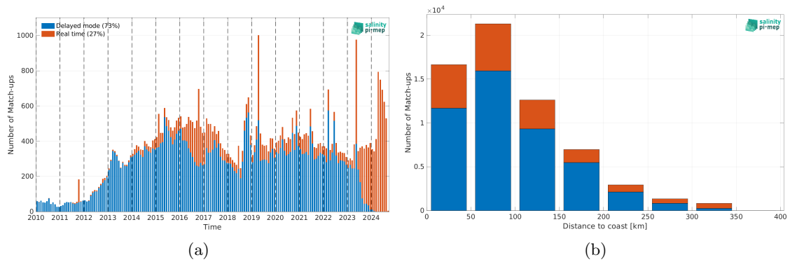
Figure 2: Number of match-ups between Argo and ISAS v7 - Monthly (Ifremer-LOPS-CMEMS) SSS as a function of time (a) and as function of the distance to coast (b) over the Mediterranean Sea Pi-MEP region and for the full satellite product period.
