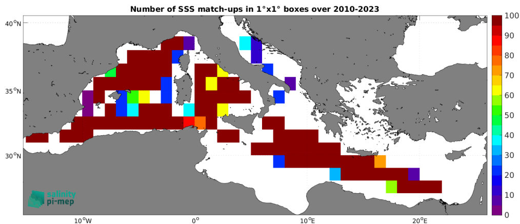
Figure 5: Number of SSS match-ups between TSG (LEGOS-DM) SSS and the CCI SSS L4 Merged-OI v5.5 - 7-day running (ESA) SSS product for the Mediterranean Sea Pi-MEP region over 1^\circ \times 1^\circ boxes and for the full satellite product period.
