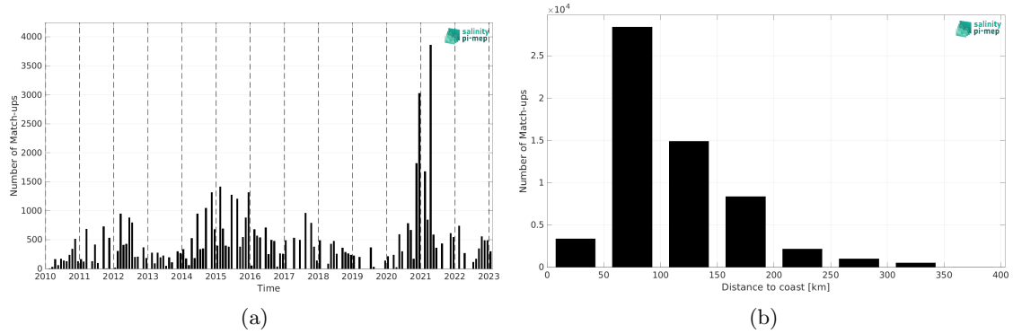
Figure 2: Number of match-ups between TSG (LEGOS-DM) and CCI SSS L4 Merged-OI v5.5 - 7-day running (ESA) SSS as a function of time (a) and as function of the distance to coast (b) over the Mediterranean Sea Pi-MEP region and for the full satellite product period.
