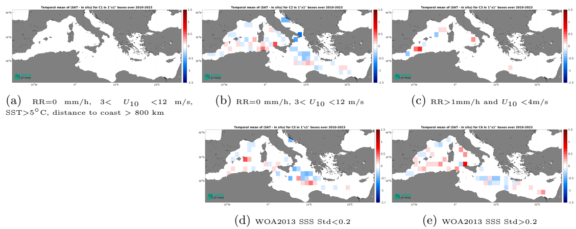
Figure 14: Temporal mean gridded over spatial boxes of size 1^\circ \times 1^\circ of \Delta\text{SSS} (CCI SSS L4 Merged-OI v5.5 - 7-day running (ESA) - TSG (LEGOS-DM)) for 5 different subdatasets corresponding to:RR=0 mm/h, 3 < U_{10} < 12 m/s, SST>5°C, distance to coast > 800 km (a), RR=0 mm/h, 3 < U_{10} < 12 m/s (b), RR>1mm/h and U_{10} < 4 m/s (c), WOA2013 SSS Std<0.2 (d), WOA2013 SSS Std>0.2 (e).
