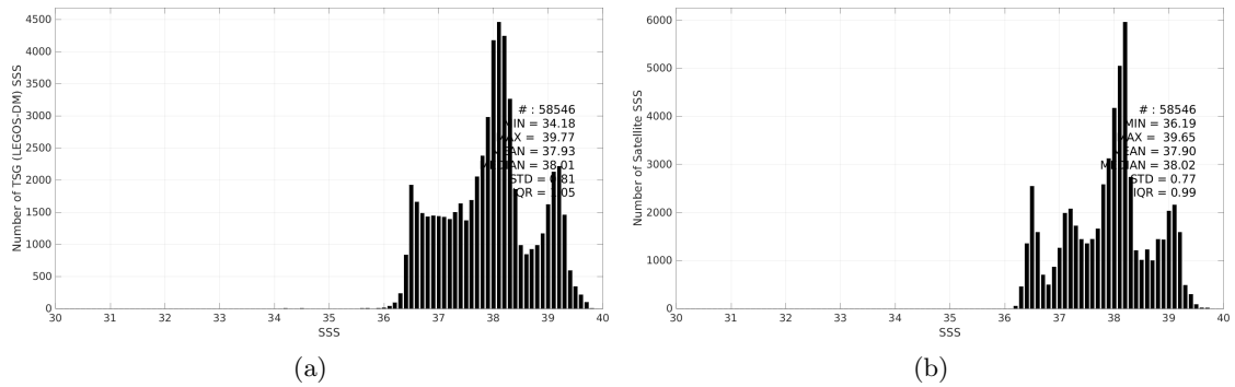
Figure 3: Histograms of SSS from TSG (LEGOS-DM) (a) and CCI SSS L4 Merged-OI v5.5 - 7-day running (ESA) (b) considering all match-up pairs per bins of 0.1 over the Mediterranean Sea Pi-MEP region and for the full satellite product period.
