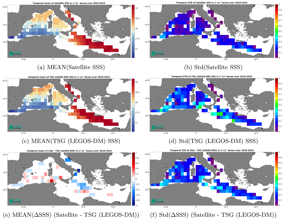
Figure 7: Temporal mean (left) and Std (right) of SSS from CCI SSS L4 Merged-OI v5.5 - 7-day running (ESA) (top), TSG (LEGOS-DM) (middle), and of \Delta SSS (Satellite - TSG (LEGOS-DM)). Only match-up pairs are used to generate these maps.
