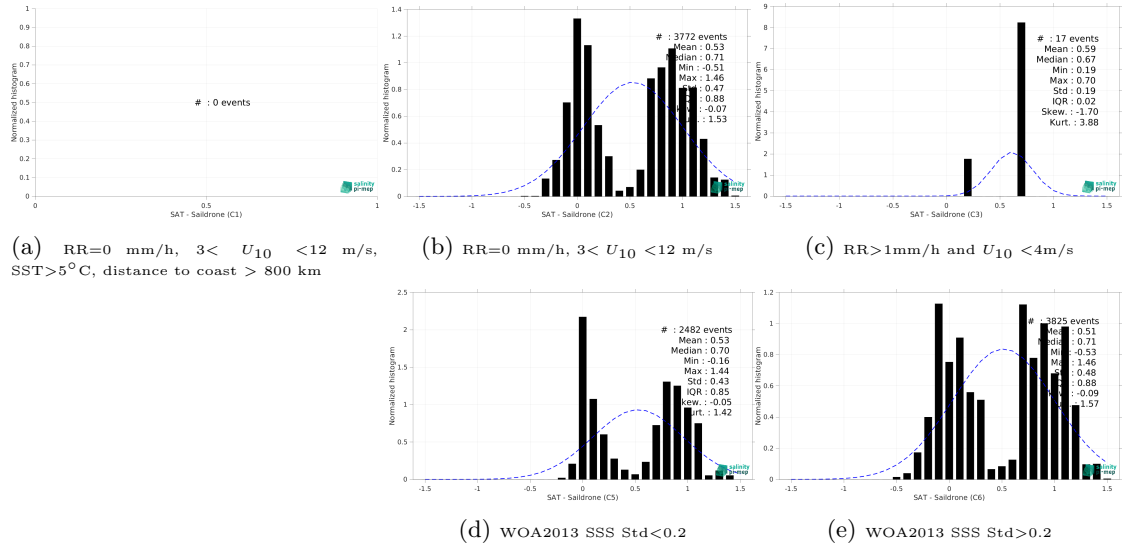
Figure 15: Normalized histogram of \Delta\text{SSS} (CCI SSS L4 Merged-OI v5.5 - 7-day running (ESA) - Saldrone) for 5 different subdatasets corresponding to: RR=0 mm/h, 3 < U_{10} < 12 m/s, SST > 5^{\circ}\text{C} , distance to coast > 800 km (a), RR=0 mm/h, 3 < U_{10} < 12 m/s (b), RR > 1\text{mm/h} and U_{10} < 4\text{m/s} (c), WOA2013 SSS Std < 0.2 (d), WOA2013 SSS Std > 0.2 (e).
