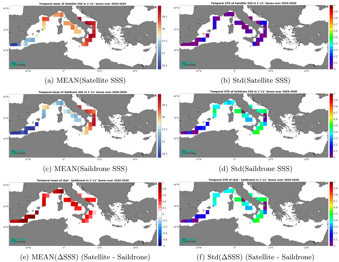
Figure 7: Temporal mean (left) and Std (right) of SSS from CCI SSS L4 Merged-OI v5.5 - 7-day running (ESA) (top), Saildrone (middle), and of \Delta SSS (Satellite - Saildrone). Only match-up pairs are used to generate these maps.
