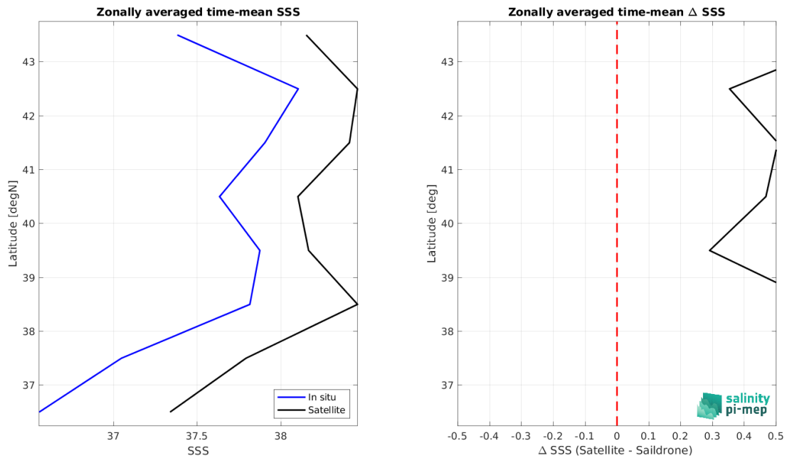
Figure 9: Left panel: Zonal mean SSS from CCI SSS L4 Merged-OI v5.5 - 7-day running (ESA) satellite product (black) and from Sairdrone (blue). Right panel: Zonal mean of \Delta SSS (Satellite - Sairdrone) for all the collected Pi-MEP match-up pairs estimated over the full satellite product period.
