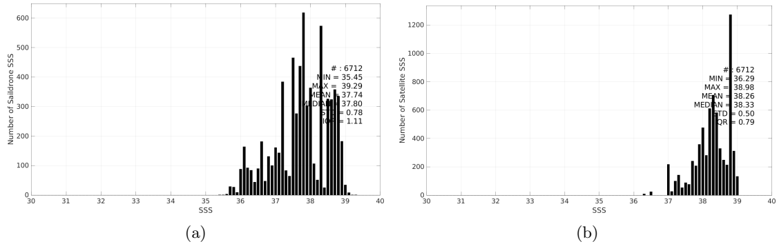
Figure 3: Histograms of SSS from Saildrone (a) and CCI SSS L4 Merged-OI v5.5 - 7-day running (ESA) (b) considering all match-up pairs per bins of 0.1 over the Mediterranean Sea Pi-MEP region and for the full satellite product period.
