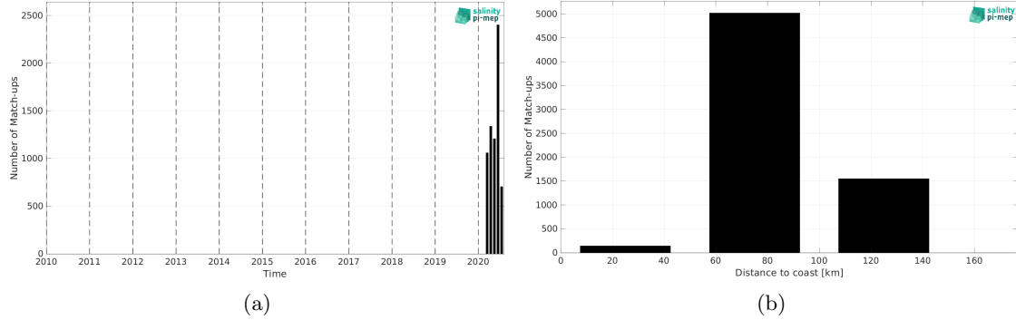
Figure 2: Number of match-ups between Saildrone and CCI SSS L4 Merged-OI v5.5 - 7-day running (ESA) SSS as a function of time (a) and as function of the distance to coast (b) over the Mediterranean Sea Pi-MEP region and for the full satellite product period.
