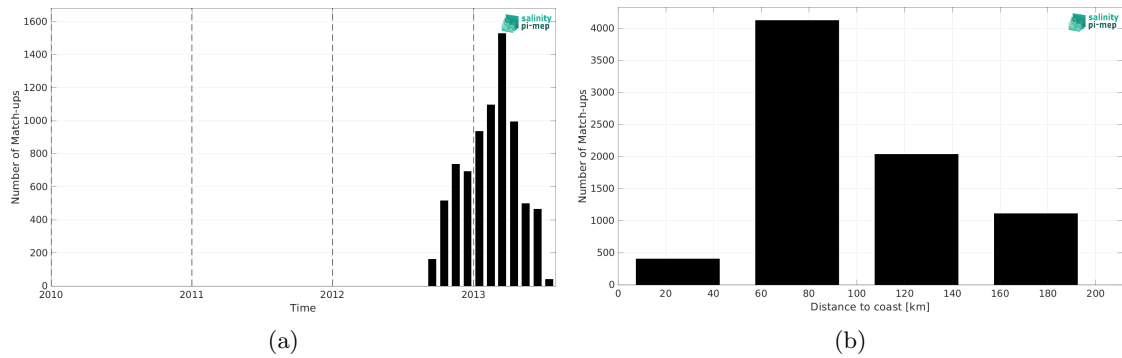
Figure 2: Number of match-ups between Surface drifters and CCI SSS L4 Merged-OI v5.5 - 7-day running (ESA) SSS as a function of time (a) and as function of the distance to coast (b) over the Mediterranean Sea Pi-MEP region and for the full satellite product period.
