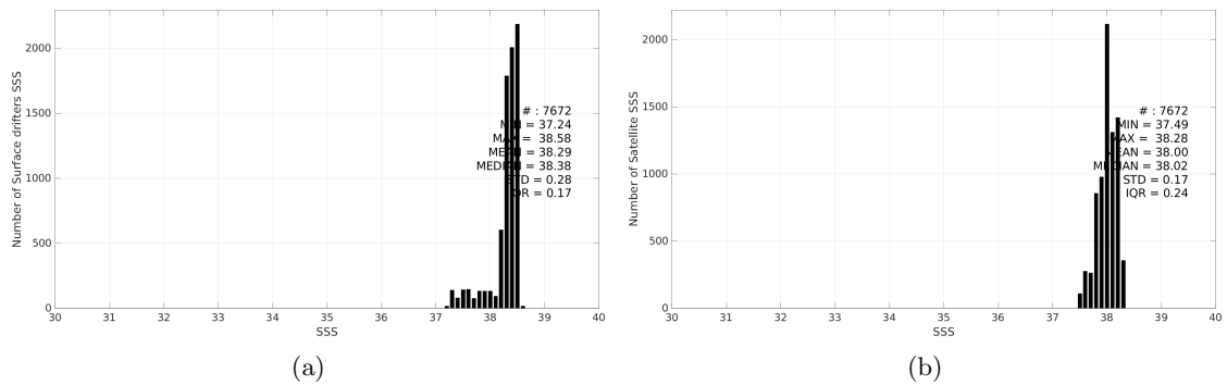
Figure 3: Histograms of SSS from Surface drifters (a) and CCI SSS L4 Merged-OI v5.5 - 7-day running (ESA) (b) considering all match-up pairs per bins of 0.1 over the Mediterranean Sea Pi-MEP region and for the full satellite product period.
