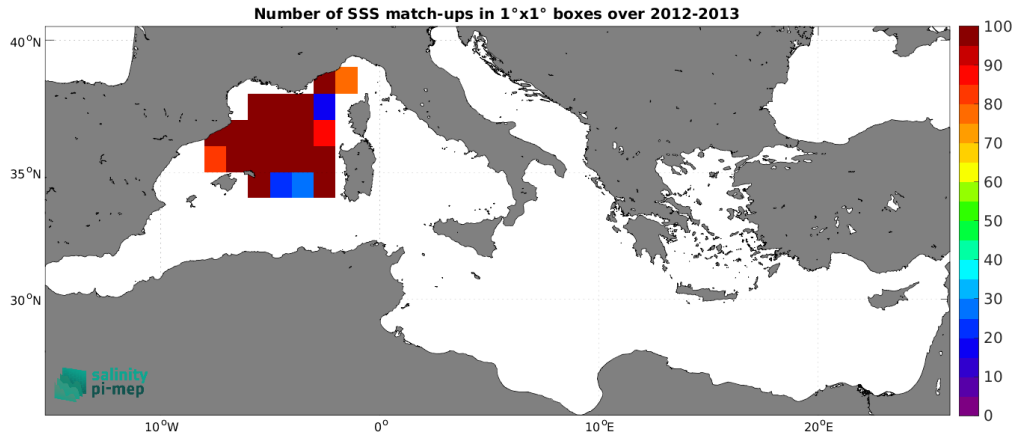
Figure 4: Number of SSS match-ups between Surface drifters SSS and the CCI SSS L4 Merged-OI v5.5 - 7-day running (ESA) SSS product for the Mediterranean Sea Pi-MEP region over 1^\circ \times 1^\circ boxes and for the full satellite product period.
