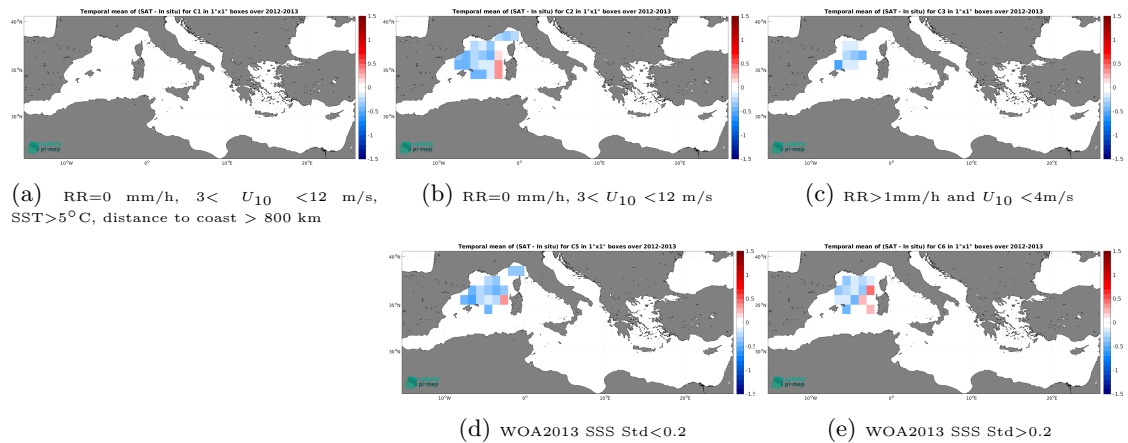
Figure 13: Temporal mean gridded over spatial boxes of size 1^\circ \times 1^\circ of \Delta SSS (CCI SSS L4 Merged-OI v5.5 - 7-day running (ESA) - Surface drifters) for 5 different subdatasets corresponding to:RR=0 mm/h, 3 < U_{10} < 12 m/s, SST >5^\circ\text{C} , distance to coast > 800 km (a), RR=0 mm/h, 3 < U_{10} < 12 m/s (b), RR >1 mm/h and U_{10} < 4 m/s (c), WOA2013 SSS Std <0.2 (d), WOA2013 SSS Std >0.2 (e).
