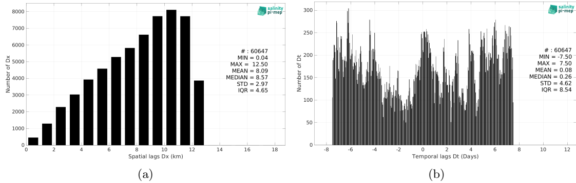
Figure 6: Histograms of the spatial (a) and temporal (b) lags between the location/time of the TSG (LEGOS-DM) measurement and the date of the corresponding CCI SSS L4 Merged-OI v5.5 - 30-day running (ESA) SSS pixel.
