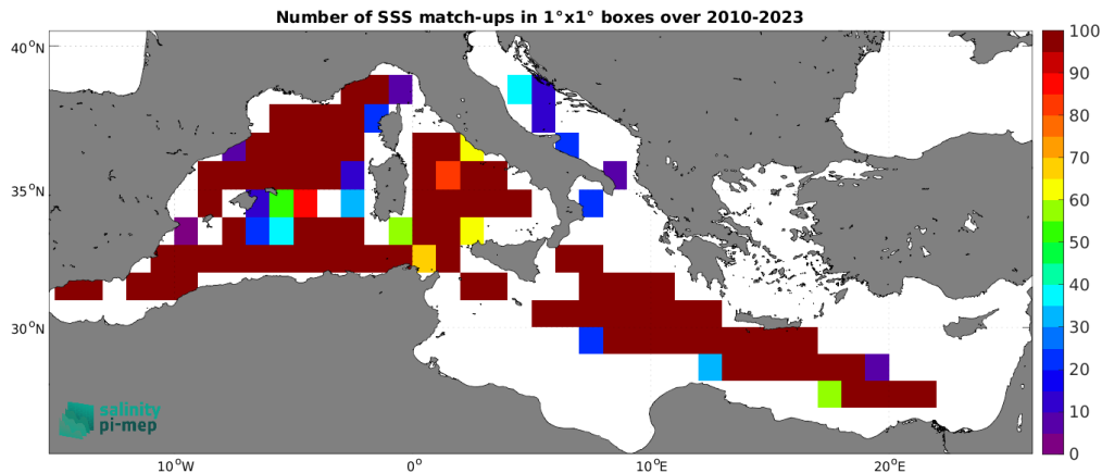
Figure 5: Number of SSS match-ups between TSG (LEGOS-DM) SSS and the CCI SSS L4 Merged-OI v5.5 - 30-day running (ESA) SSS product for the Mediterranean Sea Pi-MEP region over 1^\circ \times 1^\circ boxes and for the full satellite product period.
