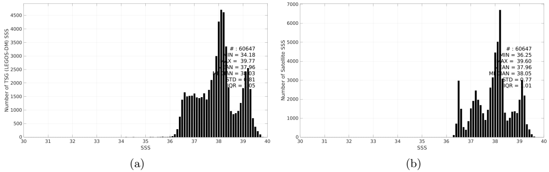
Figure 3: Histograms of SSS from TSG (LEGOS-DM) (a) and CCI SSS L4 Merged-OI v5.5 - 30-day running (ESA) (b) considering all match-up pairs per bins of 0.1 over the Mediterranean Sea Pi-MEP region and for the full satellite product period.
