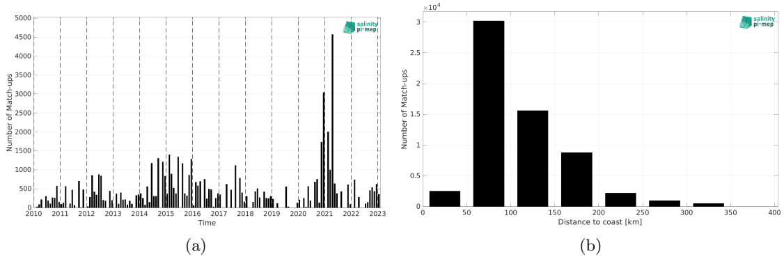
Figure 2: Number of match-ups between TSG (LEGOS-DM) and CCI SSS L4 Merged-OI v5.5 - 30-day running (ESA) SSS as a function of time (a) and as function of the distance to coast (b) over the Mediterranean Sea Pi-MEP region and for the full satellite product period.
