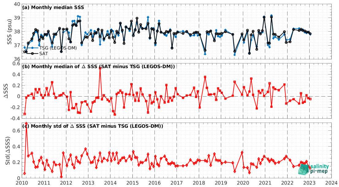
Figure 8: Time series of the monthly median SSS (top), median of \Delta\text{SSS} (Satellite - TSG (LEGOS-DM)) and Std of \Delta\text{SSS} (Satellite - TSG (LEGOS-DM)) over the Mediterranean Sea Pi-MEP region considering all match-ups collected by the Pi-MEP.
