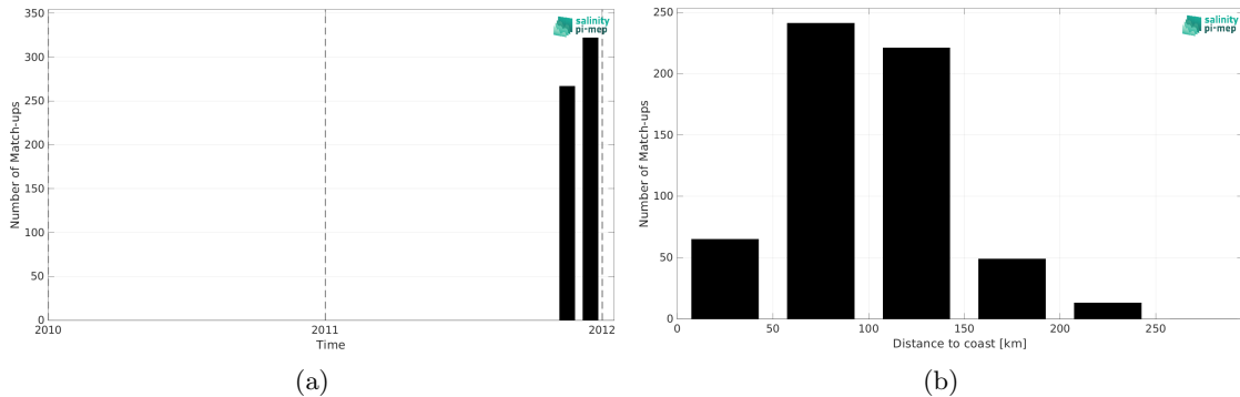
Figure 2: Number of match-ups between TSG (SAMOS) and CCI SSS L4 Merged-OI v4.41 - 7-day running (ESA) SSS as a function of time (a) and as function of the distance to coast (b) over the Mediterranean Sea Pi-MEP region and for the full satellite product period.
