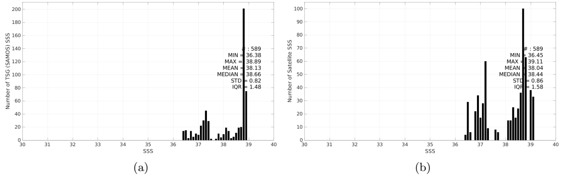
Figure 3: Histograms of SSS from TSG (SAMOS) (a) and CCI SSS L4 Merged-OI v4.41 - 7-day running (ESA) (b) considering all match-up pairs per bins of 0.1 over the Mediterranean Sea Pi-MEP region and for the full satellite product period.
