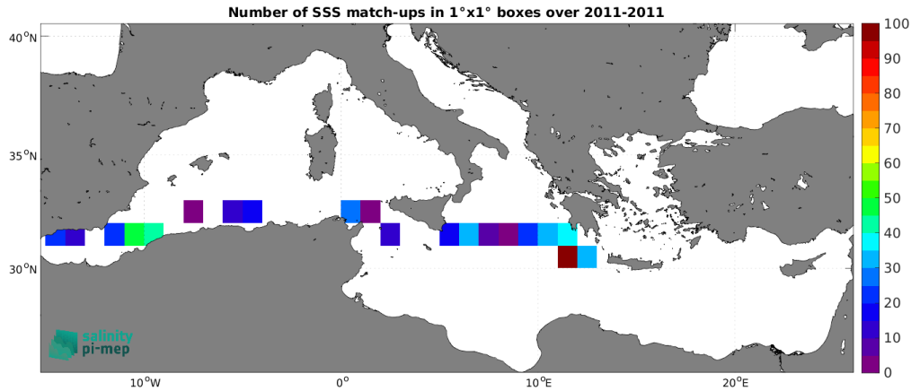
Figure 5: Number of SSS match-ups between TSG (SAMOS) SSS and the CCI SSS L4 Merged-OI v4.41 - 7-day running (ESA) SSS product for the Mediterranean Sea Pi-MEP region over 1^\circ \times 1^\circ boxes and for the full satellite product period.
