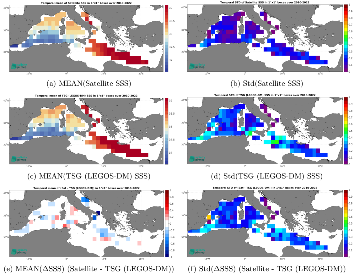
Figure 7: Temporal mean (left) and Std (right) of SSS from CCI SSS L4 Merged-OI v4.41 - 7-day running (ESA) (top), TSG (LEGOS-DM) (middle), and of \Delta\text{SSS}(\text{Satellite} - \text{TSG (LEGOS-DM)}) . Only match-up pairs are used to generate these maps.
