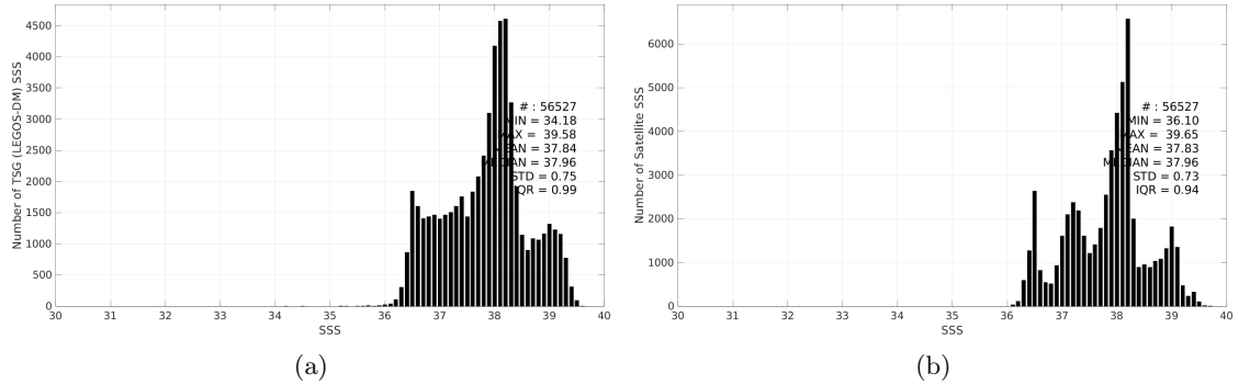
Figure 3: Histograms of SSS from TSG (LEGOS-DM) (a) and CCI SSS L4 Merged-OI v4.41 - 7-day running (ESA) (b) considering all match-up pairs per bins of 0.1 over the Mediterranean Sea Pi-MEP region and for the full satellite product period.
