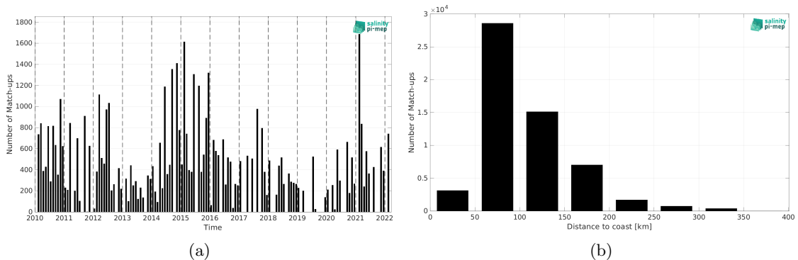
Figure 2: Number of match-ups between TSG (LEGOS-DM) and CCI SSS L4 Merged-OI v4.41 - 7-day running (ESA) SSS as a function of time (a) and as function of the distance to coast (b) over the Mediterranean Sea Pi-MEP region and for the full satellite product period.
