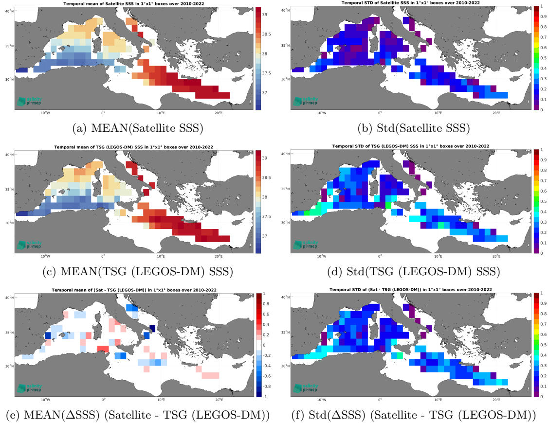
Figure 7: Temporal mean (left) and Std (right) of SSS from CCI SSS L4 Merged-OI v4.41 - 7-day running (ESA) (top), TSG (LEGOS-DM) ( in situ ) dataset (middle), and of \Delta\text{SSS} (Satellite - TSG (LEGOS-DM)). Only match-up pairs are used to generate these maps.
