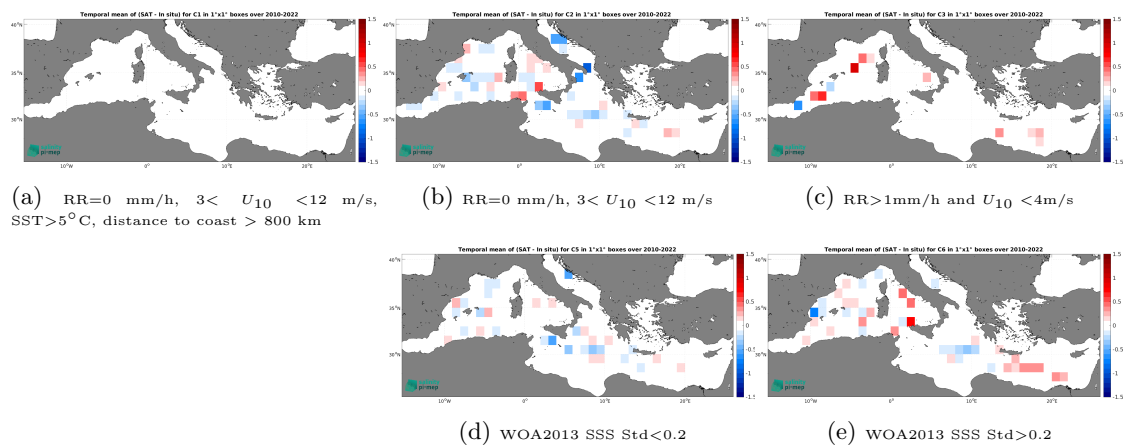
Figure 14: Temporal mean gridded over spatial boxes of size 1^\circ \times 1^\circ of \Delta\text{SSS} (CCI SSS L4 Merged-OI v4.41 - 7-day running (ESA) - TSG (LEGOS-DM)) for 5 different subdatasets corresponding to:RR=0 mm/h, 3 < U_{10} < 12 m/s, SST>5°C, distance to coast > 800 km (a), RR=0 mm/h, 3 < U_{10} < 12 m/s (b), RR>1mm/h and U_{10} < 4 m/s (c), WOA2013 SSS Std<0.2 (d), WOA2013 SSS Std>0.2 (e).
