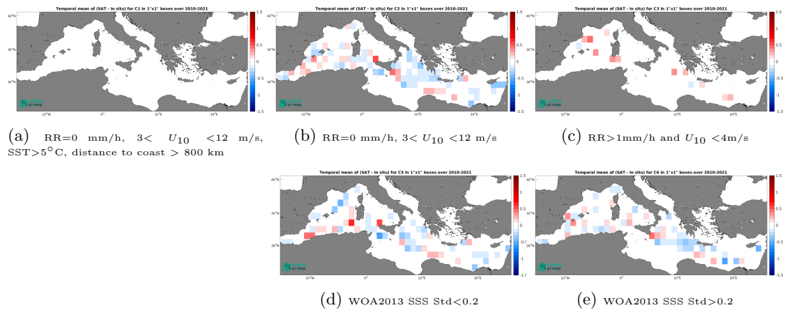
Figure 14: Temporal mean gridded over spatial boxes of size 1^\circ \times 1^\circ of \Delta SSS (CCI SSS L4 Merged-OI v4.41 - 7-day running (ESA) - TSG (GOSUD-Research-vessel)) for 5 different subdatasets corresponding to:RR=0 mm/h, 3 < U_{10} < 12 m/s, SST >5^\circ C, distance to coast > 800 km (a), RR=0 mm/h, 3 < U_{10} < 12 m/s (b), RR >1 mm/h and U_{10} < 4 m/s (c), WOA2013 SSS Std <0.2 (d), WOA2013 SSS Std >0.2 (e).
