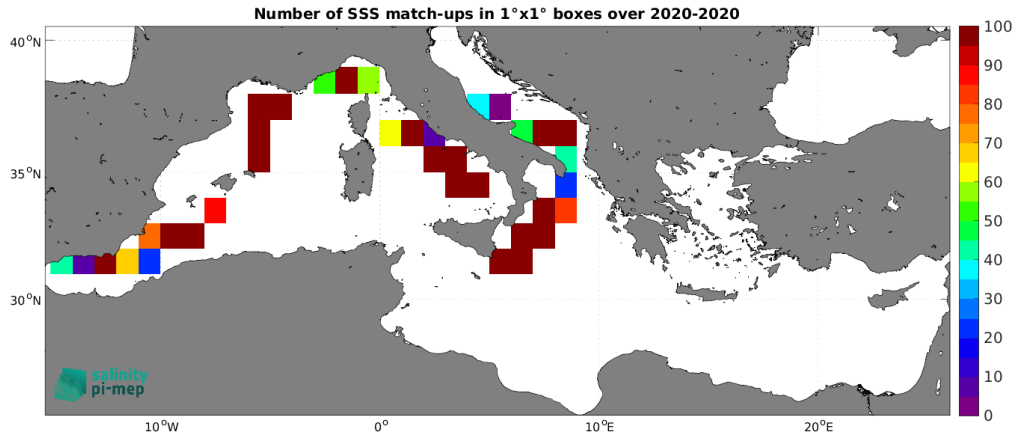
Figure 5: Number of SSS match-ups between Saildrone SSS and the CCI SSS L4 Merged-OI v4.41 - 7-day running (ESA) SSS product for the Mediterranean Sea Pi-MEP region over 1^\circ \times 1^\circ boxes and for the full satellite product period.
