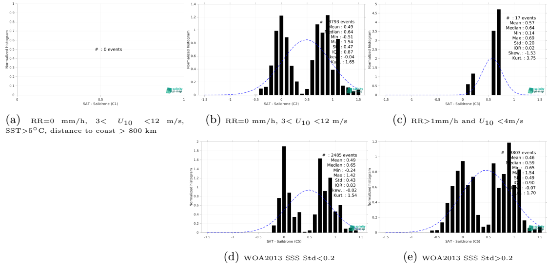
Figure 15: Normalized histogram of \Delta SSS (CCI SSS L4 Merged-OI v4.41 - 7-day running (ESA) - Saildrone) for 5 different subdatasets corresponding to: RR=0 mm/h, 3 < U_{10} < 12 m/s, SST > 5°C, distance to coast > 800 km (a), RR=0 mm/h, 3 < U_{10} < 12 m/s (b), RR > 1mm/h and U_{10} < 4 m/s (c), WOA2013 SSS Std < 0.2 (d), WOA2013 SSS Std > 0.2 (e).
