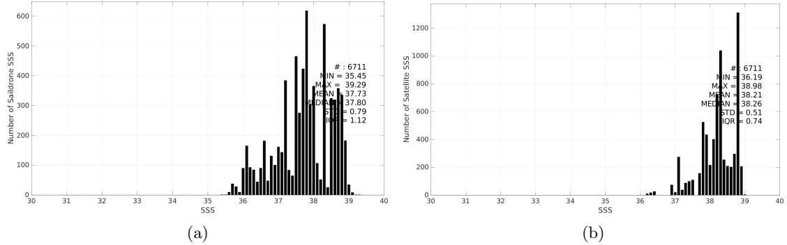
Figure 3: Histograms of SSS from Saildrone (a) and CCI SSS L4 Merged-OI v4.41 - 7-day running (ESA) (b) considering all match-up pairs per bins of 0.1 over the Mediterranean Sea Pi-MEP region and for the full satellite product period.
