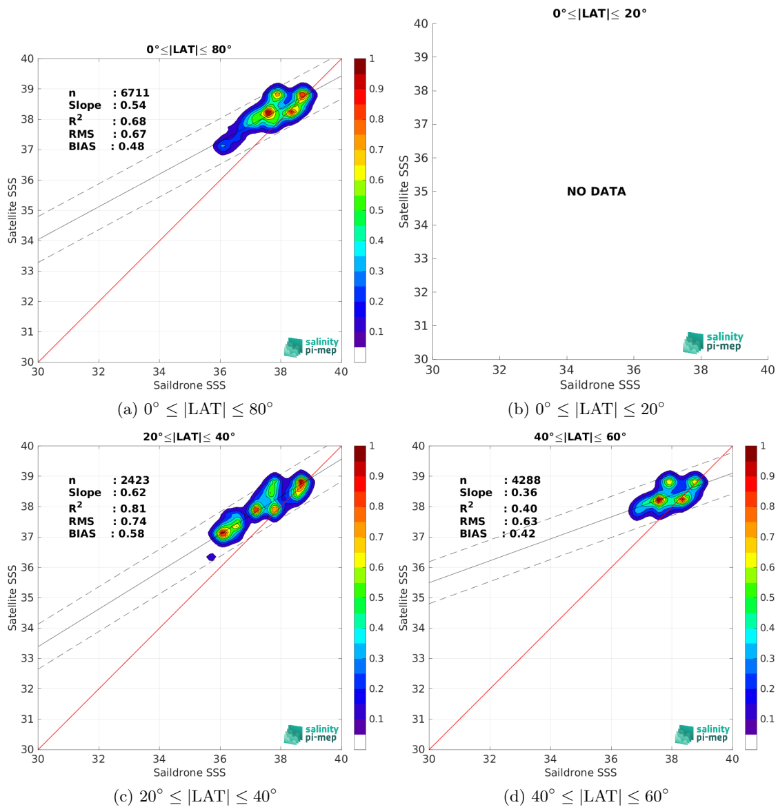
Figure 10: Contour maps of the concentration of CCI SSS L4 Merged-OI v4.41 - 7-day running (ESA) SSS (y-axis) versus Saldrone SSS (x-axis) at match-up pairs for different latitude bands. For each plot, the red line shows x=y . The black thin and dashed lines indicate a linear fit through the data cloud and the \pm 95\% confidence levels, respectively. The number match-up pairs n , the slope and R^2 coefficient of the linear fit, the root mean square (RMS) and the mean bias between satellite and in situ data are indicated for each latitude band in each plots.
