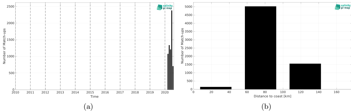
Figure 2: Number of match-ups between Saildrone and CCI SSS L4 Merged-OI v4.41 - 7-day running (ESA) SSS as a function of time (a) and as function of the distance to coast (b) over the Mediterranean Sea Pi-MEP region and for the full satellite product period.
