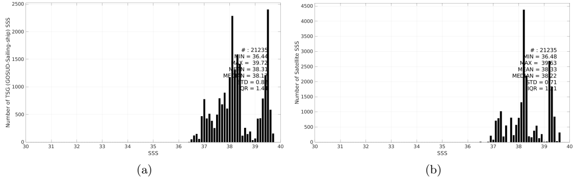
Figure 3: Histograms of SSS from TSG (GOSUD-Sailing-ship) (a) and CCI SSS L4 Merged-OI v4.41 - 30-day running (ESA) (b) considering all match-up pairs per bins of 0.1 over the Mediterranean Sea Pi-MEP region and for the full satellite product period.
