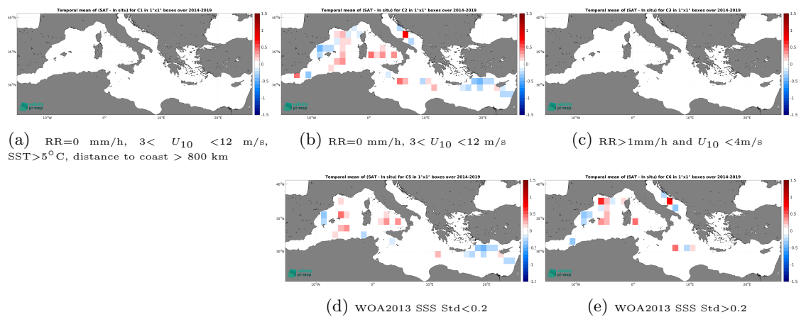
Figure 14: Temporal mean gridded over spatial boxes of size 1^\circ \times 1^\circ of \Delta SSS (CCI SSS L4 Merged-OI v4.41 - 30-day running (ESA) - TSG (GOSUD-Sailing-ship)) for 5 different subdatasets corresponding to:RR=0 mm/h, 3 < U_{10} < 12 m/s, SST >5^\circ C, distance to coast > 800 km (a), RR=0 mm/h, 3 < U_{10} < 12 m/s (b), RR >1 mm/h and U_{10} < 4 m/s (c), WOA2013 SSS Std <0.2 (d), WOA2013 SSS Std >0.2 (e).
