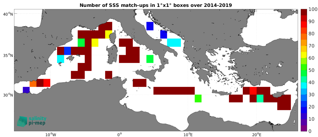
Figure 5: Number of SSS match-ups between TSG (GOSUD-Sailing-ship) SSS and the CCI SSS L4 Merged-OI v4.41 - 30-day running (ESA) SSS product for the Mediterranean Sea Pi-MEP region over 1^\circ \times 1^\circ boxes and for the full satellite product period.
