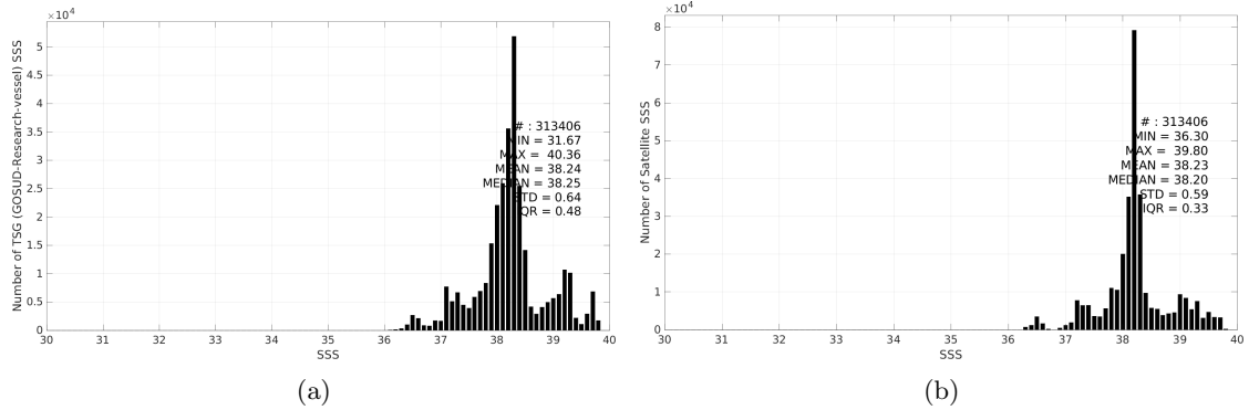
Figure 3: Histograms of SSS from TSG (GOSUD-Research-vessel) (a) and CCI SSS L4 Merged-OI v4.41 - 30-day running (ESA) (b) considering all match-up pairs per bins of 0.1 over the Mediterranean Sea Pi-MEP region and for the full satellite product period.
