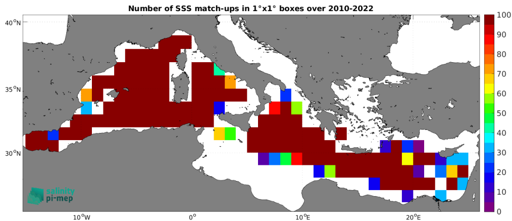
Figure 5: Number of SSS match-ups between TSG (GOSUD-Research-vessel) SSS and the CCI SSS L4 Merged-OI v4.41 - 30-day running (ESA) SSS product for the Mediterranean Sea Pi-MEP region over 1^\circ \times 1^\circ boxes and for the full satellite product period.
