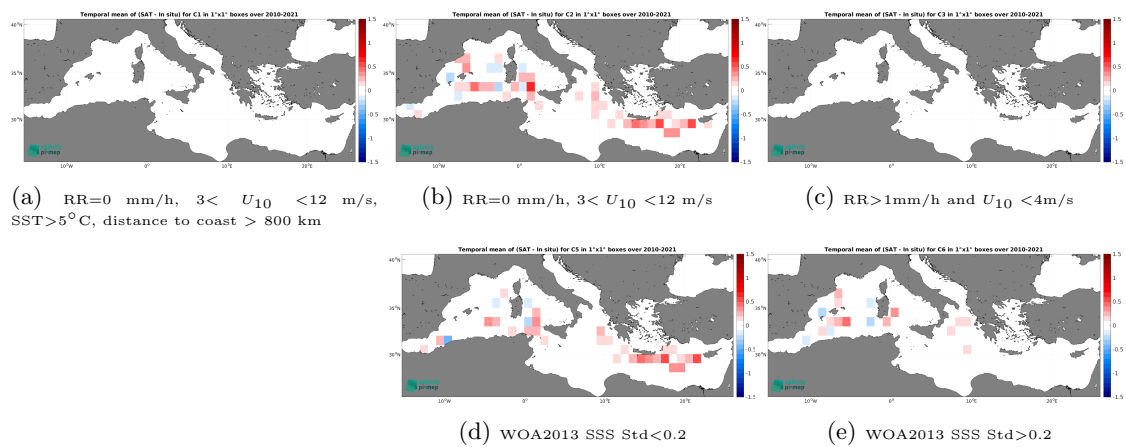
Figure 14: Temporal mean gridded over spatial boxes of size 1^\circ \times 1^\circ of \Delta SSS (CCI SSS L4 Merged-OI v4.41 - 30-day running (ESA) - TSG (CSIC-UTM)) for 5 different subdatasets corresponding to:RR=0 mm/h, 3 < U_{10} < 12 m/s, SST >5^\circ\text{C} , distance to coast > 800 km (a), RR=0 mm/h, 3 < U_{10} < 12 m/s (b), RR >1 mm/h and U_{10} < 4 m/s (c), WOA2013 SSS Std <0.2 (d), WOA2013 SSS Std >0.2 (e).
