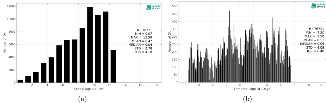
Figure 6: Histograms of the spatial (a) and temporal (b) lags between the location/time of the TSG (CSIC-UTM) measurement and the date of the corresponding CCI SSS L4 Merged-OI v4.41 - 30-day running (ESA) SSS pixel.
