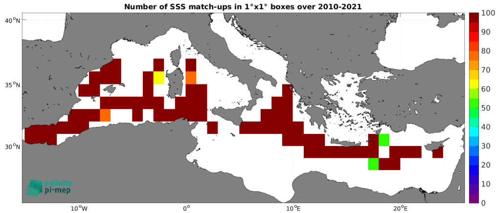
Figure 5: Number of SSS match-ups between TSG (CSIC-UTM) SSS and the CCI SSS L4 Merged-OI v4.41 - 30-day running (ESA) SSS product for the Mediterranean Sea Pi-MEP region over 1^\circ \times 1^\circ boxes and for the full satellite product period.
