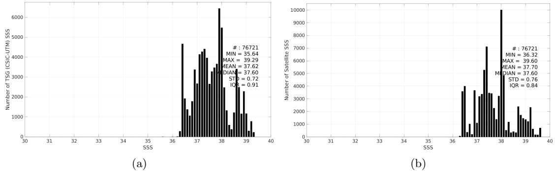
Figure 3: Histograms of SSS from TSG (CSIC-UTM) (a) and CCI SSS L4 Merged-OI v4.41 - 30-day running (ESA) (b) considering all match-up pairs per bins of 0.1 over the Mediterranean Sea Pi-MEP region and for the full satellite product period.
