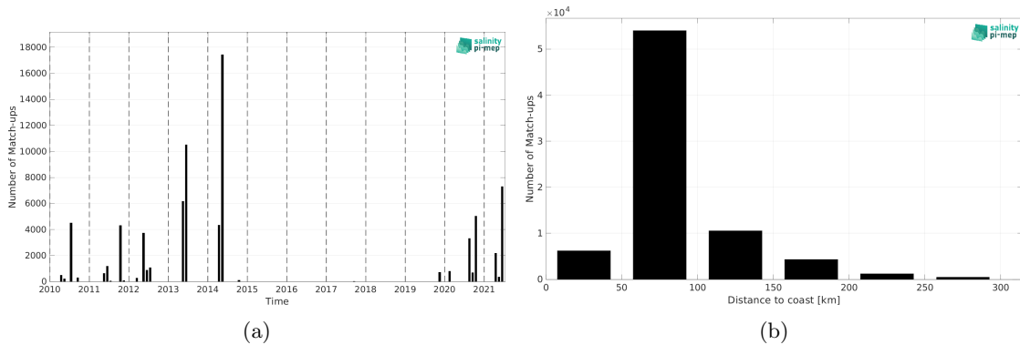
Figure 2: Number of match-ups between TSG (CSIC-UTM) and CCI SSS L4 Merged-OI v4.41 - 30-day running (ESA) SSS as a function of time (a) and as function of the distance to coast (b) over the Mediterranean Sea Pi-MEP region and for the full satellite product period.
