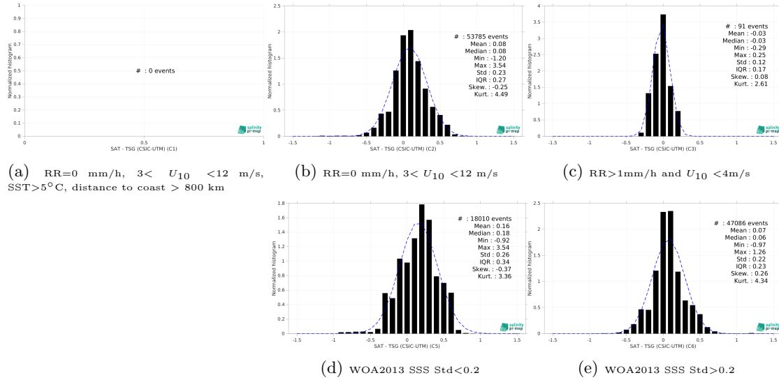
Figure 15: Normalized histogram of \Delta SSS (CCI SSS L4 Merged-OI v4.41 - 30-day running (ESA) - TSG (CSIC-UTM)) for 5 different subdatasets corresponding to: RR=0 mm/h, 3 < U_{10} < 12 m/s, SST > 5°C, distance to coast > 800 km (a), RR=0 mm/h, 3 < U_{10} < 12 m/s (b), RR > 1mm/h and U_{10} < 4 m/s (c), WOA2013 SSS Std < 0.2 (d), WOA2013 SSS Std > 0.2 (e).
