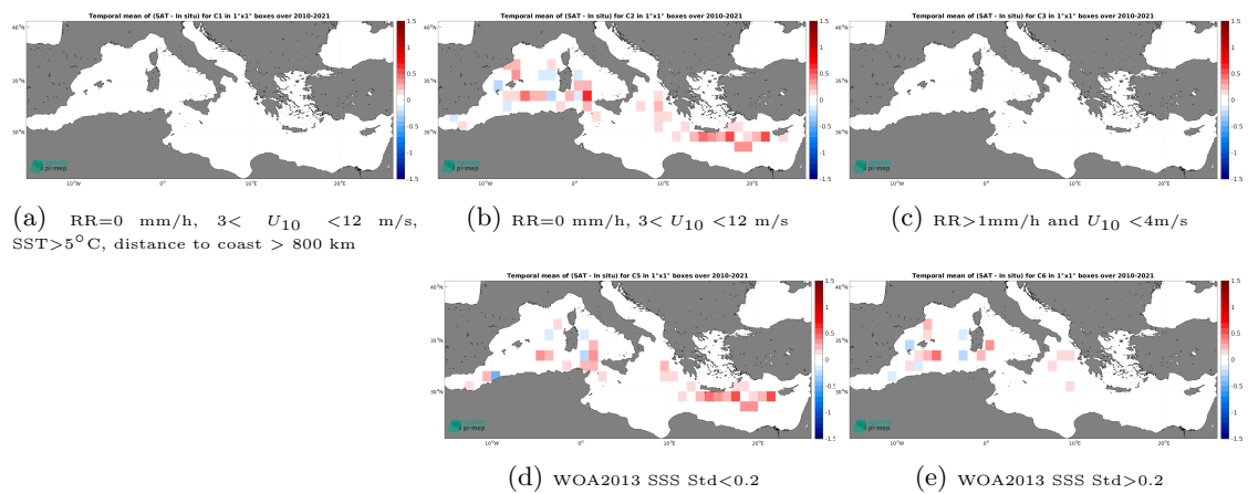
Figure 14: Temporal mean gridded over spatial boxes of size 1^\circ \times 1^\circ of \Delta SSS (CCI SSS L4 Merged-OI v4.41 - 30-day running (ESA) - TSG (CSIC-UTM)) for 5 different subdatasets corresponding to:RR=0 mm/h, 3 < U_{10} < 12 m/s, SST >5^\circ\text{C} , distance to coast > 800 km (a), RR=0 mm/h, 3 < U_{10} < 12 m/s (b), RR >1 mm/h and U_{10} < 4 m/s (c), WOA2013 SSS Std <0.2 (d), WOA2013 SSS Std >0.2 (e).
