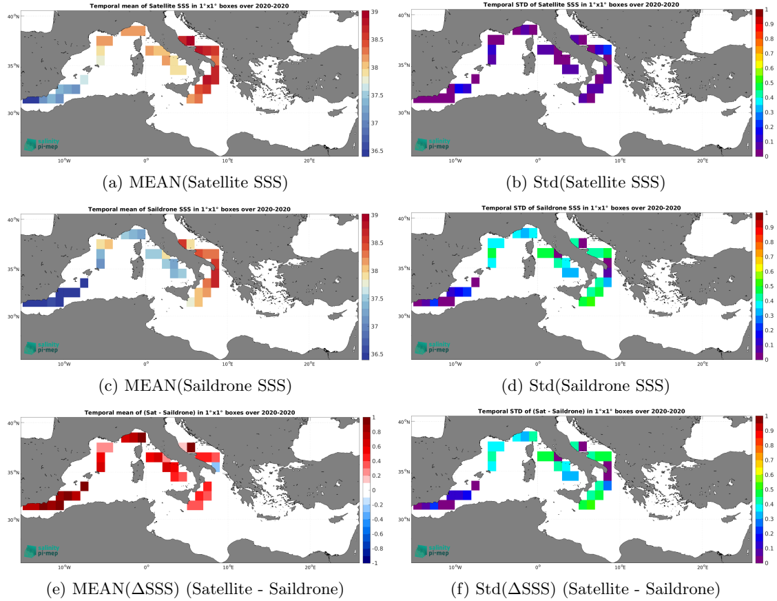
Figure 7: Temporal mean (left) and Std (right) of SSS from CCI SSS L4 Merged-OI v4.41 - 30-day running (ESA) (top), Saildrone (middle), and of \Delta SSS (Satellite - Saildrone). Only match-up pairs are used to generate these maps.
