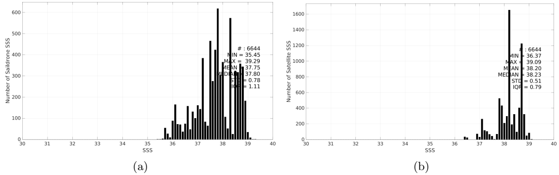
Figure 3: Histograms of SSS from Saildrone (a) and CCI SSS L4 Merged-OI v4.41 - 30-day running (ESA) (b) considering all match-up pairs per bins of 0.1 over the Mediterranean Sea Pi-MEP region and for the full satellite product period.
