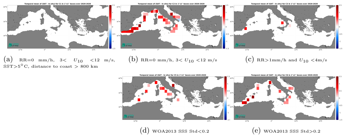
Figure 14: Temporal mean gridded over spatial boxes of size 1^\circ \times 1^\circ of \Delta SSS (CCI SSS L4 Merged-OI v4.41 - 30-day running (ESA) - Saildrone) for 5 different subdatasets corresponding to:RR=0 mm/h, 3 < U_{10} < 12 m/s, SST >5^\circ\text{C} , distance to coast > 800 km (a), RR=0 mm/h, 3 < U_{10} < 12 m/s (b), RR >1 mm/h and U_{10} < 4 m/s (c), WOA2013 SSS Std <0.2 (d), WOA2013 SSS Std >0.2 (e).
