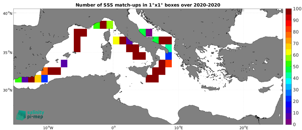
Figure 5: Number of SSS match-ups between Saildrone SSS and the CCI SSS L4 Merged-OI v4.41 - 30-day running (ESA) SSS product for the Mediterranean Sea Pi-MEP region over 1^\circ \times 1^\circ boxes and for the full satellite product period.
