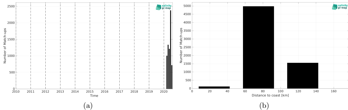
Figure 2: Number of match-ups between Saildrone and CCI SSS L4 Merged-OI v4.41 - 30-day running (ESA) SSS as a function of time (a) and as function of the distance to coast (b) over the Mediterranean Sea Pi-MEP region and for the full satellite product period.
