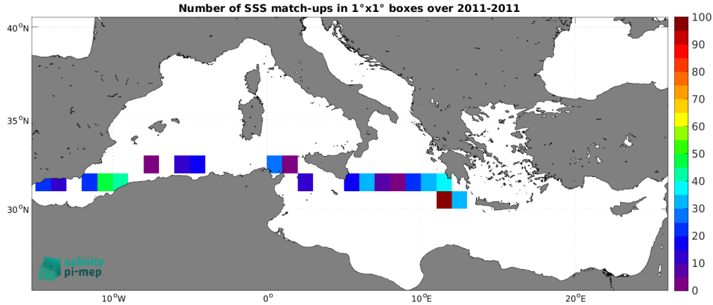
Figure 4: Number of SSS match-ups between TSG (SAMOS) SSS and the CCI SSS L4 Merged-OI v4.4 - 7-day running (ESA) SSS product for the Mediterranean Sea Pi-MEP region over 1^\circ \times 1^\circ boxes and for the full satellite product period.
