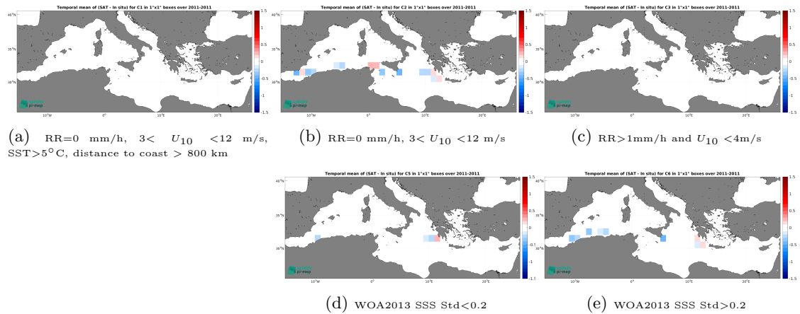
Figure 12: Temporal mean gridded over spatial boxes of size 1^{\circ}\times 1^{\circ} of \Delta\text{SSS} (CCI SSS L4 Merged-OI v4.4 - 7-day running (ESA) - TSG (SAMOS)) for 5 different subdatasets corresponding to:RR=0 mm/h, 3 < U_{10} < 12 m/s, SST > 5^{\circ}\text{C} , distance to coast > 800 km (a), RR=0 mm/h, 3 < U_{10} < 12 m/s (b), RR > 1 mm/h and U_{10} < 4 m/s (c), WOA2013 SSS Std < 0.2 (d), WOA2013 SSS Std > 0.2 (e).
