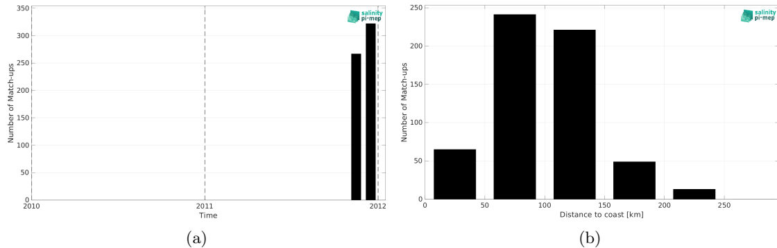
Figure 1: Number of match-ups between TSG (SAMOS) and CCI SSS L4 Merged-OI v4.4 - 7-day running (ESA) SSS as a function of time (a) and as function of the distance to coast (b) over the Mediterranean Sea Pi-MEP region and for the full satellite product period.
