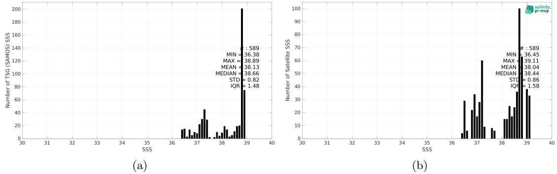
Figure 2: Histograms of SSS from TSG (SAMOS) (a) and CCI SSS L4 Merged-OI v4.4 - 7-day running (ESA) (b) considering all match-up pairs per bins of 0.1 over the Mediterranean Sea Pi-MEP region and for the full satellite product period.
