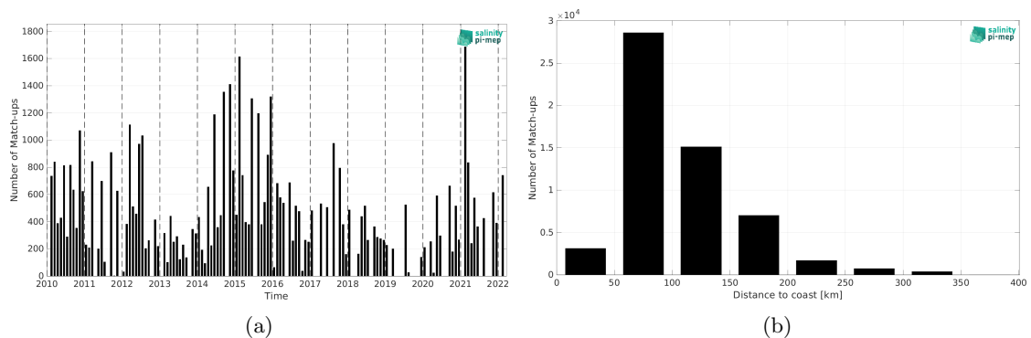
Figure 1: Number of match-ups between TSG (LEGOS-DM) and CCI SSS L4 Merged-OI v4.4 - 7-day running (ESA) SSS as a function of time (a) and as function of the distance to coast (b) over the Mediterranean Sea Pi-MEP region and for the full satellite product period.
