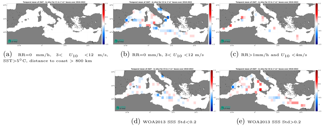
Figure 12: Temporal mean gridded over spatial boxes of size 1^{\circ}\times 1^{\circ} of \Delta\text{SSS} (CCI SSS L4 Merged-OI v4.4 - 7-day running (ESA) - TSG (LEGOS-DM)) for 5 different subdatasets corresponding to:RR=0 mm/h, 3 < U_{10} < 12 m/s, SST >5^{\circ}\text{C} , distance to coast > 800 km (a), RR=0 mm/h, 3 < U_{10} < 12 m/s (b), RR >1 mm/h and U_{10} < 4 m/s (c), WOA2013 SSS Std <0.2 (d), WOA2013 SSS Std >0.2 (e).
