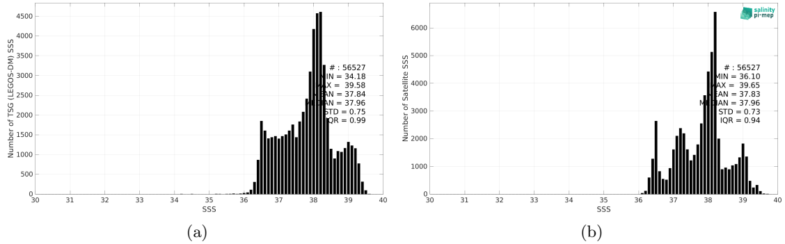
Figure 2: Histograms of SSS from TSG (LEGOS-DM) (a) and CCI SSS L4 Merged-OI v4.4 - 7-day running (ESA) (b) considering all match-up pairs per bins of 0.1 over the Mediterranean Sea Pi-MEP region and for the full satellite product period.
