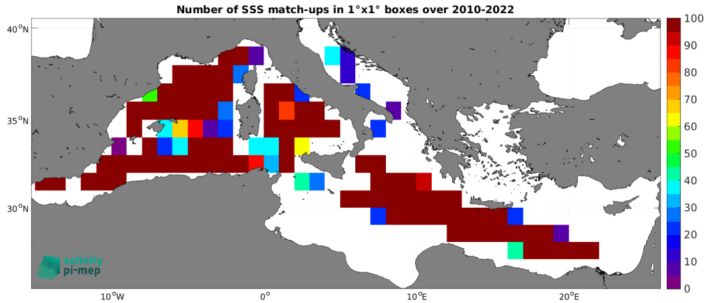
Figure 4: Number of SSS match-ups between TSG (LEGOS-DM) SSS and the CCI SSS L4 Merged-OI v4.4 - 7-day running (ESA) SSS product for the Mediterranean Sea Pi-MEP region over 1^\circ \times 1^\circ boxes and for the full satellite product period.
