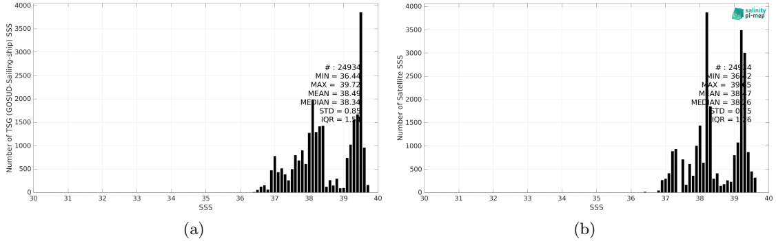
Figure 2: Histograms of SSS from TSG (GOSUD-Sailing-ship) (a) and CCI SSS L4 Merged-OI v4.4 - 7-day running (ESA) (b) considering all match-up pairs per bins of 0.1 over the Mediterranean Sea Pi-MEP region and for the full satellite product period.
