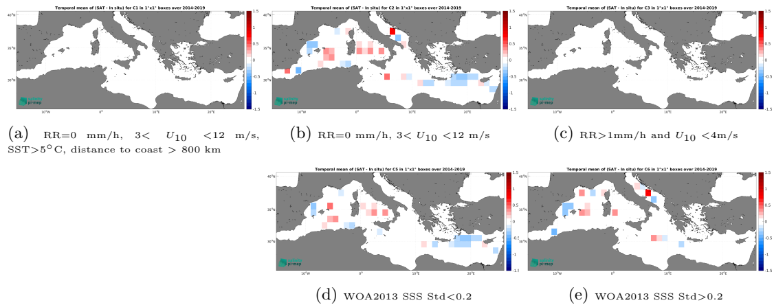
Figure 12: Temporal mean gridded over spatial boxes of size 1^{\circ}\times 1^{\circ} of \Delta SSS (CCI SSS L4 Merged-OI v4.4 - 7-day running (ESA) - TSG (GOSUD-Sailing-ship)) for 5 different subdatasets corresponding to:RR=0 mm/h, 3 < U_{10} < 12 m/s, SST >5^{\circ}\text{C} , distance to coast > 800 km (a), RR=0 mm/h, 3 < U_{10} < 12 m/s (b), RR >1 mm/h and U_{10} < 4 m/s (c), WOA2013 SSS Std <0.2 (d), WOA2013 SSS Std >0.2 (e).
