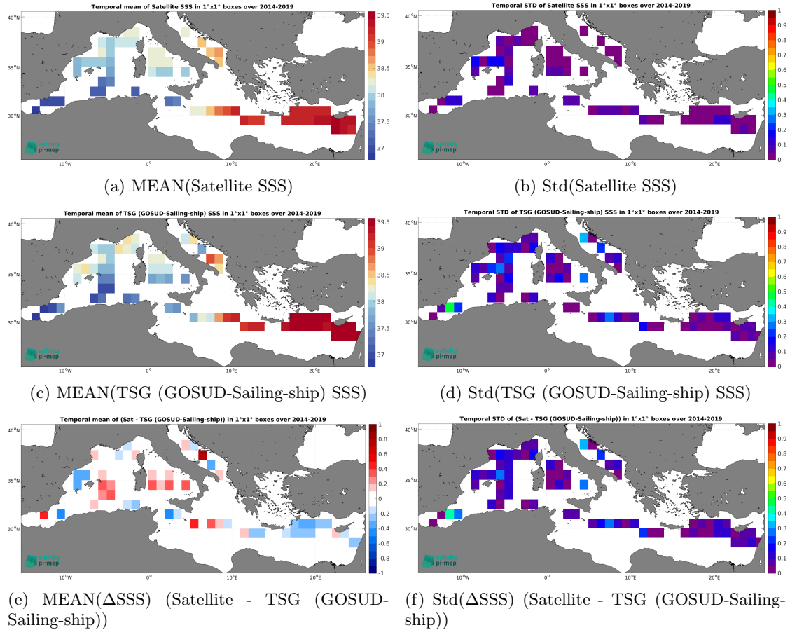
Figure 6: Temporal mean (left) and Std (right) of SSS from CCI SSS L4 Merged-OI v4.4 - 7-day running (ESA) (top), TSG (GOSUD-Sailing-ship) (middle), and of \Delta\text{SSS} (Satellite - TSG (GOSUD-Sailing-ship)). Only match-up pairs are used to generate these maps.
