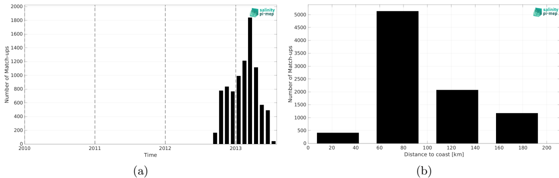
Figure 1: Number of match-ups between Surface drifters and CCI SSS L4 Merged-OI v4.4 - 7-day running (ESA) SSS as a function of time (a) and as function of the distance to coast (b) over the Mediterranean Sea Pi-MEP region and for the full satellite product period.
