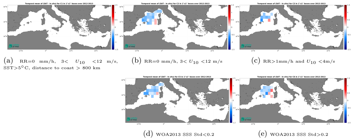
Figure 11: Temporal mean gridded over spatial boxes of size 1^\circ \times 1^\circ of \Delta SSS (CCI SSS L4 Merged-OI v4.4 - 7-day running (ESA) - Surface drifters) for 5 different subdatasets corresponding to:RR=0 mm/h, 3 < U_{10} < 12 m/s, SST >5^\circ\text{C} , distance to coast > 800 km (a), RR=0 mm/h, 3 < U_{10} < 12 m/s (b), RR >1 mm/h and U_{10} < 4 m/s (c), WOA2013 SSS Std <0.2 (d), WOA2013 SSS Std >0.2 (e).
