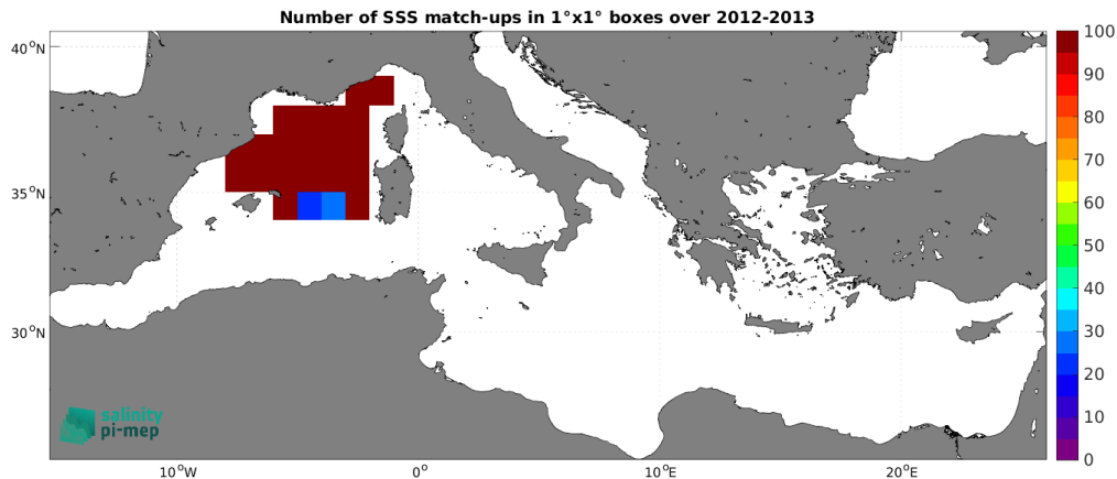
Figure 3: Number of SSS match-ups between Surface drifters SSS and the CCI SSS L4 Merged-OI v4.4 - 7-day running (ESA) SSS product for the Mediterranean Sea Pi-MEP region over 1^\circ \times 1^\circ boxes and for the full satellite product period.
