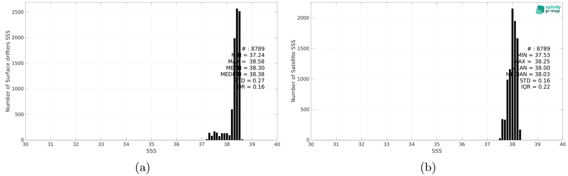
Figure 2: Histograms of SSS from Surface drifters (a) and CCI SSS L4 Merged-OI v4.4 - 7-day running (ESA) (b) considering all match-up pairs per bins of 0.1 over the Mediterranean Sea Pi-MEP region and for the full satellite product period.
