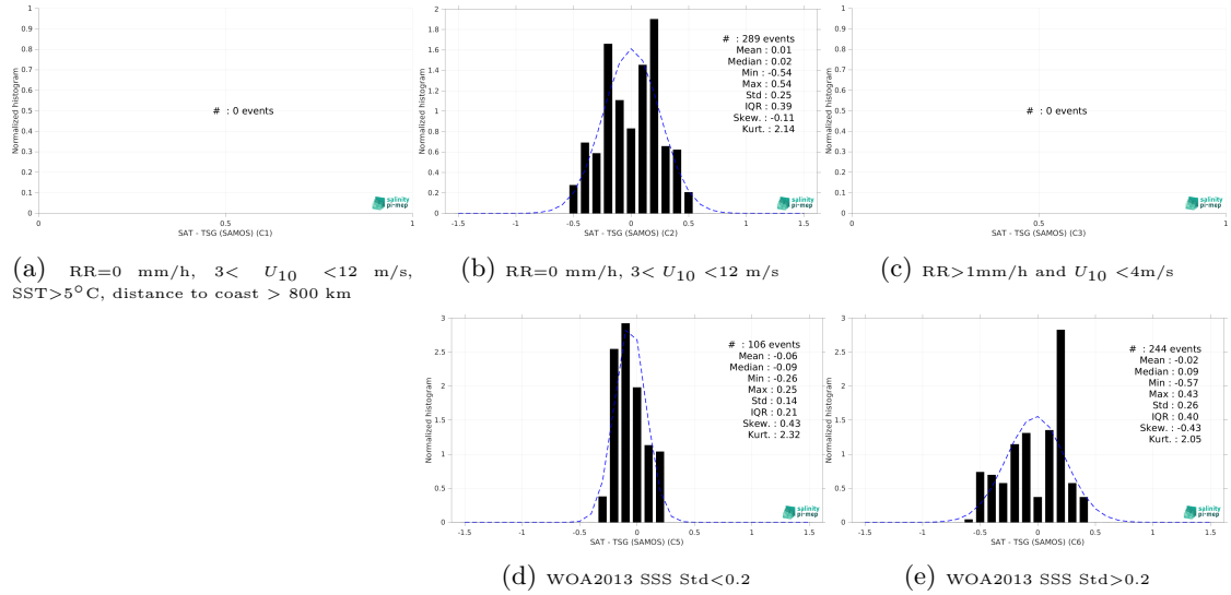
Figure 13: Normalized histogram of \Delta SSS (CCI SSS L4 Merged-OI v4.4 - 30-day running (ESA) - TSG (SAMOS)) for 5 different subdatasets corresponding to: RR=0 mm/h, 3 < U_{10} < 12 m/s, SST > 5°C, distance to coast > 800 km (a), RR=0 mm/h, 3 < U_{10} < 12 m/s (b), RR > 1mm/h and U_{10} < 4 m/s (c), WOA2013 SSS Std < 0.2 (d), WOA2013 SSS Std > 0.2 (e).
