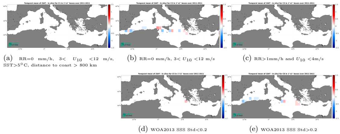
Figure 12: Temporal mean gridded over spatial boxes of size 1^{\circ}\times 1^{\circ} of \Delta\text{SSS} (CCI SSS L4 Merged-OI v4.4 - 30-day running (ESA) - TSG (SAMOS)) for 5 different subdatasets corresponding to:RR=0 mm/h, 3 < U_{10} < 12 m/s, SST > 5^{\circ}\text{C} , distance to coast > 800 km (a), RR=0 mm/h, 3 < U_{10} < 12 m/s (b), RR > 1 mm/h and U_{10} < 4 m/s (c), WOA2013 SSS Std < 0.2 (d), WOA2013 SSS Std > 0.2 (e).
