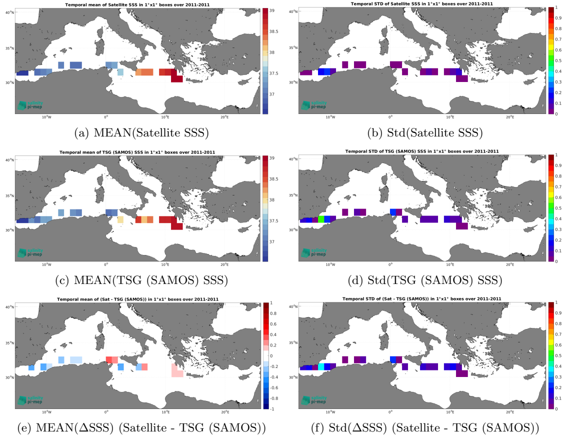
Figure 6: Temporal mean (left) and Std (right) of SSS from CCI SSS L4 Merged-OI v4.4 - 30-day running (ESA) (top), TSG (SAMOS) (middle), and of \Delta\text{SSS} (Satellite - TSG (SAMOS)). Only match-up pairs are used to generate these maps.
