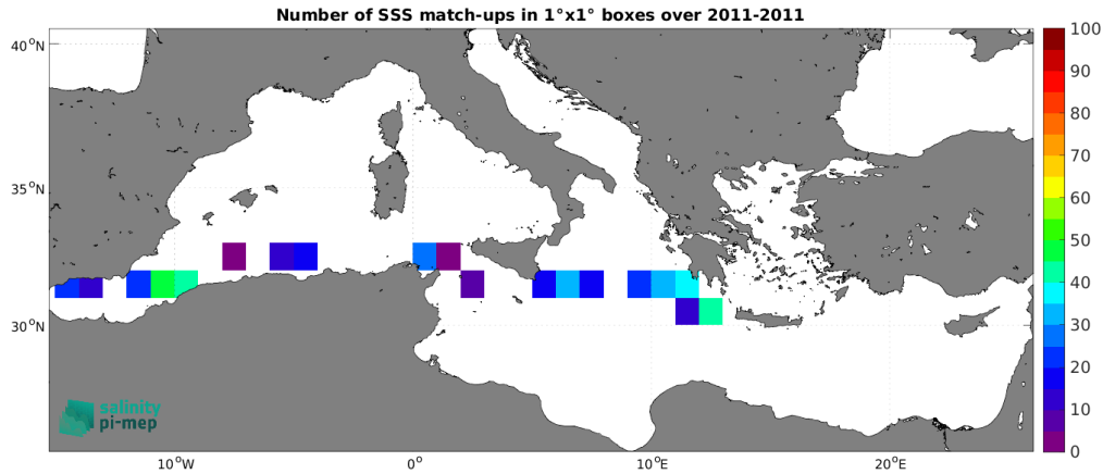
Figure 4: Number of SSS match-ups between TSG (SAMOS) SSS and the CCI SSS L4 Merged-OI v4.4 - 30-day running (ESA) SSS product for the Mediterranean Sea Pi-MEP region over 1^\circ \times 1^\circ boxes and for the full satellite product period.
