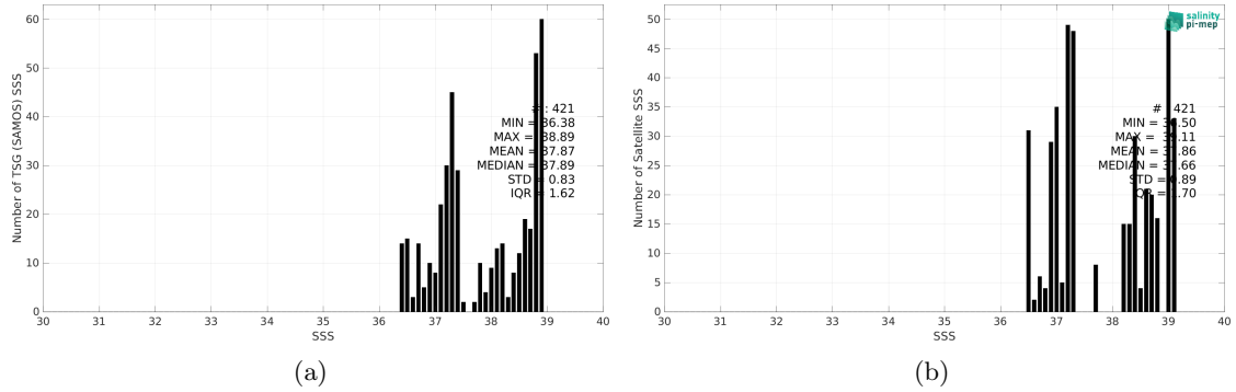
Figure 2: Histograms of SSS from TSG (SAMOS) (a) and CCI SSS L4 Merged-OI v4.4 - 30-day running (ESA) (b) considering all match-up pairs per bins of 0.1 over the Mediterranean Sea Pi-MEP region and for the full satellite product period.
