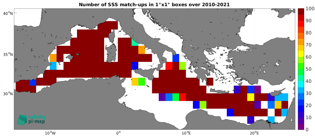
Figure 4: Number of SSS match-ups between TSG (GOSUD-Research-vessel) SSS and the CCI SSS L4 Merged-OI v4.4 - 30-day running (ESA) SSS product for the Mediterranean Sea Pi-MEP region over 1^\circ \times 1^\circ boxes and for the full satellite product period.
