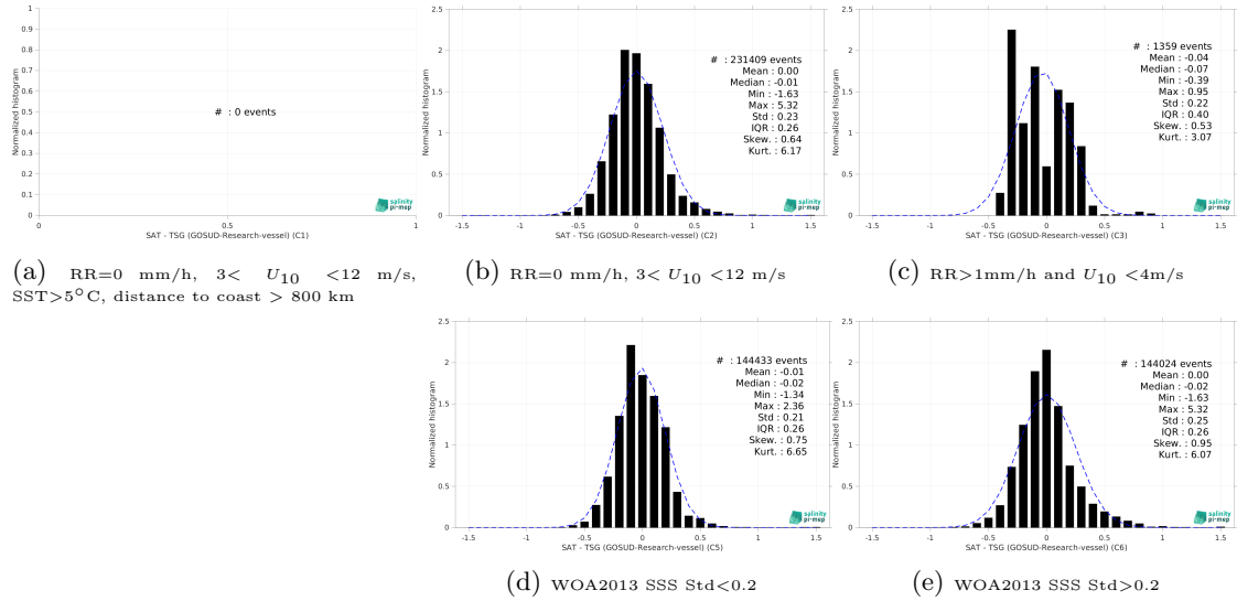
Figure 13: Normalized histogram of \Delta SSS (CCI SSS L4 Merged-OI v4.4 - 30-day running (ESA) - TSG (GOSUD-Research-vessel)) for 5 different subdatasets corresponding to: RR=0 mm/h, 3 < U_{10} < 12 m/s, SST>5°C, distance to coast > 800 km (a), RR=0 mm/h, 3 < U_{10} < 12 m/s (b), RR>1mm/h and U_{10} < 4 m/s (c), WOA2013 SSS Std<0.2 (d), WOA2013 SSS Std>0.2 (e).
