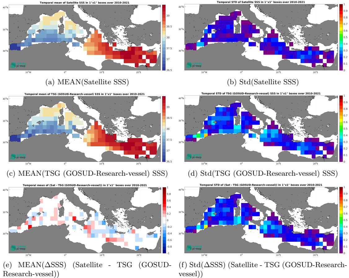
Figure 6: Temporal mean (left) and Std (right) of SSS from CCI SSS L4 Merged-OI v4.4 - 30-day running (ESA) (top), TSG (GOSUD-Research-vessel) (middle), and of \Delta\text{SSS} (Satellite - TSG (GOSUD-Research-vessel)). Only match-up pairs are used to generate these maps.
