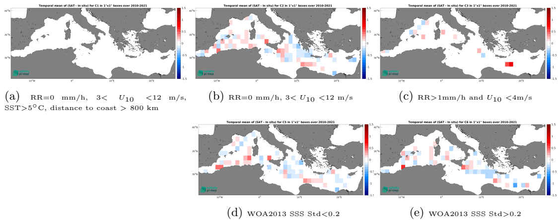
Figure 12: Temporal mean gridded over spatial boxes of size 1^{\circ}\times 1^{\circ} of \Delta SSS (CCI SSS L4 Merged-OI v4.4 - 30-day running (ESA) - TSG (GOSUD-Research-vessel)) for 5 different subdatasets corresponding to:RR=0 mm/h, 3 < U_{10} < 12 m/s, SST >5^{\circ}\text{C} , distance to coast > 800 km (a), RR=0 mm/h, 3 < U_{10} < 12 m/s (b), RR >1 mm/h and U_{10} < 4 m/s (c), WOA2013 SSS Std <0.2 (d), WOA2013 SSS Std >0.2 (e).
