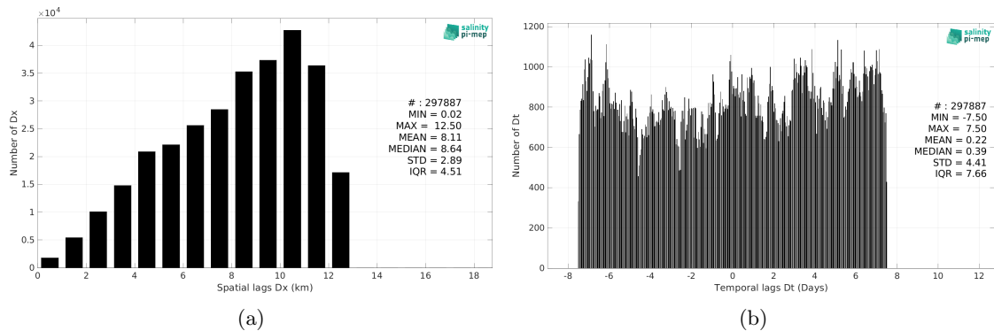
Figure 5: Histograms of the spatial (a) and temporal (b) lags between the location/time of the TSG (GOSUD-Research-vessel) measurement and the date of the corresponding CCI SSS L4 Merged-OI v4.4 - 30-day running (ESA) SSS pixel.
