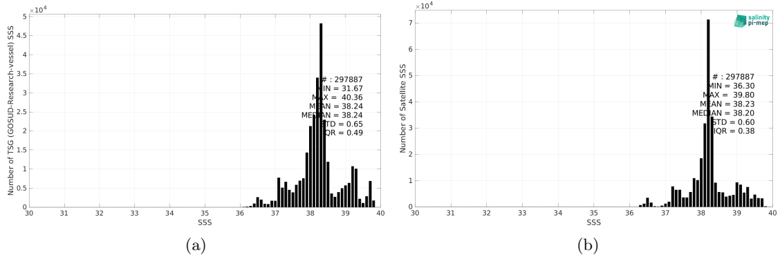
Figure 2: Histograms of SSS from TSG (GOSUD-Research-vessel) (a) and CCI SSS L4 Merged-OI v4.4 - 30-day running (ESA) (b) considering all match-up pairs per bins of 0.1 over the Mediterranean Sea Pi-MEP region and for the full satellite product period.
