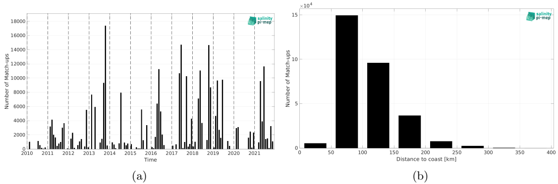
Figure 1: Number of match-ups between TSG (GOSUD-Research-vessel) and CCI SSS L4 Merged-OI v4.4 - 30-day running (ESA) SSS as a function of time (a) and as function of the distance to coast (b) over the Mediterranean Sea Pi-MEP region and for the full satellite product period.
