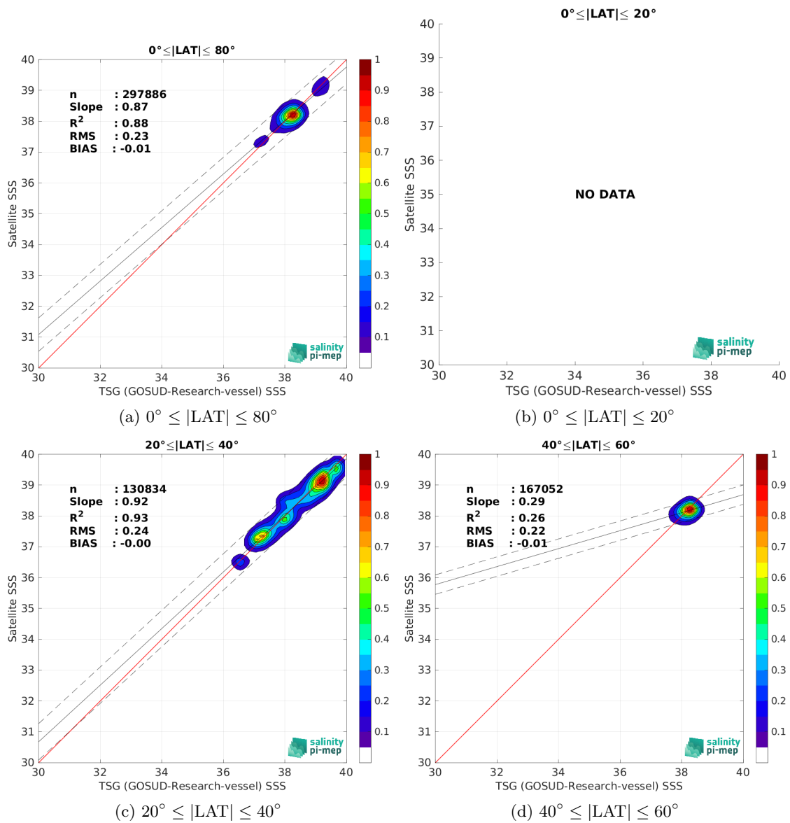
Figure 9: Contour maps of the concentration of CCI SSS L4 Merged-OI v4.4 - 30-day running (ESA) SSS (y-axis) versus TSG (GOSUD-Research-vessel) SSS (x-axis) at match-up pairs for different latitude bands. For each plot, the red line shows x=y . The black thin and dashed lines indicate a linear fit through the data cloud and the \pm 95\% confidence levels, respectively. The number match-up pairs n , the slope and R^2 coefficient of the linear fit, the root mean square (RMS) and the mean bias between satellite and in situ data are indicated for each latitude band in each plots.
