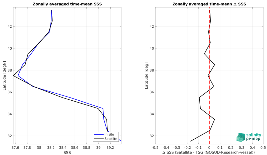
Figure 8: Left panel: Zonal mean SSS from CCI SSS L4 Merged-OI v4.4 - 30-day running (ESA) satellite product (black) and from TSG (GOSUD-Research-vessel) (blue). Right panel: Zonal mean of \Delta SSS (Satellite - TSG (GOSUD-Research-vessel)) for all the collected Pi-MEP match-up pairs estimated over the full satellite product period.
