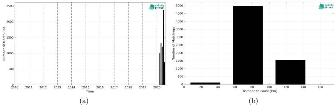
Figure 1: Number of match-ups between Saildrone and CCI SSS L4 Merged-OI v4.4 - 30-day running (ESA) SSS as a function of time (a) and as function of the distance to coast (b) over the Mediterranean Sea Pi-MEP region and for the full satellite product period.
