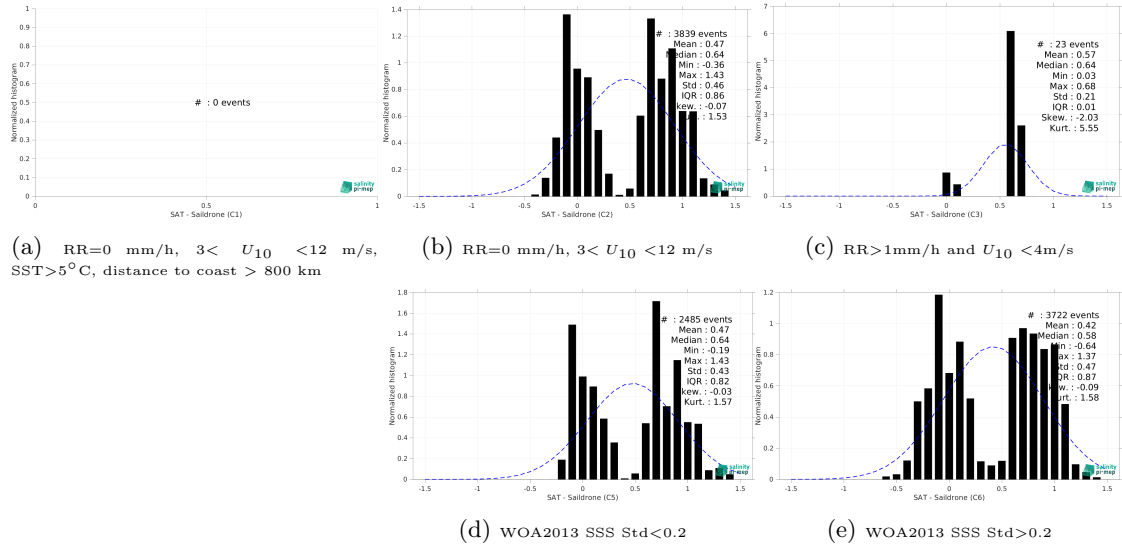
Figure 13: Normalized histogram of \Delta SSS (CCI SSS L4 Merged-OI v4.4 - 30-day running (ESA) - Saildrone) for 5 different subdatasets corresponding to: RR=0 mm/h, 3 < U_{10} < 12 m/s, SST>5°C, distance to coast > 800 km (a), RR=0 mm/h, 3 < U_{10} < 12 m/s (b), RR>1mm/h and U_{10} < 4 m/s (c), WOA2013 SSS Std<0.2 (d), WOA2013 SSS Std>0.2 (e).
