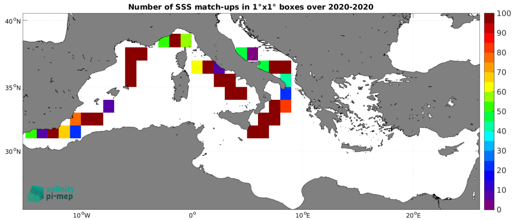
Figure 4: Number of SSS match-ups between Saildrone SSS and the CCI SSS L4 Merged-OI v4.4 - 30-day running (ESA) SSS product for the Mediterranean Sea Pi-MEP region over 1^\circ \times 1^\circ boxes and for the full satellite product period.
