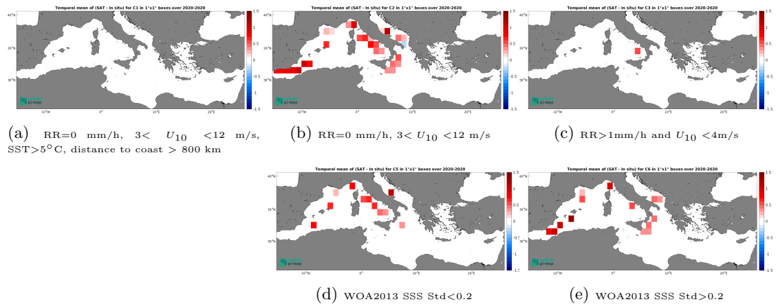
Figure 12: Temporal mean gridded over spatial boxes of size 1^\circ \times 1^\circ of \Delta SSS (CCI SSS L4 Merged-OI v4.4 - 30-day running (ESA) - Saildrone) for 5 different subdatasets corresponding to:RR=0 mm/h, 3 < U_{10} < 12 m/s, SST >5^\circ\text{C} , distance to coast > 800 km (a), RR=0 mm/h, 3 < U_{10} < 12 m/s (b), RR >1 mm/h and U_{10} < 4 m/s (c), WOA2013 SSS Std <0.2 (d), WOA2013 SSS Std >0.2 (e).
