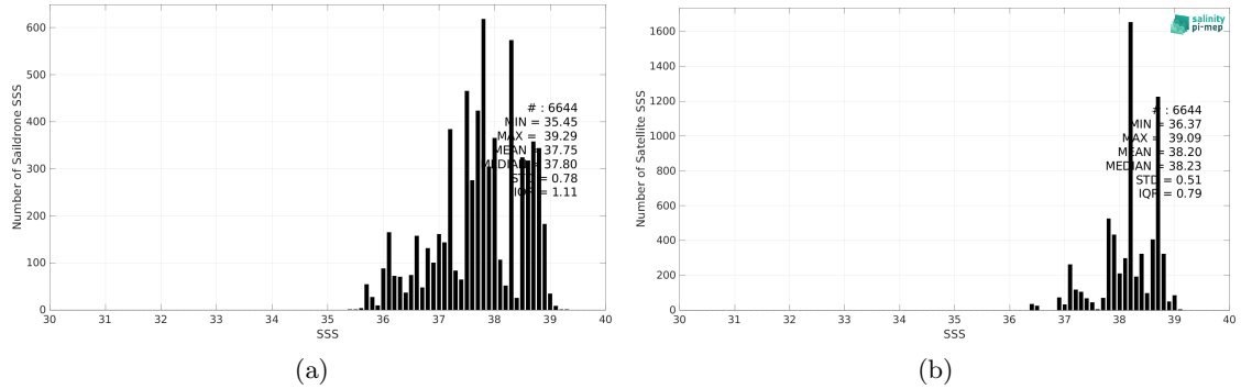
Figure 2: Histograms of SSS from Saildrone (a) and CCI SSS L4 Merged-OI v4.4 - 30-day running (ESA) (b) considering all match-up pairs per bins of 0.1 over the Mediterranean Sea Pi-MEP region and for the full satellite product period.
