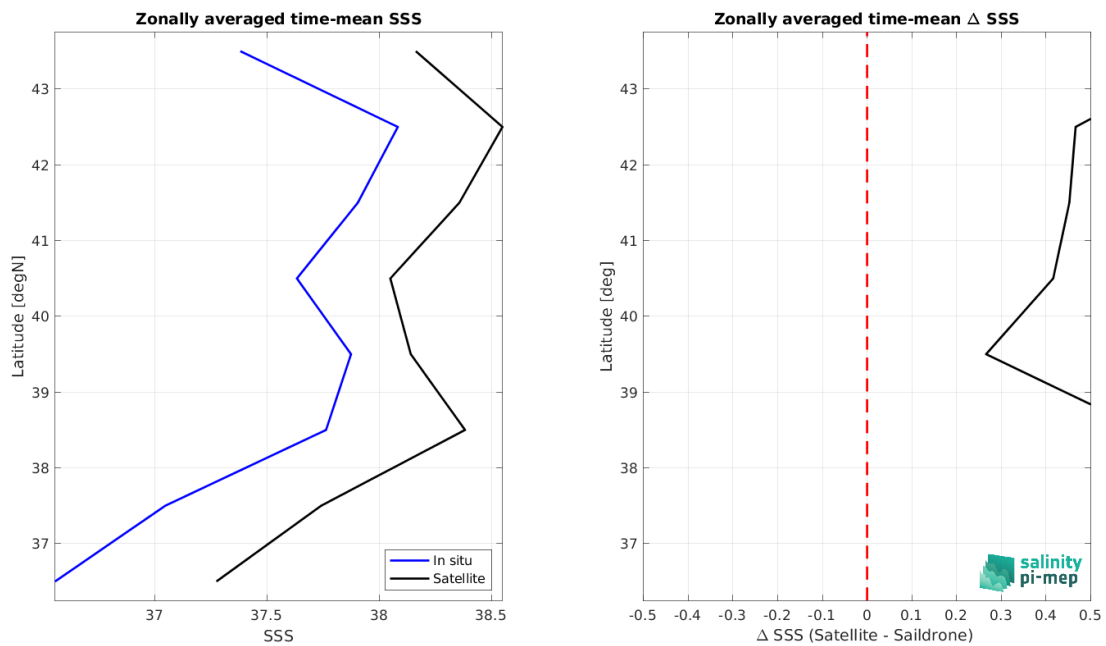
Figure 8: Left panel: Zonal mean SSS from CCI SSS L4 Merged-OI v4.4 - 30-day running (ESA) satellite product (black) and from Saildrone (blue). Right panel: Zonal mean of \Delta SSS (Satellite - Saildrone) for all the collected Pi-MEP match-up pairs estimated over the full satellite product period.
