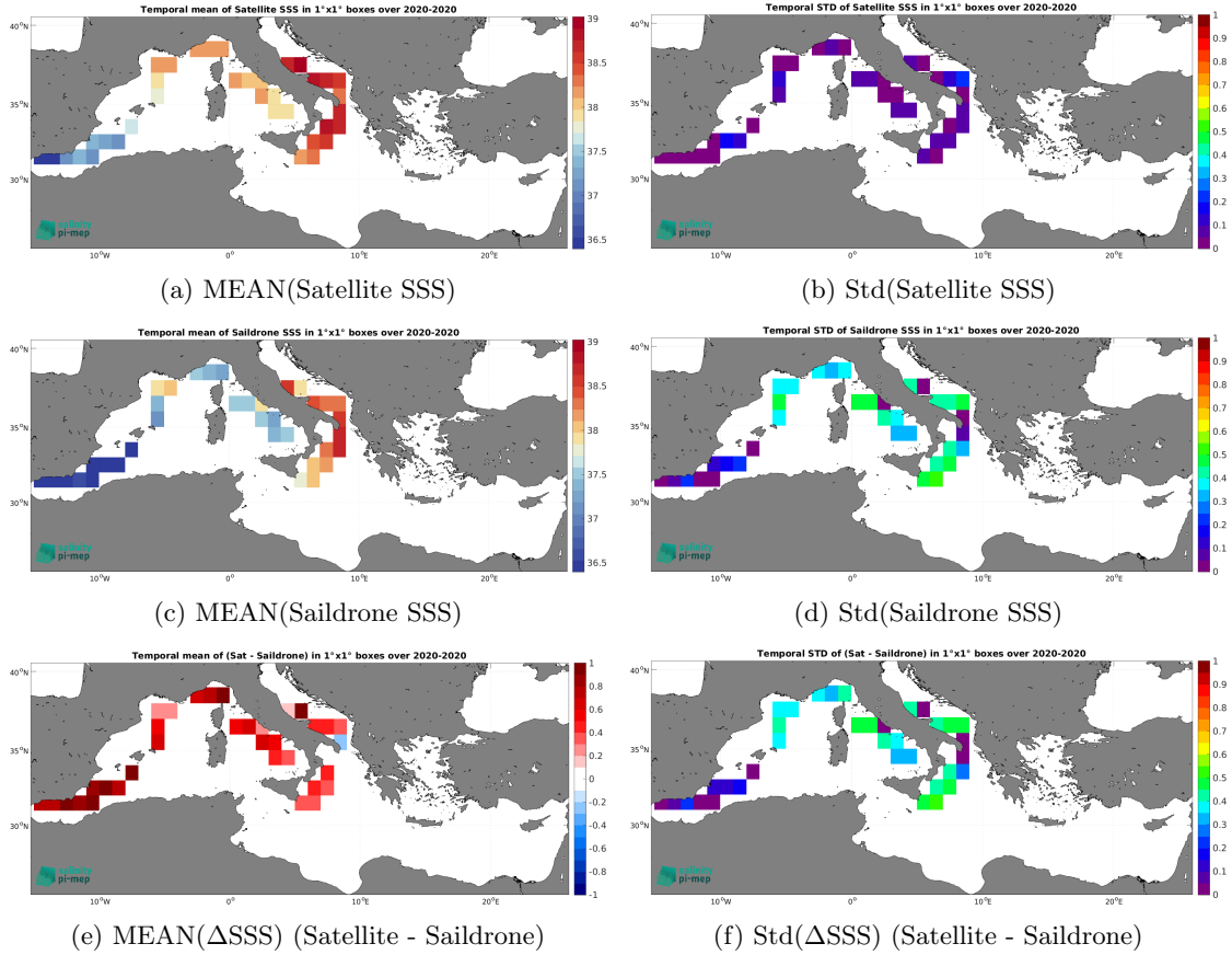
Figure 6: Temporal mean (left) and Std (right) of SSS from CCI SSS L4 Merged-OI v4.4 - 30-day running (ESA) (top), Saildrone (middle), and of \Delta SSS (Satellite - Saildrone). Only match-up pairs are used to generate these maps.
