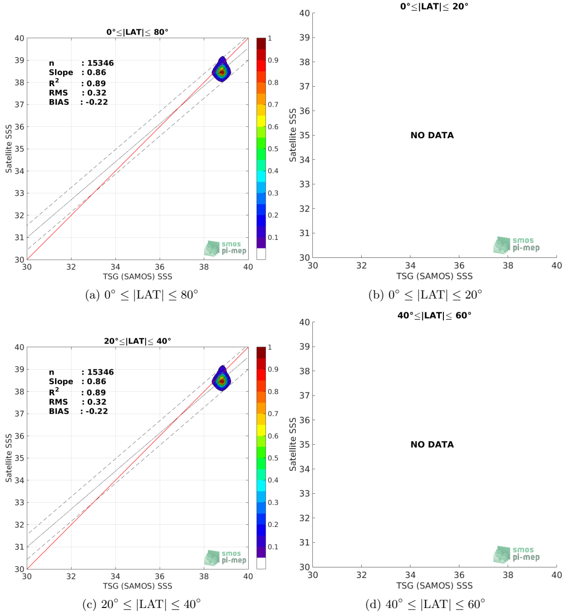
Figure 9: Contour maps of the concentration of CCI SSS L4 Merged-OI v3.2 - 7-day running (ESA) SSS (y-axis) versus TSG (SAMOS) SSS (x-axis) at match-up pairs for different latitude bands. For each plot, the red line shows x=y . The black thin and dashed lines indicate a linear fit through the data cloud and the \pm 95\% confidence levels, respectively. The number match-up pairs n , the slope and R^2 coefficient of the linear fit, the root mean square (RMS) and the mean bias between satellite and in situ data are indicated for each latitude band in each plots.
