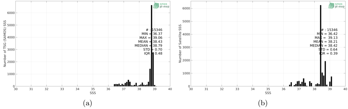
Figure 2: Histograms of SSS from TSG (SAMOS) (a) and CCI SSS L4 Merged-OI v3.2 - 7-day running (ESA) (b) considering all match-up pairs per bins of 0.1 over the Mediterranean Sea Pi-MEP region and for the full satellite product period.
