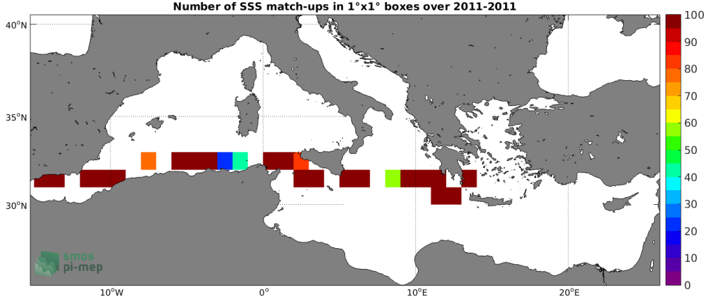
Figure 4: Number of SSS match-ups between TSG (SAMOS) SSS and the CCI SSS L4 Merged-OI v3.2 - 7-day running (ESA) SSS product for the Mediterranean Sea Pi-MEP region over 1^\circ \times 1^\circ boxes and for the full satellite product period.
