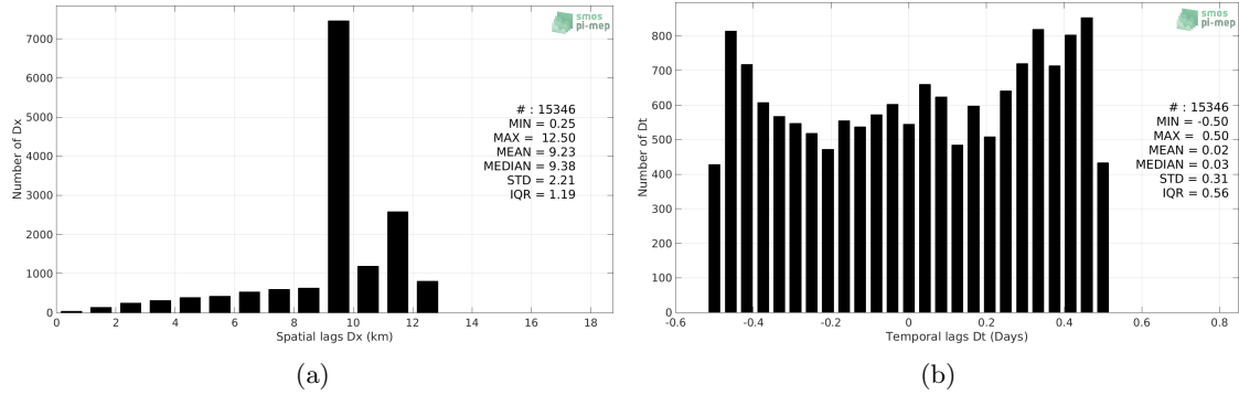
Figure 5: Histograms of the spatial (a) and temporal (b) lags between the location/time of the TSG (SAMOS) measurement and the date of the corresponding CCI SSS L4 Merged-OI v3.2 - 7-day running (ESA) SSS pixel.
