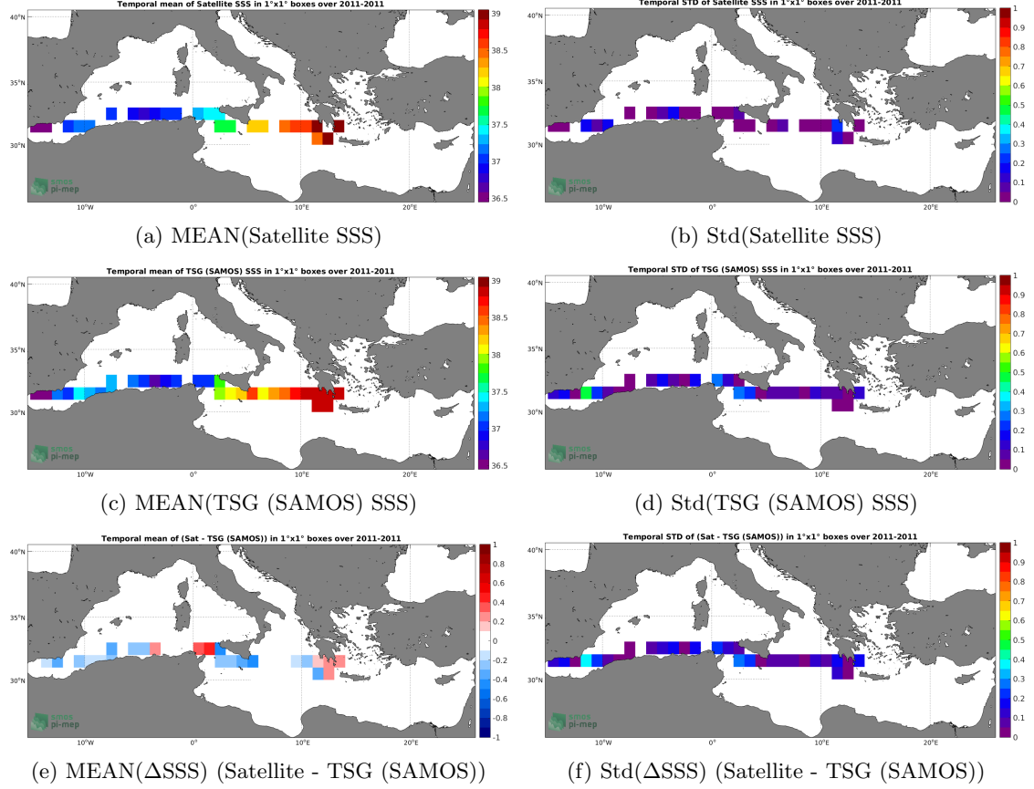
Figure 6: Temporal mean (left) and Std (right) of SSS from CCI SSS L4 Merged-OI v3.2 - 7-day running (ESA) (top), TSG (SAMOS) (middle), and of \Delta\text{SSS} (Satellite - TSG (SAMOS)). Only match-up pairs are used to generate these maps.
