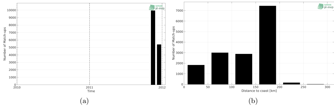
Figure 1: Number of match-ups between TSG (SAMOS) and CCI SSS L4 Merged-OI v3.2 - 7-day running (ESA) SSS as a function of time (a) and as function of the distance to coast (b) over the Mediterranean Sea Pi-MEP region and for the full satellite product period.
