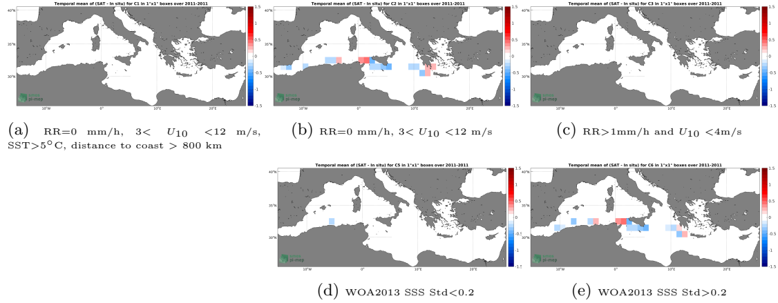
Figure 12: Temporal mean gridded over spatial boxes of size 1^{\circ}\times 1^{\circ} of \Delta\text{SSS} (CCI SSS L4 Merged-OI v3.2 - 7-day running (ESA) - TSG (SAMOS)) for 5 different subdatasets corresponding to: RR=0 mm/h, 3 < U_{10} < 12 m/s, SST >5^{\circ}\text{C} , distance to coast > 800 km (a), RR=0 mm/h, 3 < U_{10} < 12 m/s (b), RR >1 mm/h and U_{10} < 4 m/s (c), WOA2013 SSS Std <0.2 (d), WOA2013 SSS Std >0.2 (e).
