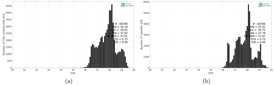
Figure 2: Histograms of SSS from TSG (LEGOS-DM) (a) and CCI SSS L4 Merged-OI v3.2 - 7-day running (ESA) (b) considering all match-up pairs per bins of 0.1 over the Mediterranean Sea Pi-MEP region and for the full satellite product period.
