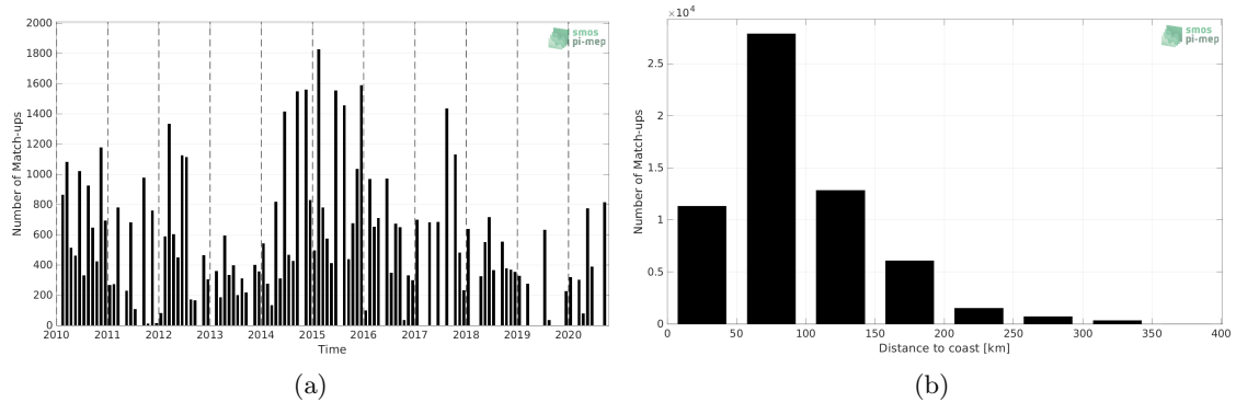
Figure 1: Number of match-ups between TSG (LEGOS-DM) and CCI SSS L4 Merged-OI v3.2 - 7-day running (ESA) SSS as a function of time (a) and as function of the distance to coast (b) over the Mediterranean Sea Pi-MEP region and for the full satellite product period.
