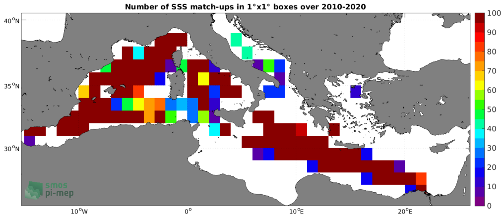
Figure 4: Number of SSS match-ups between TSG (LEGOS-DM) SSS and the CCI SSS L4 Merged-OI v3.2 - 7-day running (ESA) SSS product for the Mediterranean Sea Pi-MEP region over 1^\circ \times 1^\circ boxes and for the full satellite product period.
