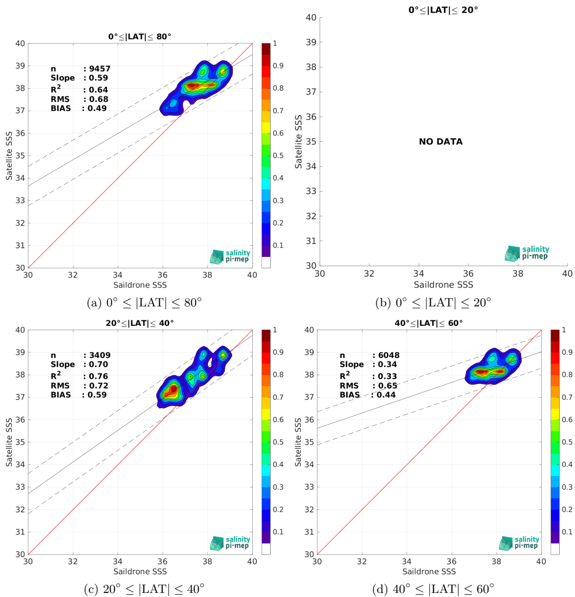
Figure 9: Contour maps of the concentration of CCI SSS L4 Merged-OI v3.2 - 7-day running (ESA) SSS (y-axis) versus Saldrone SSS (x-axis) at match-up pairs for different latitude bands. For each plot, the red line shows x=y . The black thin and dashed lines indicate a linear fit through the data cloud and the \pm 95\% confidence levels, respectively. The number match-up pairs n , the slope and R^2 coefficient of the linear fit, the root mean square (RMS) and the mean bias between satellite and in situ data are indicated for each latitude band in each plots.
