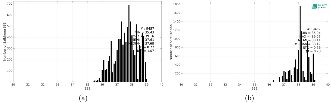
Figure 2: Histograms of SSS from Saildrone (a) and CCI SSS L4 Merged-OI v3.2 - 7-day running (ESA) (b) considering all match-up pairs per bins of 0.1 over the Mediterranean Sea Pi-MEP region and for the full satellite product period.
