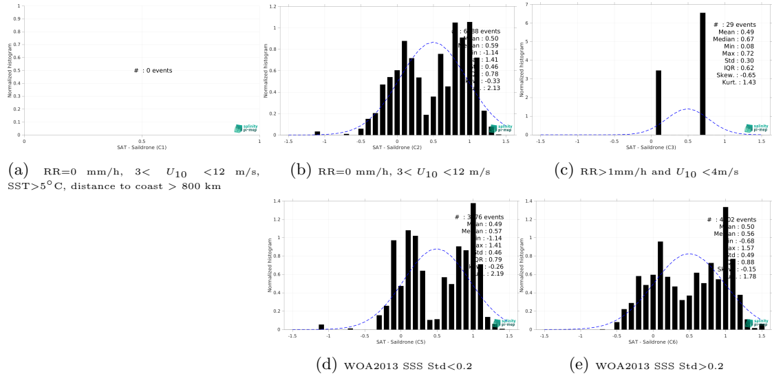
Figure 13: Normalized histogram of \Delta\text{SSS} (CCI SSS L4 Merged-OI v3.2 - 7-day running (ESA) - Sailability) for 5 different subdatasets corresponding to: RR=0 mm/h, 3 < U_{10} < 12 m/s, SST > 5^{\circ}\text{C} , distance to coast > 800 km (a), RR=0 mm/h, 3 < U_{10} < 12 m/s (b), RR > 1\text{mm/h} and U_{10} < 4\text{m/s} (c), WOA2013 SSS Std < 0.2 (d), WOA2013 SSS Std > 0.2 (e).
