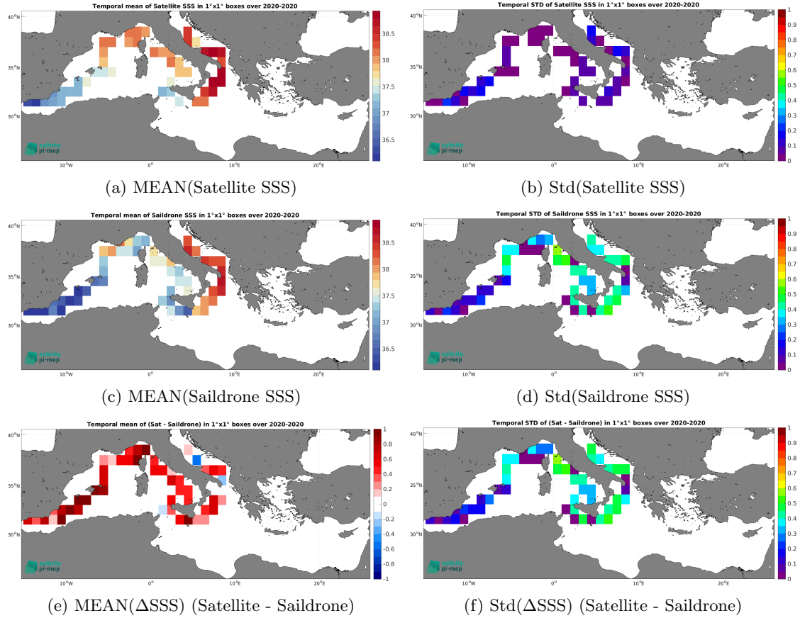
Figure 6: Temporal mean (left) and Std (right) of SSS from CCI SSS L4 Merged-OI v3.2 - 7-day running (ESA) (top), Saildrone (middle), and of \Delta\text{SSS} (Satellite - Saildrone). Only match-up pairs are used to generate these maps.
