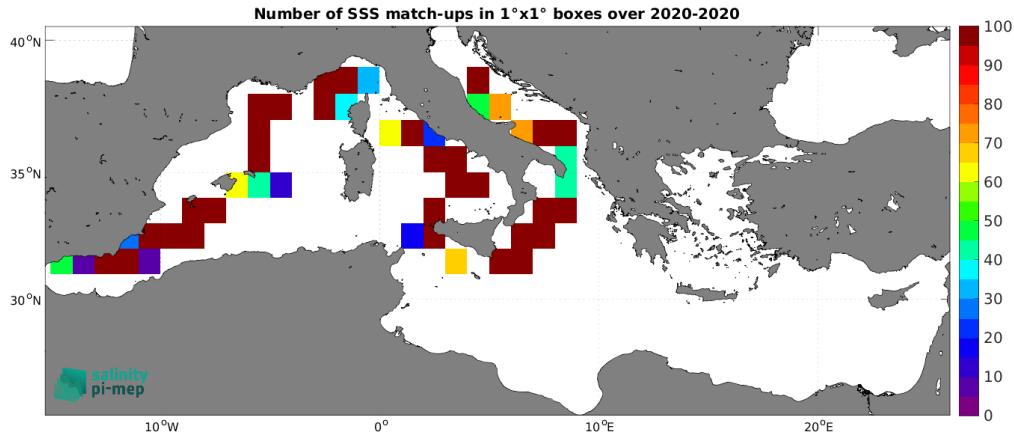
Figure 4: Number of SSS match-ups between Saildrone SSS and the CCI SSS L4 Merged-OI v3.2 - 7-day running (ESA) SSS product for the Mediterranean Sea Pi-MEP region over 1^\circ \times 1^\circ boxes and for the full satellite product period.
