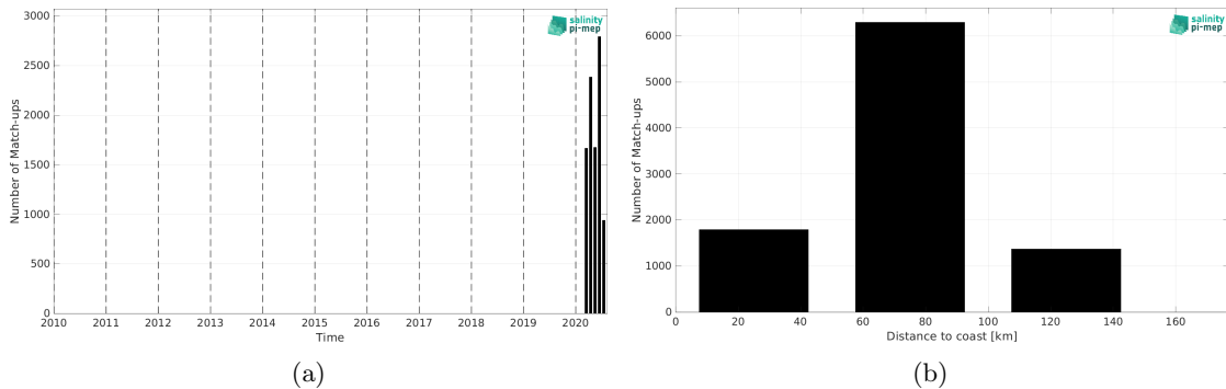
Figure 1: Number of match-ups between Saildrone and CCI SSS L4 Merged-OI v3.2 - 7-day running (ESA) SSS as a function of time (a) and as function of the distance to coast (b) over the Mediterranean Sea Pi-MEP region and for the full satellite product period.
