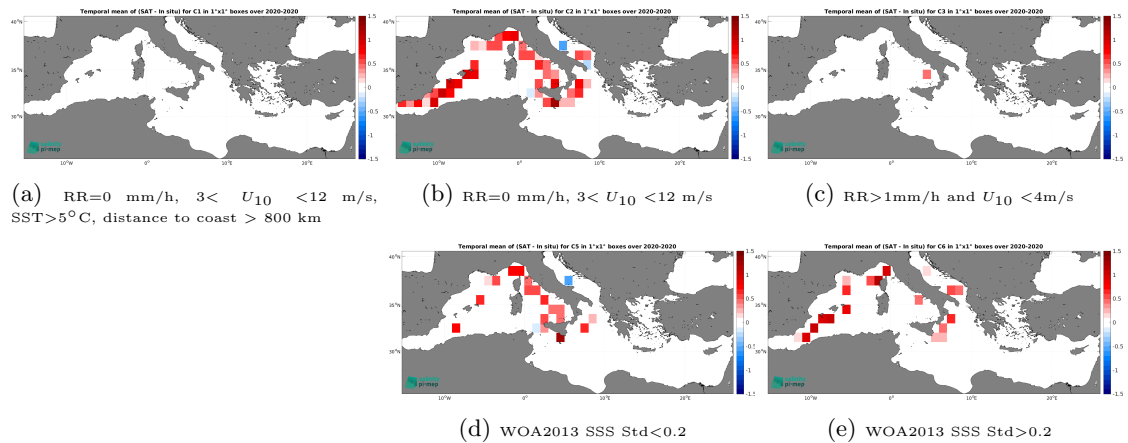
Figure 12: Temporal mean gridded over spatial boxes of size 1^\circ \times 1^\circ of \Delta SSS (CCI SSS L4 Merged-OI v3.2 - 7-day running (ESA) - Saildrone) for 5 different subdatasets corresponding to:RR=0 mm/h, 3 < U_{10} < 12 m/s, SST >5^\circ C, distance to coast > 800 km (a), RR=0 mm/h, 3 < U_{10} < 12 m/s (b), RR >1 mm/h and U_{10} < 4 m/s (c), WOA2013 SSS Std <0.2 (d), WOA2013 SSS Std >0.2 (e).
