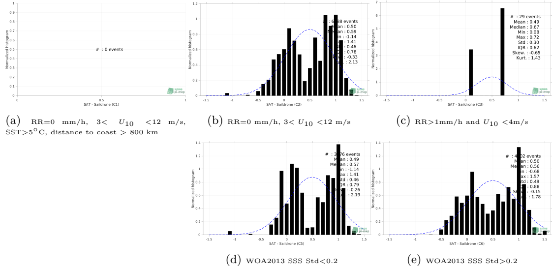
Figure 13: Normalized histogram of \Delta\text{SSS} (CCI SSS L4 Merged-OI v3.2 - 7-day running (ESA) - Saldrone) for 5 different subdatasets corresponding to: RR=0 mm/h, 3 < U_{10} < 12 m/s, SST > 5^{\circ}\text{C} , distance to coast > 800 km (a), RR=0 mm/h, 3 < U_{10} < 12 m/s (b), RR > 1\text{mm/h} and U_{10} < 4\text{m/s} (c), WOA2013 SSS Std < 0.2 (d), WOA2013 SSS Std > 0.2 (e).
