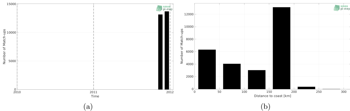
Figure 1: Number of match-ups between TSG (SAMOS) and CCI SSS L4 Merged-OI v3.2 - 30-day running (ESA) SSS as a function of time (a) and as function of the distance to coast (b) over the Mediterranean Sea Pi-MEP region and for the full satellite product period.
