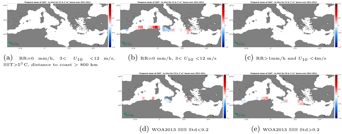
Figure 12: Temporal mean gridded over spatial boxes of size 1^{\circ}\times 1^{\circ} of \Delta\text{SSS} (CCI SSS L4 Merged-OI v3.2 - 30-day running (ESA) - TSG (SAMOS)) for 5 different subdatasets corresponding to:RR=0 mm/h, 3 < U_{10} < 12 m/s, SST >5^{\circ}\text{C} , distance to coast > 800 km (a), RR=0 mm/h, 3 < U_{10} < 12 m/s (b), RR >1 mm/h and U_{10} < 4 m/s (c), WOA2013 SSS Std <0.2 (d), WOA2013 SSS Std >0.2 (e).
