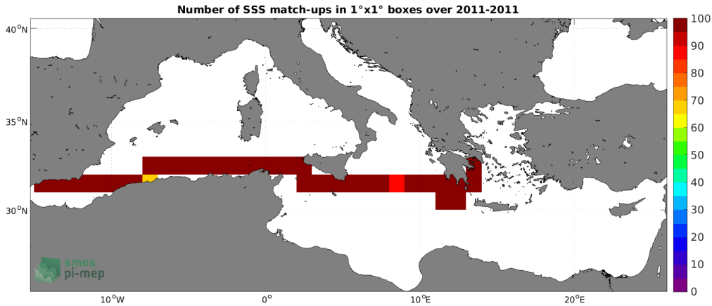
Figure 4: Number of SSS match-ups between TSG (SAMOS) SSS and the CCI SSS L4 Merged-OI v3.2 - 30-day running (ESA) SSS product for the Mediterranean Sea Pi-MEP region over 1^\circ \times 1^\circ boxes and for the full satellite product period.
