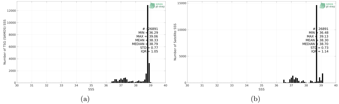
Figure 2: Histograms of SSS from TSG (SAMOS) (a) and CCI SSS L4 Merged-OI v3.2 - 30-day running (ESA) (b) considering all match-up pairs per bins of 0.1 over the Mediterranean Sea Pi-MEP region and for the full satellite product period.
