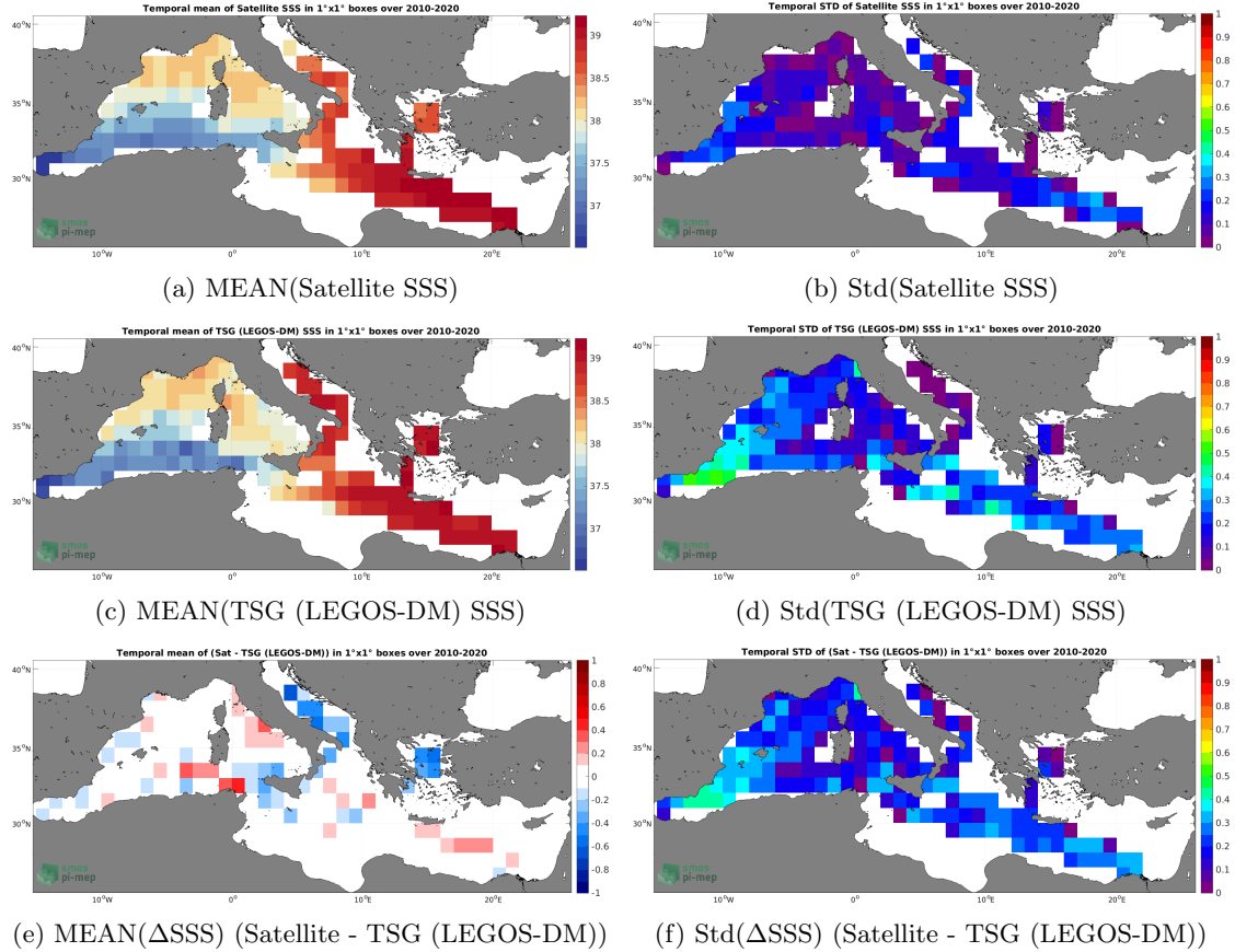
Figure 6: Temporal mean (left) and Std (right) of SSS from CCI SSS L4 Merged-OI v3.2 - 30-day running (ESA) (top), TSG (LEGOS-DM) ( in situ ) (middle), and of \Delta\text{SSS} (Satellite - TSG (LEGOS-DM)). Only match-up pairs are used to generate these maps.
