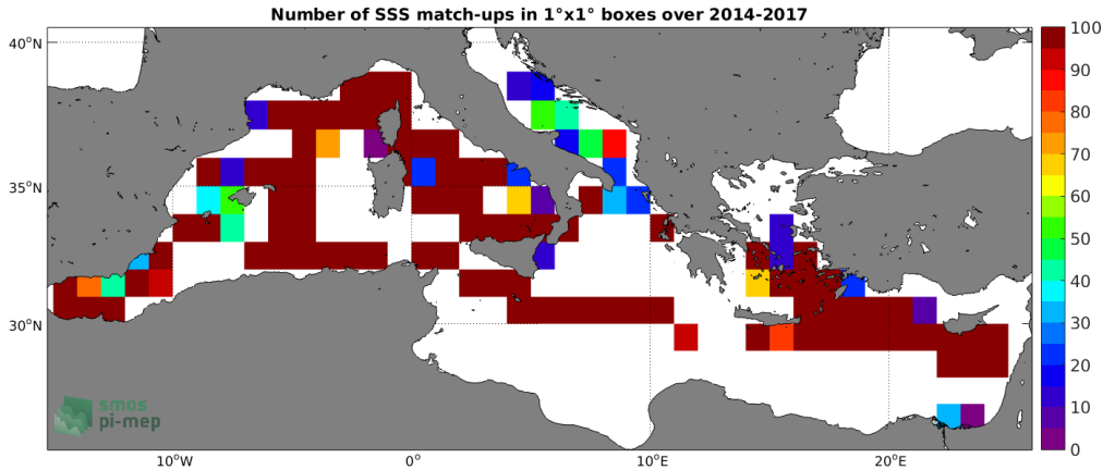
Figure 4: Number of SSS match-ups between TSG (GOSUD-Sailing-ship) SSS and the CCI SSS L4 Merged-OI v3.2 - 30-day running (ESA) SSS product for the Mediterranean Sea Pi-MEP region over 1^\circ \times 1^\circ boxes and for the full satellite product period.
