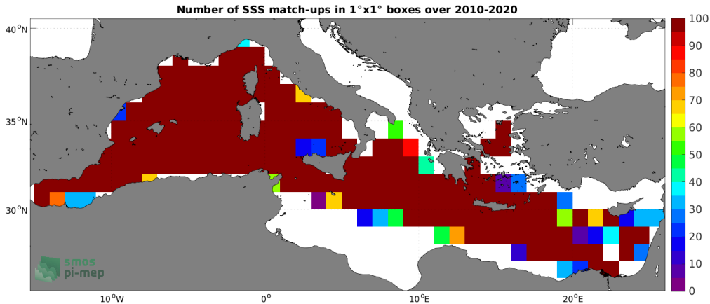
Figure 4: Number of SSS match-ups between TSG (GOSUD-Research-vessel) SSS and the CCI SSS L4 Merged-OI v3.2 - 30-day running (ESA) SSS product for the Mediterranean Sea Pi-MEP region over 1^\circ \times 1^\circ boxes and for the full satellite product period.
