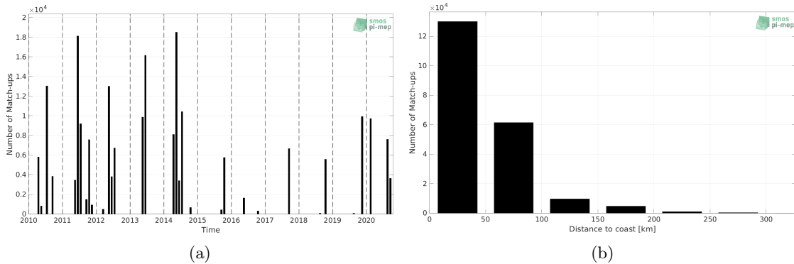
Figure 1: Number of match-ups between TSG (CSIC-UTM) and CCI SSS L4 Merged-OI v3.2 - 30-day running (ESA) SSS as a function of time (a) and as function of the distance to coast (b) over the Mediterranean Sea Pi-MEP region and for the full satellite product period.
