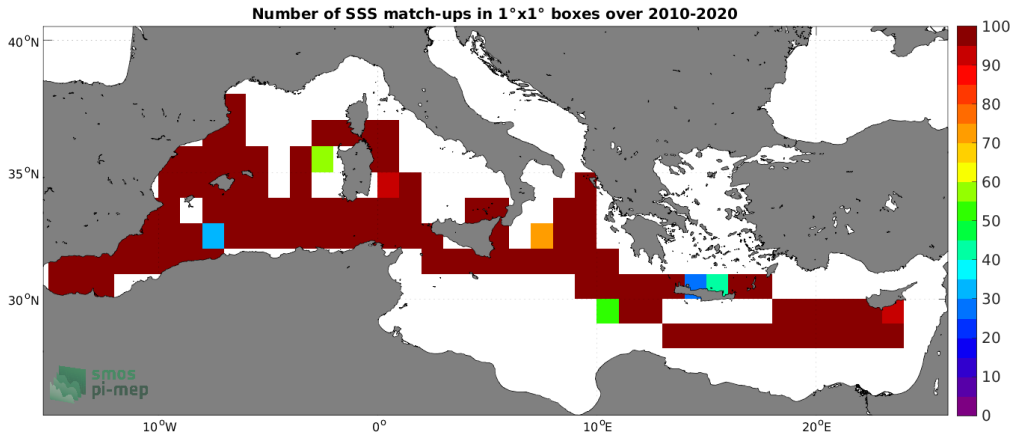
Figure 4: Number of SSS match-ups between TSG (CSIC-UTM) SSS and the CCI SSS L4 Merged-OI v3.2 - 30-day running (ESA) SSS product for the Mediterranean Sea Pi-MEP region over 1^\circ \times 1^\circ boxes and for the full satellite product period.
