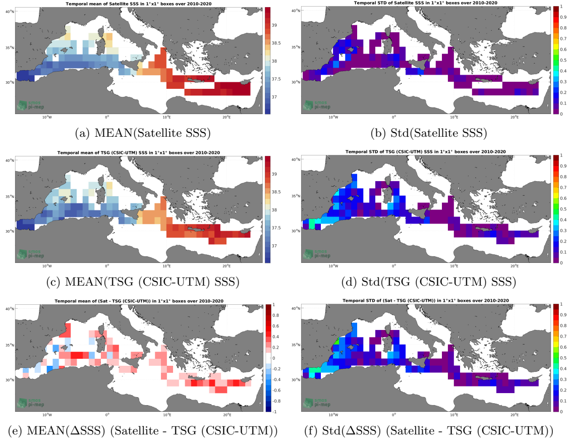
Figure 6: Temporal mean (left) and Std (right) of SSS from CCI SSS L4 Merged-OI v3.2 - 30-day running (ESA) (top), TSG (CSIC-UTM) (middle), and of \Delta\text{SSS} (Satellite - TSG (CSIC-UTM)). Only match-up pairs are used to generate these maps.
