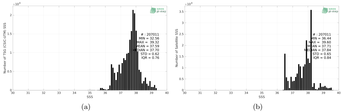
Figure 2: Histograms of SSS from TSG (CSIC-UTM) (a) and CCI SSS L4 Merged-OI v3.2 - 30-day running (ESA) (b) considering all match-up pairs per bins of 0.1 over the Mediterranean Sea Pi-MEP region and for the full satellite product period.
