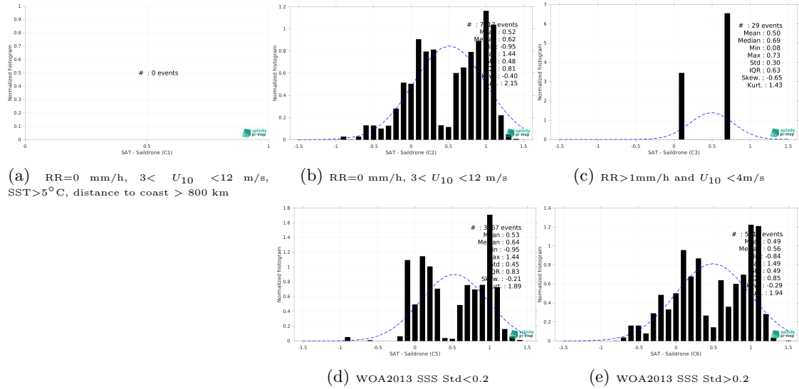
Figure 13: Normalized histogram of \Delta\text{SSS} (CCI SSS L4 Merged-OI v3.2 - 30-day running (ESA) - Saildrone) for 5 different subdatasets corresponding to: RR=0 mm/h, 3 < U_{10} < 12 m/s, SST >5^{\circ}\text{C} , distance to coast > 800 km (a), RR=0 mm/h, 3 < U_{10} < 12 m/s (b), RR>1\text{mm/h} and U_{10} < 4\text{m/s} (c), WOA2013 SSS Std <0.2 (d), WOA2013 SSS Std >0.2 (e).
