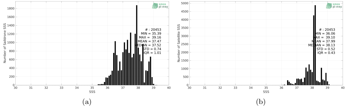
Figure 2: Histograms of SSS from Saildrone (a) and CCI SSS L4 Merged-OI v3.2 - 30-day running (ESA) (b) considering all match-up pairs per bins of 0.1 over the Mediterranean Sea Pi-MEP region and for the full satellite product period.
