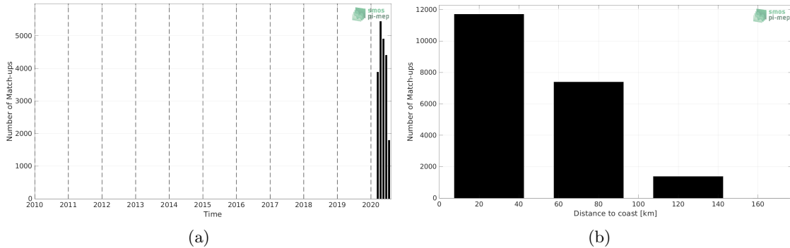
Figure 1: Number of match-ups between Saildrone and CCI SSS L4 Merged-OI v3.2 - 30-day running (ESA) SSS as a function of time (a) and as function of the distance to coast (b) over the Mediterranean Sea Pi-MEP region and for the full satellite product period.
