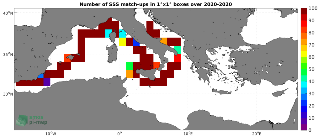
Figure 4: Number of SSS match-ups between Saildrone SSS and the CCI SSS L4 Merged-OI v3.2 - 30-day running (ESA) SSS product for the Mediterranean Sea Pi-MEP region over 1^\circ \times 1^\circ boxes and for the full satellite product period.
