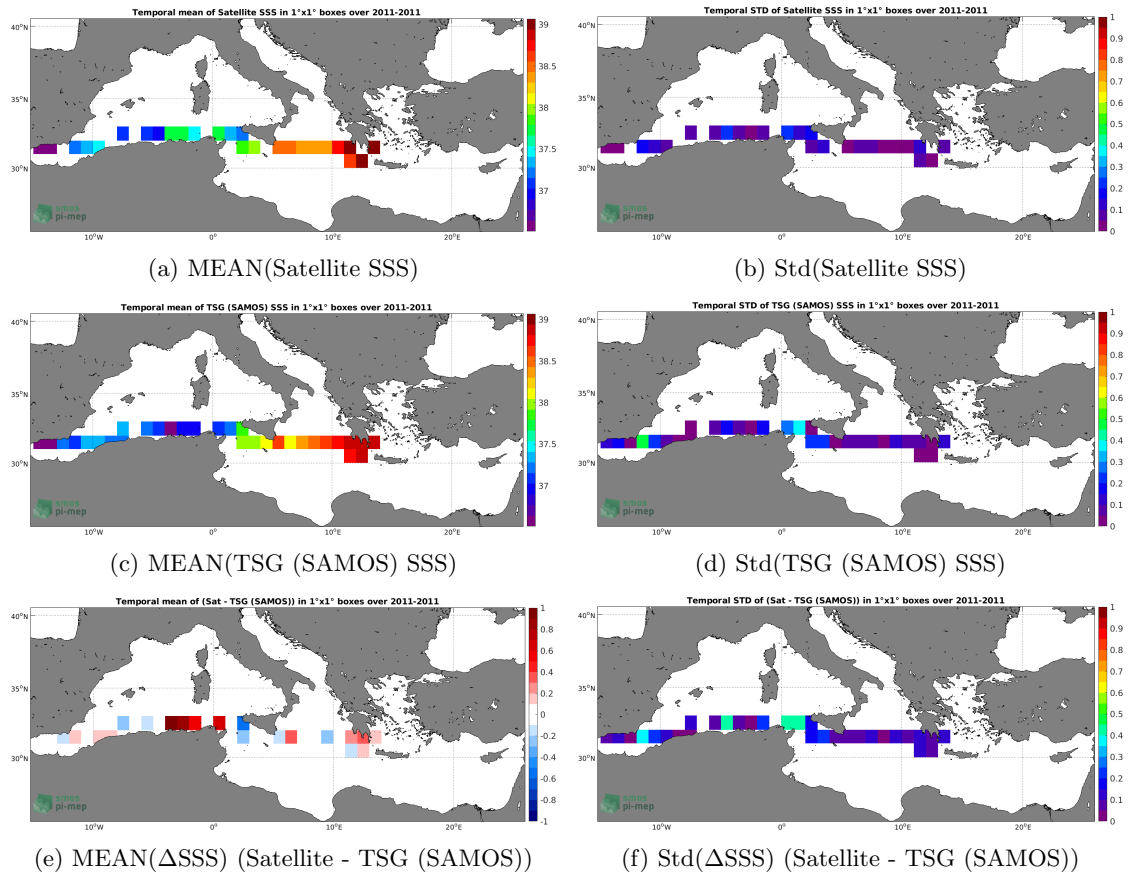
Figure 6: Temporal mean (left) and Std (right) of SSS from CCI SSS L4 Merged-OI v2.31 - 7-day running (ESA) (top), TSG (SAMOS) (middle), and of \Delta SSS (Satellite - TSG (SAMOS)). Only match-up pairs are used to generate these maps.
