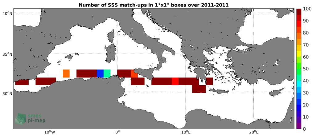
Figure 4: Number of SSS match-ups between TSG (SAMOS) SSS and the CCI SSS L4 Merged-OI v2.31 - 7-day running (ESA) SSS product for the Mediterranean Sea Pi-MEP region over 1^\circ \times 1^\circ boxes and for the full satellite product period.
