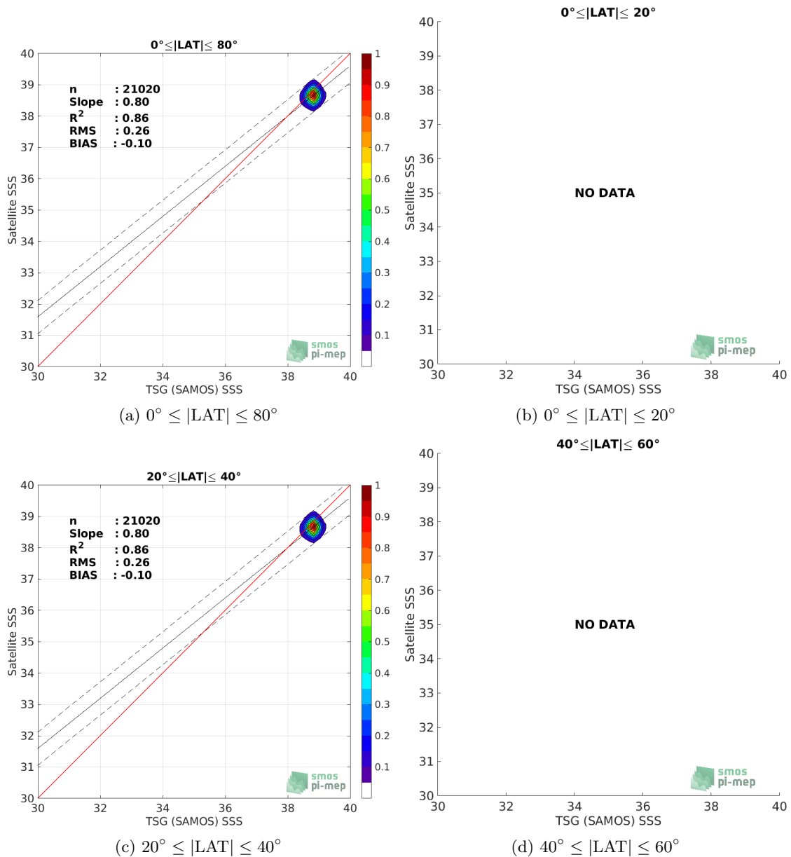
Figure 9: Contour maps of the concentration of CCI SSS L4 Merged-OI v2.31 - 7-day running (ESA) SSS (y-axis) versus TSG (SAMOS) SSS (x-axis) at match-up pairs for different latitude bands. For each plot, the red line shows x=y . The black thin and dashed lines indicate a linear fit through the data cloud and the \pm 95\% confidence levels, respectively. The number match-up pairs n , the slope and R^2 coefficient of the linear fit, the root mean square (RMS) and the mean bias between satellite and in situ data are indicated for each latitude band in each plots.
