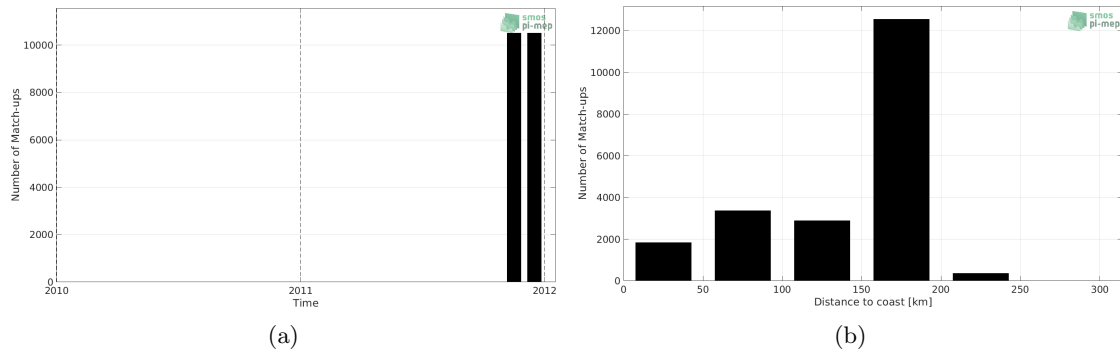
Figure 1: Number of match-ups between TSG (SAMOS) and CCI SSS L4 Merged-OI v2.31 - 7-day running (ESA) SSS as a function of time (a) and as function of the distance to coast (b) over the Mediterranean Sea Pi-MEP region and for the full satellite product period.
