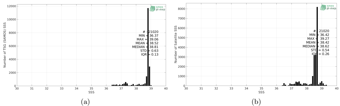
Figure 2: Histograms of SSS from TSG (SAMOS) (a) and CCI SSS L4 Merged-OI v2.31 - 7-day running (ESA) (b) considering all match-up pairs per bins of 0.1 over the Mediterranean Sea Pi-MEP region and for the full satellite product period.
