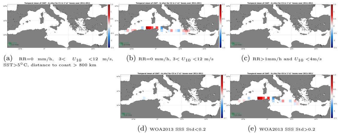
Figure 12: Temporal mean gridded over spatial boxes of size 1^{\circ}\times 1^{\circ} of \Delta\text{SSS} (CCI SSS L4 Merged-OI v2.31 - 7-day running (ESA) - TSG (SAMOS)) for 5 different subdatasets corresponding to: RR=0 mm/h, 3 < U_{10} < 12 m/s, SST > 5^{\circ}\text{C} , distance to coast > 800 km (a), RR=0 mm/h, 3 < U_{10} < 12 m/s (b), RR > 1 mm/h and U_{10} < 4 m/s (c), WOA2013 SSS Std < 0.2 (d), WOA2013 SSS Std > 0.2 (e).
