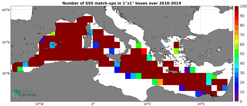
Figure 4: Number of SSS match-ups between TSG (GOSUD-Research-vessel) SSS and the CCI SSS L4 Merged-OI v2.31 - 7-day running (ESA) SSS product for the Mediterranean Sea Pi-MEP region over 1^\circ \times 1^\circ boxes and for the full satellite product period.
