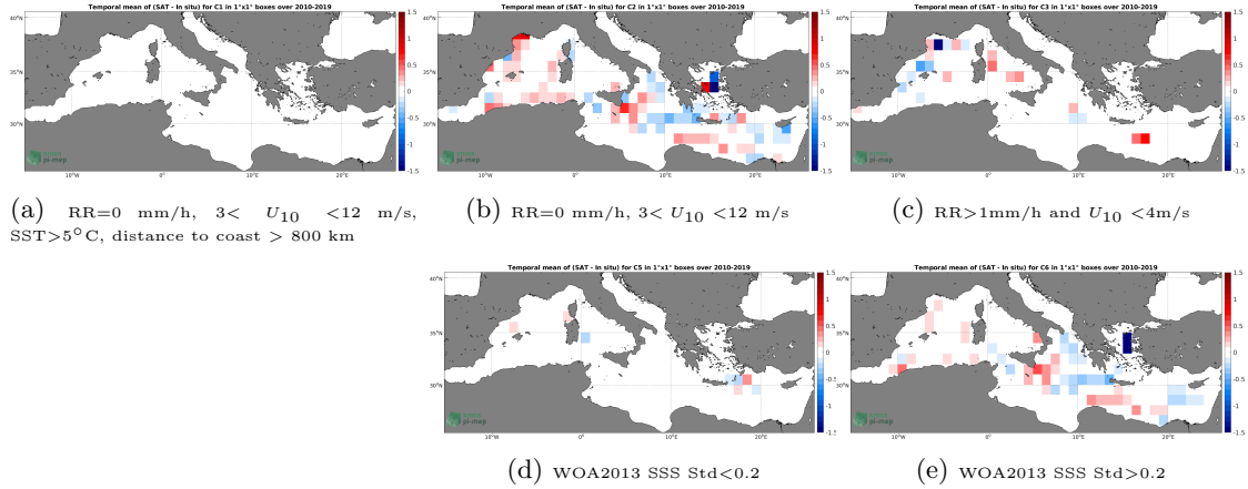
Figure 12: Temporal mean gridded over spatial boxes of size 1^{\circ}\times 1^{\circ} of \Delta SSS (CCI SSS L4 Merged-OI v2.31 - 7-day running (ESA) - TSG (GOSUD-Research-vessel)) for 5 different subdatasets corresponding to: RR=0 mm/h, 3 < U_{10} < 12 m/s, SST > 5^{\circ}\text{C} , distance to coast > 800 km (a), RR=0 mm/h, 3 < U_{10} < 12 m/s (b), RR > 1 mm/h and U_{10} < 4 m/s (c), WOA2013 SSS Std < 0.2 (d), WOA2013 SSS Std > 0.2 (e).
