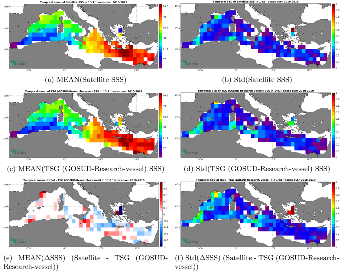
Figure 6: Temporal mean (left) and Std (right) of SSS from CCI SSS L4 Merged-OI v2.31 - 7-day running (ESA) (top), TSG (GOSUD-Research-vessel) ( in situ ) dataset (middle), and of \Delta\text{SSS} (Satellite - TSG (GOSUD-Research-vessel)). Only match-up pairs are used to generate these maps.
