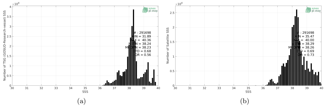
Figure 2: Histograms of SSS from TSG (GOSUD-Research-vessel) (a) and CCI SSS L4 Merged-OI v2.31 - 7-day running (ESA) (b) considering all match-up pairs per bins of 0.1 over the Mediterranean Sea Pi-MEP region and for the full satellite product period.
