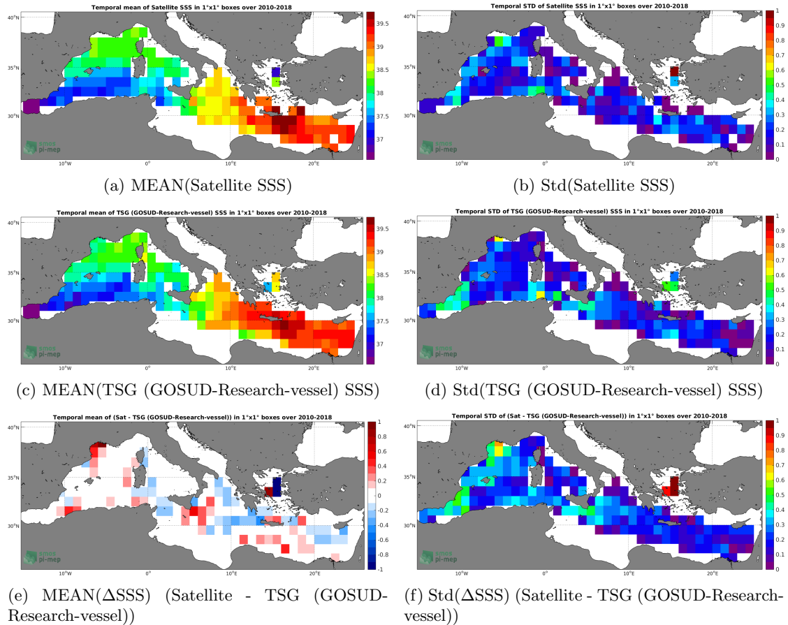
Figure 6: Temporal mean (left) and Std (right) of SSS from CCI SSS L4 Merged-OI v2.31 - 7-day running (ESA) (top), TSG (GOSUD-Research-vessel) (middle), and of \Delta SSS (Satellite - TSG (GOSUD-Research-vessel)). Only match-up pairs are used to generate these maps.
