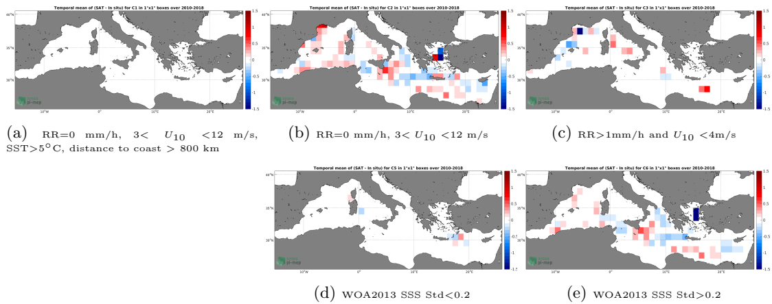
Figure 12: Temporal mean gridded over spatial boxes of size 1^\circ \times 1^\circ of \Delta SSS (CCI SSS L4 Merged-OI v2.31 - 7-day running (ESA) - TSG (GOSUD-Research-vessel)) for 5 different subdatasets corresponding to:RR=0 mm/h, 3 < U_{10} < 12 m/s, SST >5^\circ\text{C} , distance to coast > 800 km (a), RR=0 mm/h, 3 < U_{10} < 12 m/s (b), RR >1 mm/h and U_{10} < 4 m/s (c), WOA2013 SSS Std <0.2 (d), WOA2013 SSS Std >0.2 (e).
