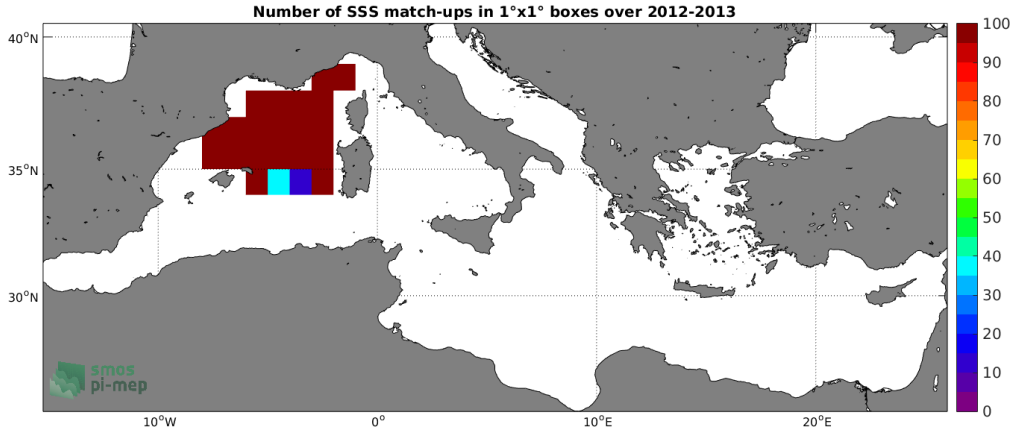
Figure 3: Number of SSS match-ups between Surface drifters SSS and the CCI SSS L4 Merged-OI v2.31 - 7-day running (ESA) SSS product for the Mediterranean Sea Pi-MEP region over 1^\circ \times 1^\circ boxes and for the full satellite product period.
