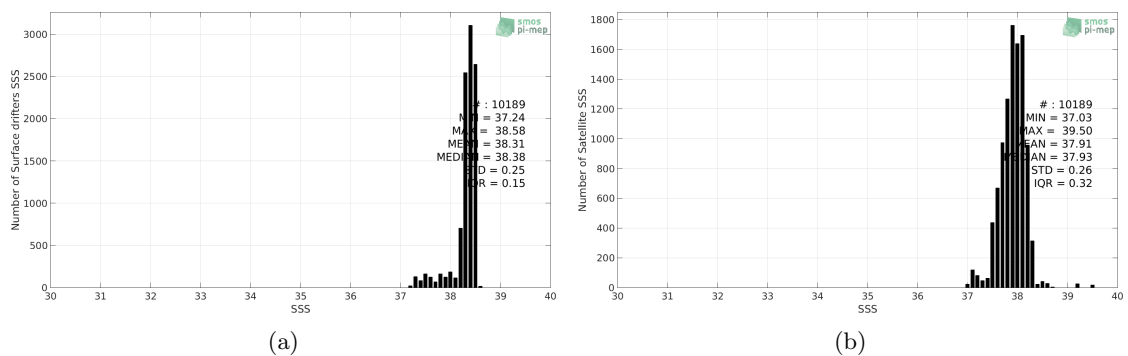
Figure 2: Histograms of SSS from Surface drifters (a) and CCI SSS L4 Merged-OI v2.31 - 7-day running (ESA) (b) considering all match-up pairs per bins of 0.1 over the Mediterranean Sea Pi-MEP region and for the full satellite product period.
