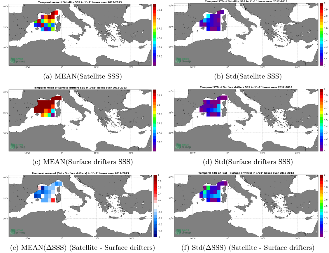
Figure 5: Temporal mean (left) and Std (right) of SSS from CCI SSS L4 Merged-OI v2.31 - 7-day running (ESA) (top), Surface drifters (middle), and of \Delta SSS (Satellite - Surface drifters). Only match-up pairs are used to generate these maps.
