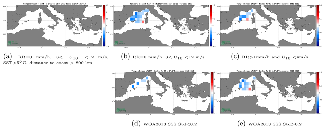
Figure 11: Temporal mean gridded over spatial boxes of size 1^\circ \times 1^\circ of \Delta SSS (CCI SSS L4 Merged-OI v2.31 - 7-day running (ESA) - Surface drifters) for 5 different subdatasets corresponding to:RR=0 mm/h, 3 < U_{10} < 12 m/s, SST >5^\circ C, distance to coast > 800 km (a), RR=0 mm/h, 3 < U_{10} < 12 m/s (b), RR >1 mm/h and U_{10} < 4 m/s (c), WOA2013 SSS Std <0.2 (d), WOA2013 SSS Std >0.2 (e).
