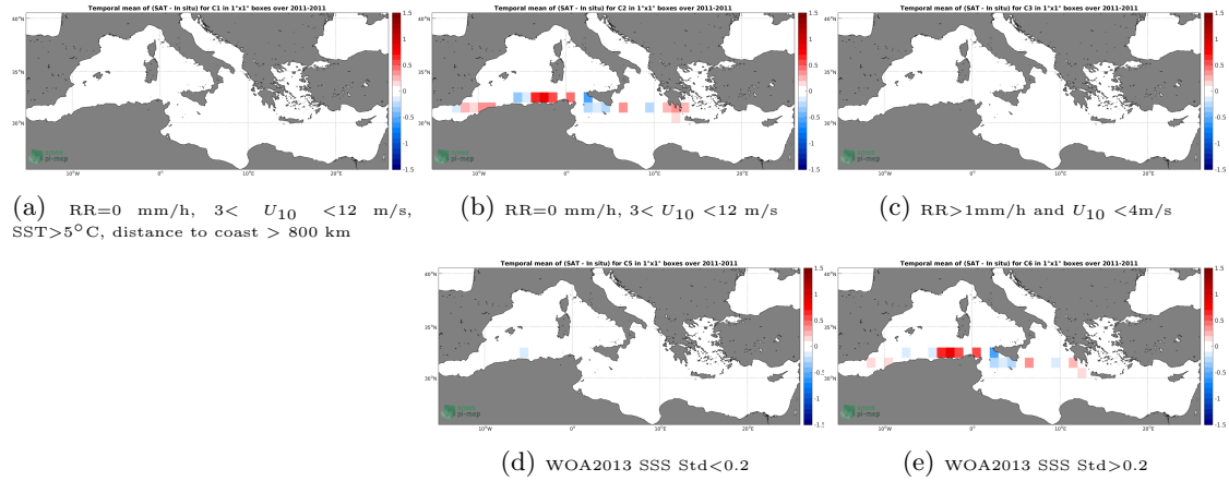
Figure 12: Temporal mean gridded over spatial boxes of size 1^{\circ}\times 1^{\circ} of \Delta\text{SSS} (CCI L4 Merged-OI v2.31 - 30-day running (ESA) - TSG (SAMOS)) for 5 different subdatasets corresponding to:RR=0 mm/h, 3 < U_{10} < 12 m/s, SST >5^{\circ}\text{C} , distance to coast > 800 km (a), RR=0 mm/h, 3 < U_{10} < 12 m/s (b), RR >1 mm/h and U_{10} < 4 m/s (c), WOA2013 SSS Std <0.2 (d), WOA2013 SSS Std >0.2 (e).
