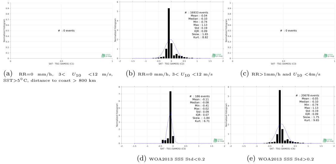
Figure 13: Normalized histogram of \Delta\text{SSS} (CCI L4 Merged-OI v2.31 - 30-day running (ESA) - TSG (SAMOS)) for 5 different subdatasets corresponding to: RR=0 mm/h, 3 < U_{10} < 12 m/s, SST > 5^{\circ}\text{C} , distance to coast > 800 km (a), RR=0 mm/h, 3 < U_{10} < 12 m/s (b), RR > 1\text{mm/h} and U_{10} < 4\text{m/s} (c), WOA2013 SSS Std < 0.2 (d), WOA2013 SSS Std > 0.2 (e).
