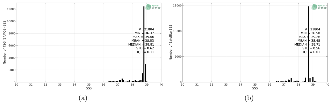
Figure 2: Histograms of SSS from TSG (SAMOS) (a) and CCI L4 Merged-OI v2.31 - 30-day running (ESA) (b) considering all match-up pairs per bins of 0.1 over the Mediterranean Sea Pi-MEP region and for the full satellite product period.
