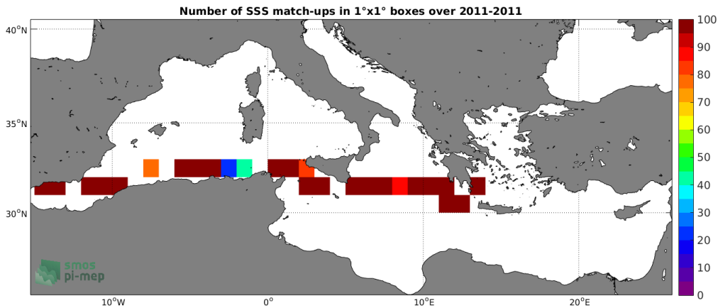
Figure 4: Number of SSS match-ups between TSG (SAMOS) SSS and the CCI L4 Merged-OI v2.31 - 30-day running (ESA) SSS product for the Mediterranean Sea Pi-MEP region over 1^\circ \times 1^\circ boxes and for the full satellite product period.
