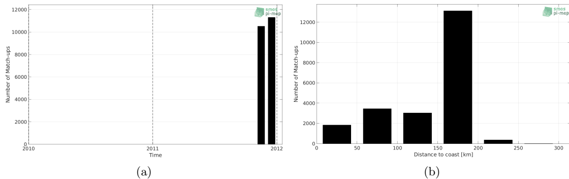
Figure 1: Number of match-ups between TSG (SAMOS) and CCI L4 Merged-OI v2.31 - 30-day running (ESA) SSS as a function of time (a) and as function of the distance to coast (b) over the Mediterranean Sea Pi-MEP region and for the full satellite product period.
