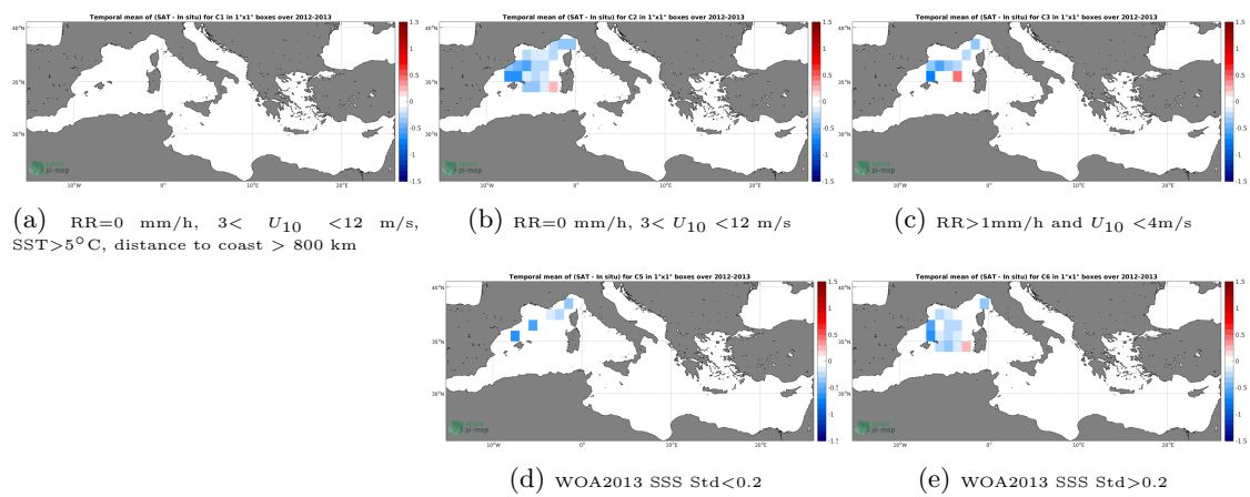
Figure 11: Temporal mean gridded over spatial boxes of size 1^\circ \times 1^\circ of \Delta SSS (CCI L4 Merged-OI v2.31 - 30-day running (ESA) - Surface drifters) for 5 different subdatasets corresponding to:RR=0 mm/h, 3 < U_{10} < 12 m/s, SST >5^\circ C, distance to coast > 800 km (a), RR=0 mm/h, 3 < U_{10} < 12 m/s (b), RR >1 mm/h and U_{10} < 4 m/s (c), WOA2013 SSS Std <0.2 (d), WOA2013 SSS Std >0.2 (e).
