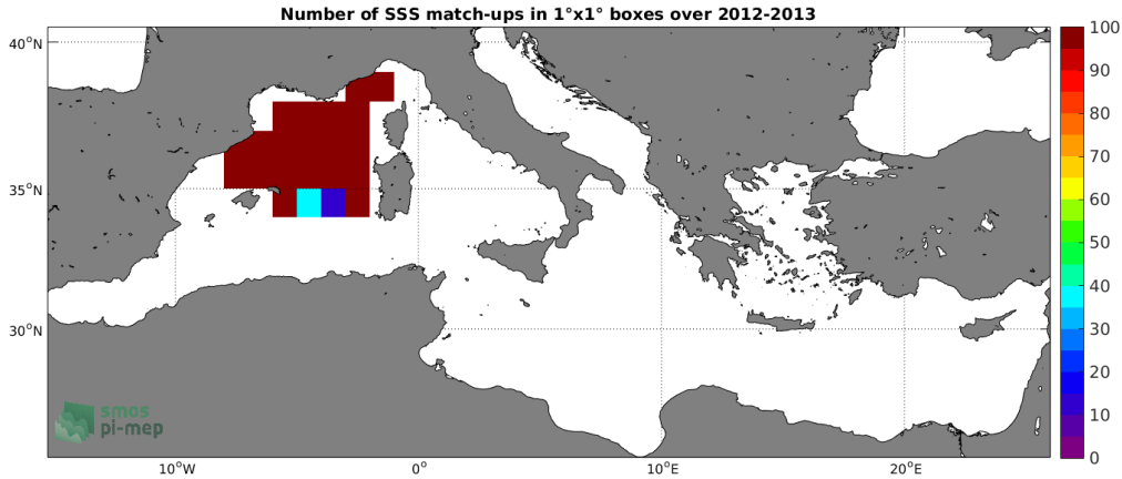
Figure 3: Number of SSS match-ups between Surface drifters SSS and the CCI L4 Merged-OI v2.31 - 30-day running (ESA) SSS product for the Mediterranean Sea Pi-MEP region over 1^\circ \times 1^\circ boxes and for the full satellite product period.
