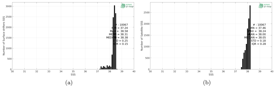
Figure 2: Histograms of SSS from Surface drifters (a) and CCI L4 Merged-OI v2.31 - 30-day running (ESA) (b) considering all match-up pairs per bins of 0.1 over the Mediterranean Sea Pi-MEP region and for the full satellite product period.
