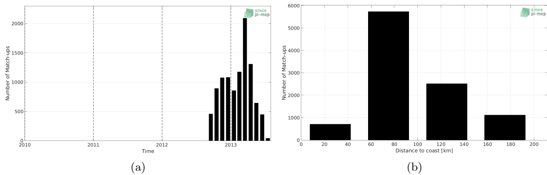
Figure 1: Number of match-ups between Surface drifters and CCI L4 Merged-OI v2.31 - 30-day running (ESA) SSS as a function of time (a) and as function of the distance to coast (b) over the Mediterranean Sea Pi-MEP region and for the full satellite product period.
