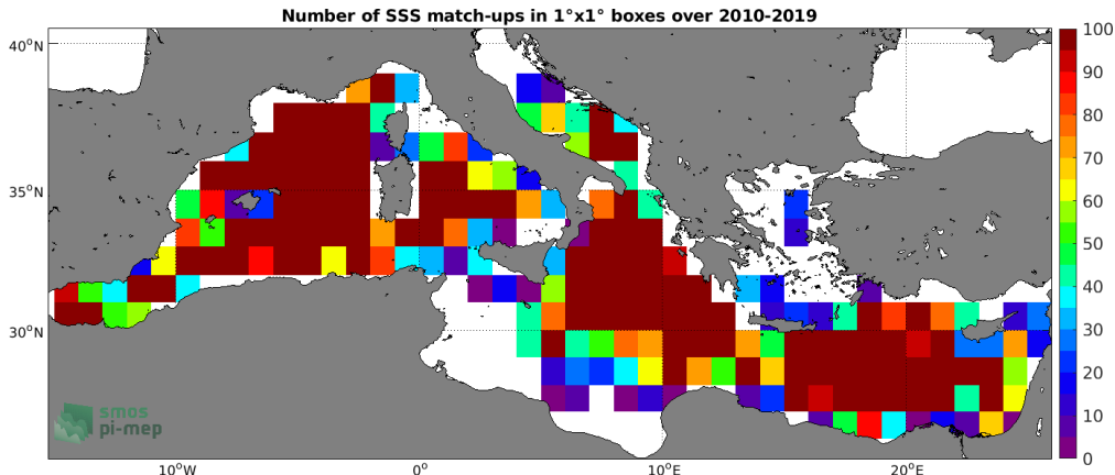
Figure 4: Number of SSS match-ups between Argo SSS and the CCI SSS L4 Merged-OI v2.31 - 30-day running (ESA) SSS product for the Mediterranean Sea Pi-MEP region over 1^\circ \times 1^\circ boxes and for the full satellite product period.
