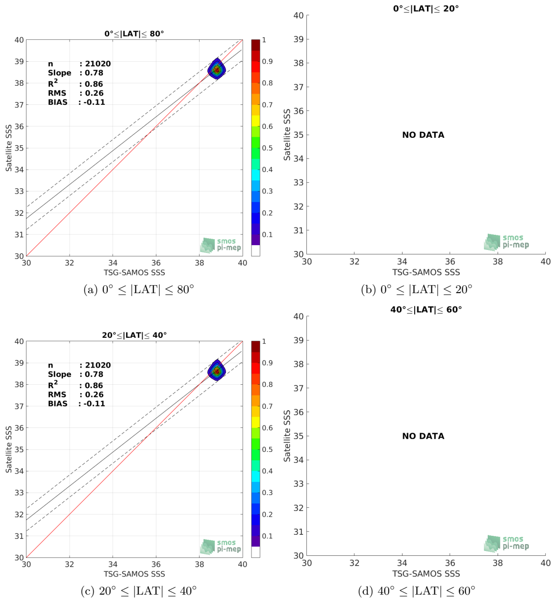
Figure 9: Contour maps of the concentration of CCI-L4-ESA-MERGED-OI-V1.8-7DAY-RUNNING SSS (y-axis) versus TSG-SAMOS SSS (x-axis) at match-up pairs for different latitude bands. For each plot, the red line shows x=y . The black thin and dashed lines indicate a linear fit through the data cloud and the \pm 95\% confidence levels, respectively. The number match-up pairs n , the slope and R^2 coefficient of the linear fit, the root mean square (RMS) and the mean bias between satellite and in situ data are indicated for each latitude band in each plots.
