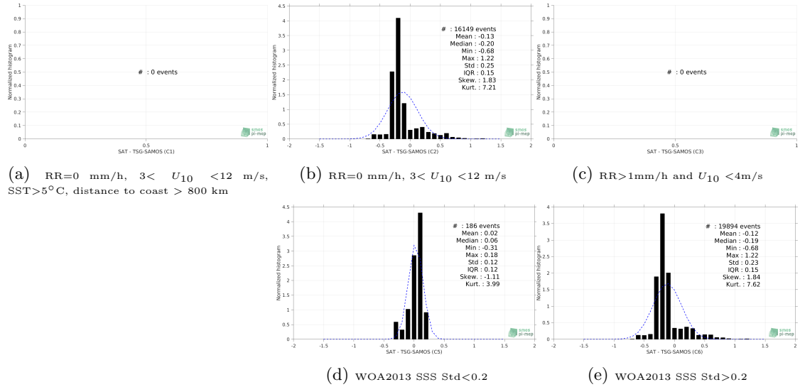
Figure 13: Normalized histogram of \Delta SSS (CCI-L4-ESA-MERGED-OI-V1.8-7DAY-RUNNING - TSG-SAMOS) for 5 different subdatasets corresponding to: RR=0 mm/h, 3 < U_{10} < 12 m/s, SST > 5°C, distance to coast > 800 km (a), RR=0 mm/h, 3 < U_{10} < 12 m/s (b), RR > 1mm/h and U_{10} < 4 m/s (c), WOA2013 SSS Std < 0.2 (d), WOA2013 SSS Std > 0.2 (e).
