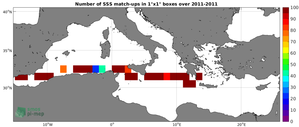
Figure 4: Number of SSS match-ups between TSG-SAMOS SSS and the CCI-L4-ESA-MERGED-OI-V1.8-7DAY-RUNNING SSS product for the Mediterranean Sea Pi-MEP region over 1^\circ \times 1^\circ boxes and for the full satellite product period.
