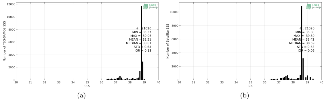
Figure 2: Histograms of SSS from TSG-SAMOS (a) and CCI-L4-ESA-MERGED-OI-V1.8-7DAY-RUNNING (b) considering all match-up pairs per bins of 0.1 over the Mediterranean Sea Pi-MEP region and for the full satellite product period.
