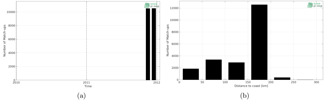
Figure 1: Number of match-ups between TSG-SAMOS and CCI-L4-ESA-MERGED-OI-V1.8-7DAY-RUNNING SSS as a function of time (a) and as function of the distance to coast (b) over the Mediterranean Sea Pi-MEP region and for the full satellite product period.
