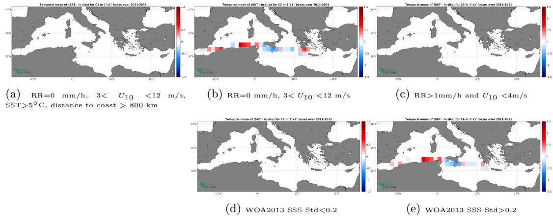
Figure 12: Temporal mean gridded over spatial boxes of size 1^\circ \times 1^\circ of \Delta SSS (CCI-L4-ESAMERGED-OI-V1.8-7DAY-RUNNING - TSG-SAMOS) for 5 different subdatasets corresponding to:RR=0 mm/h, 3 < U_{10} < 12 m/s, SST >5^\circ\text{C} , distance to coast > 800 km (a), RR=0 mm/h, 3 < U_{10} < 12 m/s (b), RR >1 mm/h and U_{10} < 4 m/s (c), WOA2013 SSS Std <0.2 (d), WOA2013 SSS Std >0.2 (e).
